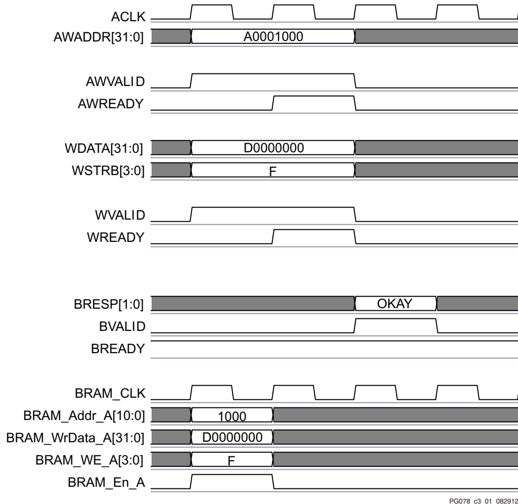
Figure 3-1: AXI4-Lite Write Timing
