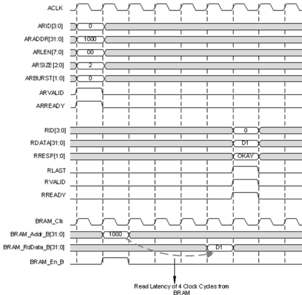
Figure 1-3: Example 1: Single Read, Read Latency = 4
