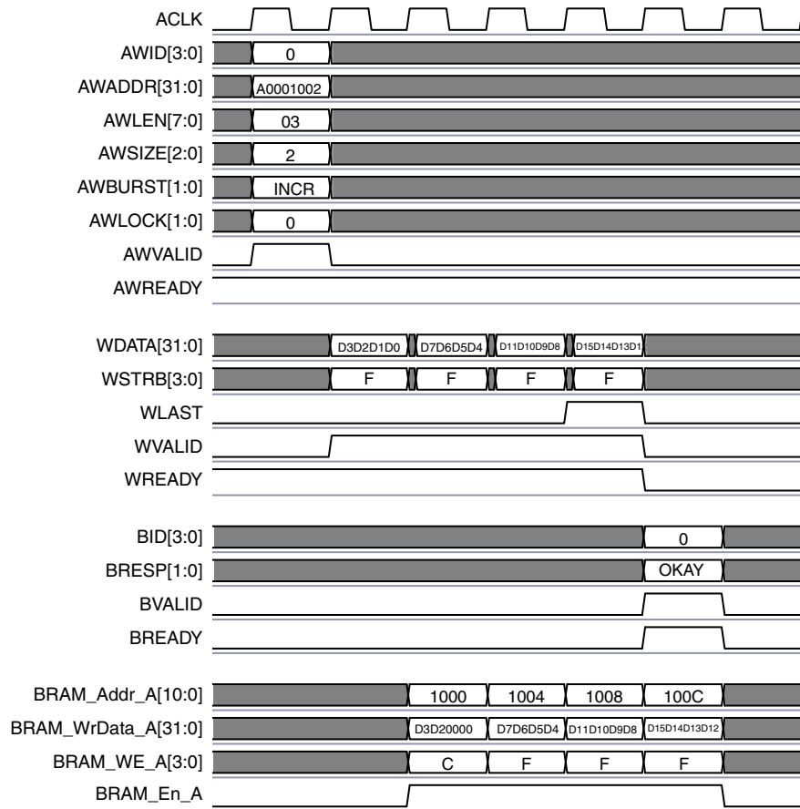
Figure 3-10: AXI Unaligned Burst Write Timing
