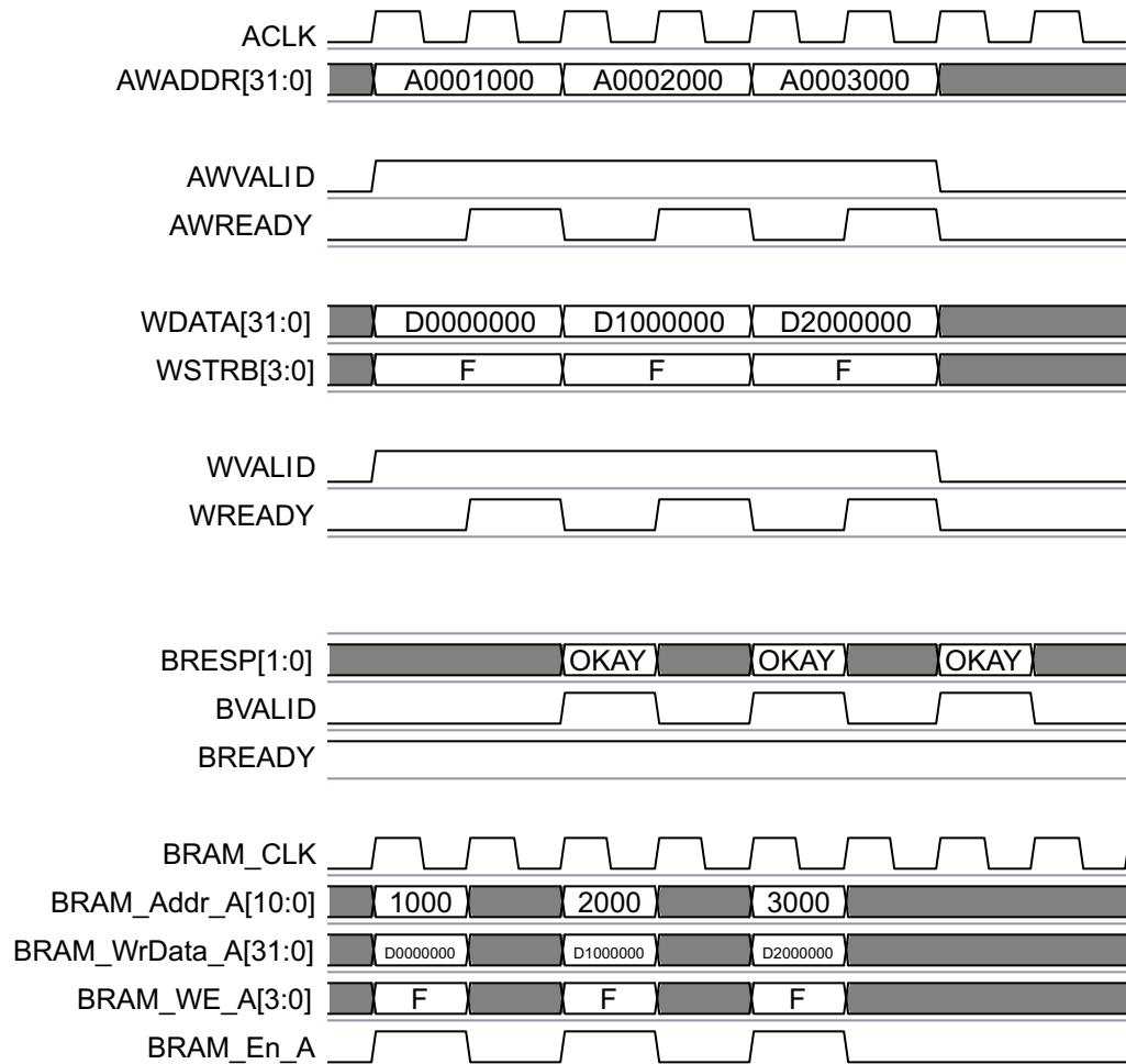
Figure 3-2: Multiple AXI4-Lite Write Transactions
