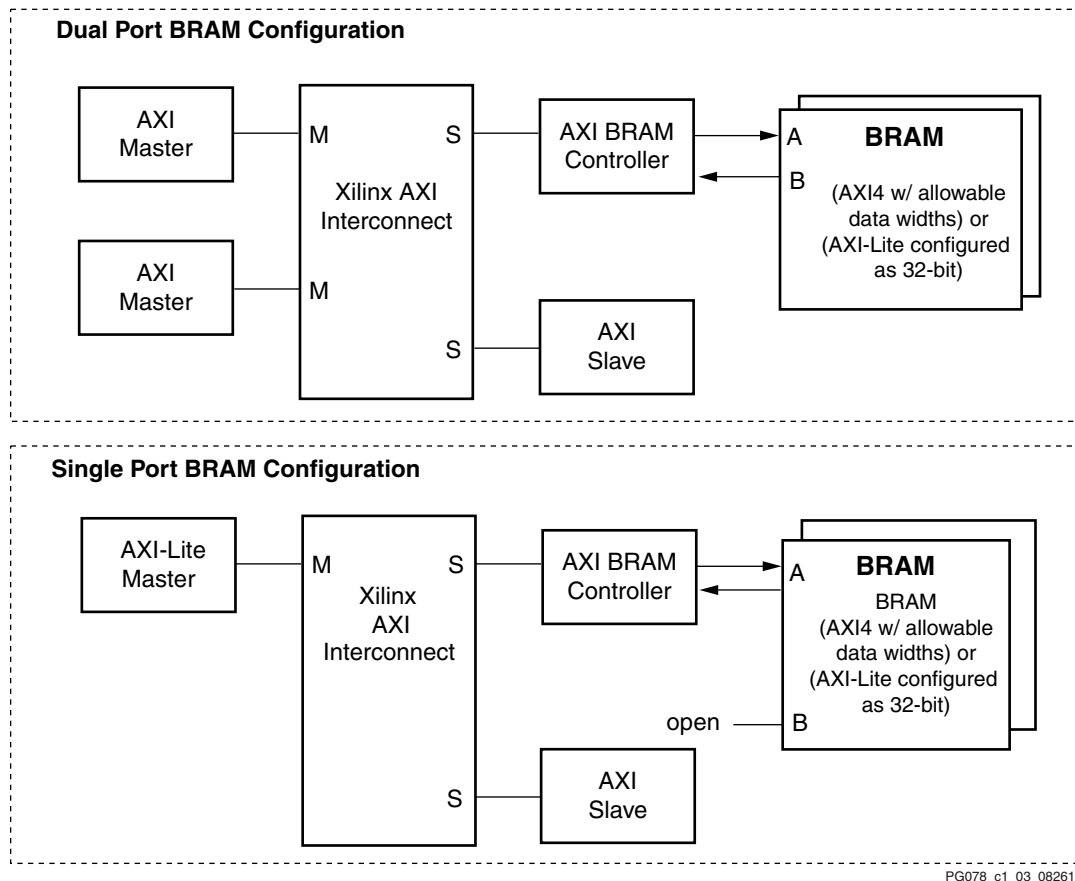
Figure 1-7: AXI System Configuration
