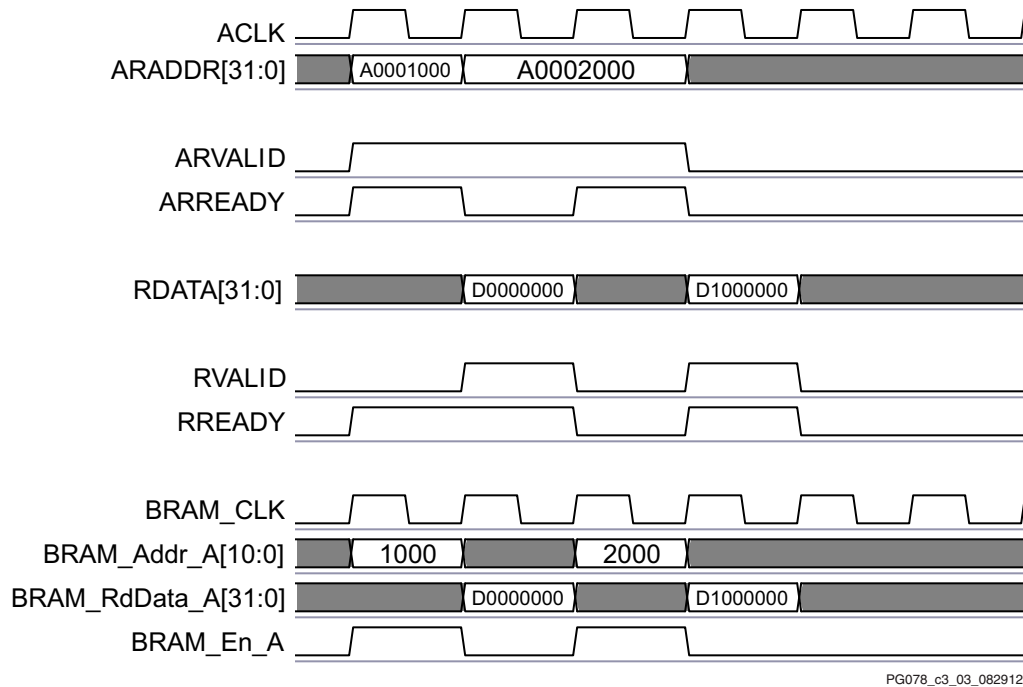
Figure 3-3: AXI4-Lite Read Timing
