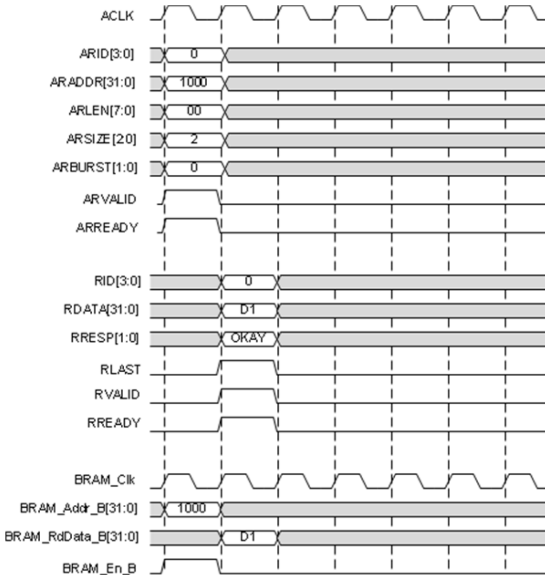
Figure 1-5: Example 1: AXI4 Single Read
