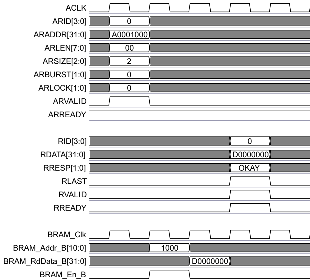
Figure 3-6: AXI Single Read Timing Diagram
