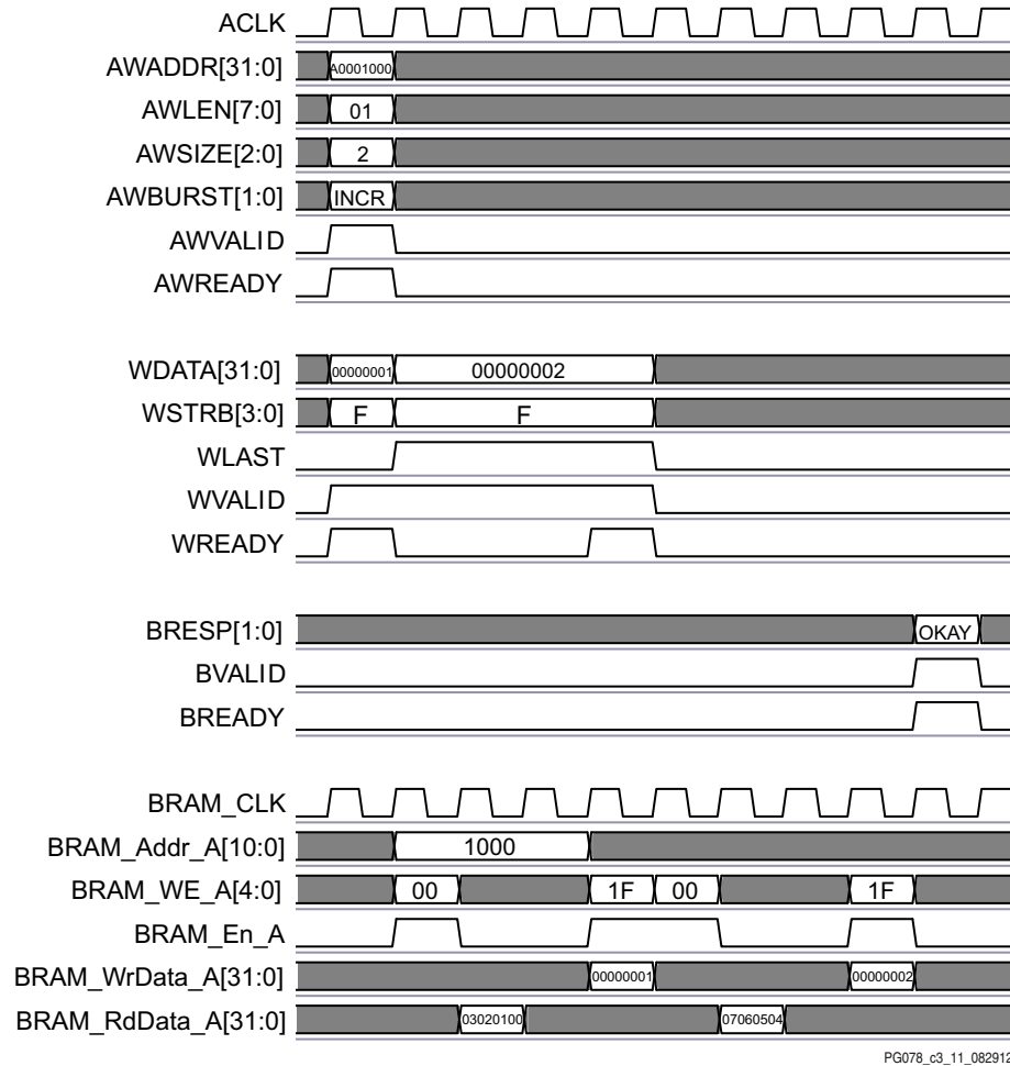
Figure 3-11: AXI Write Burst with ECC
