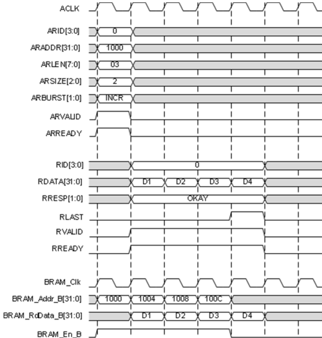
Figure 1-6: Example 2: AXI4 Burst Read
