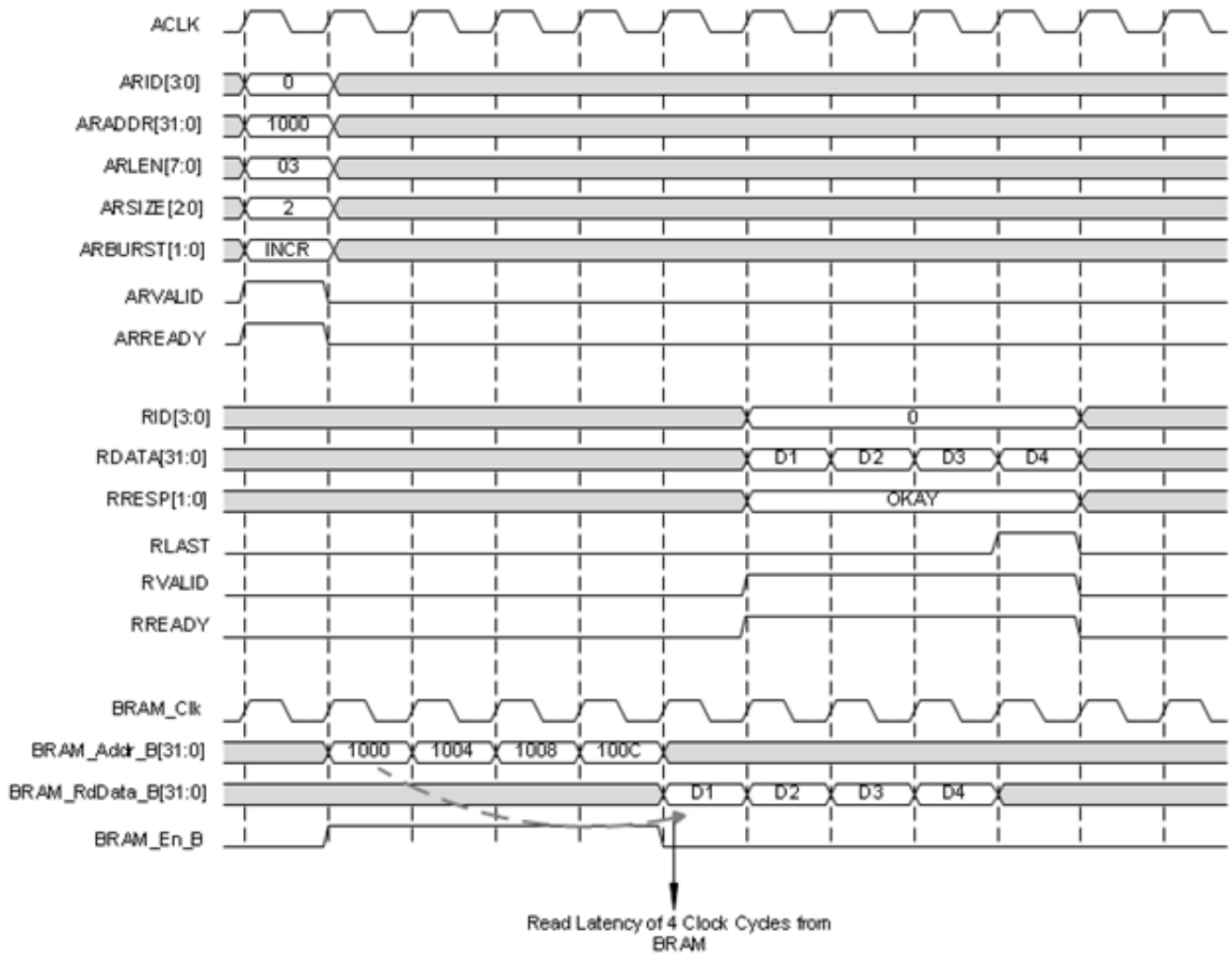
Figure 1-4: Example 2: AXI4 Burst Read, Read Latency = 4
