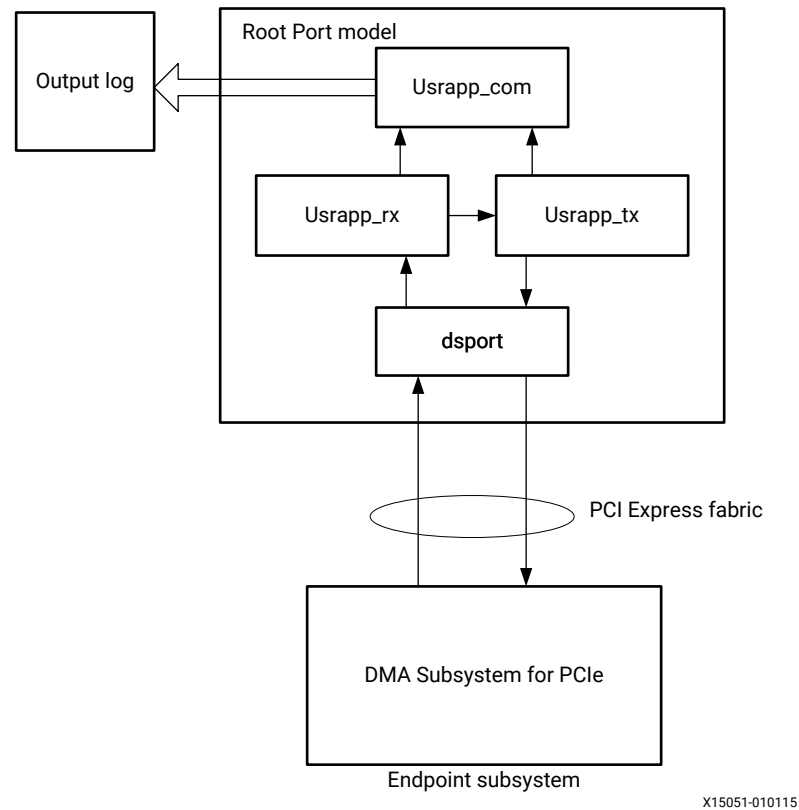
Figure 32: Root Port Module with DMA Subsystem for PCIe
