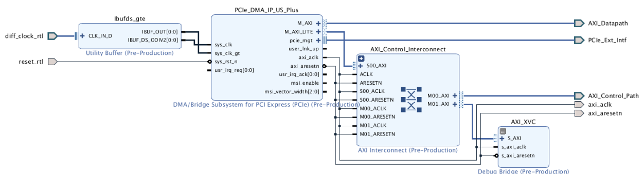
Figure 36: XVC over PCIe with AXI4-Lite Interface
