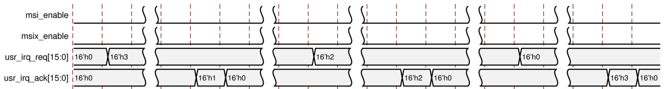
Figure 2: Legacy Interrupts
