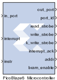
PicoBlaze6 Microcontroller
