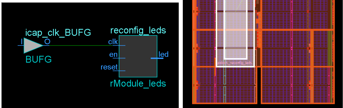
Figure 6-1: Pre-routing Global Clock to Reconfigurable Partition
