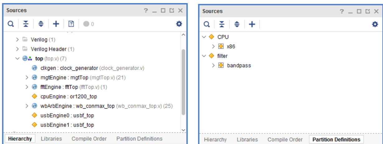
Figure 4-4: Partition Definitions as seen in the Sources Window
