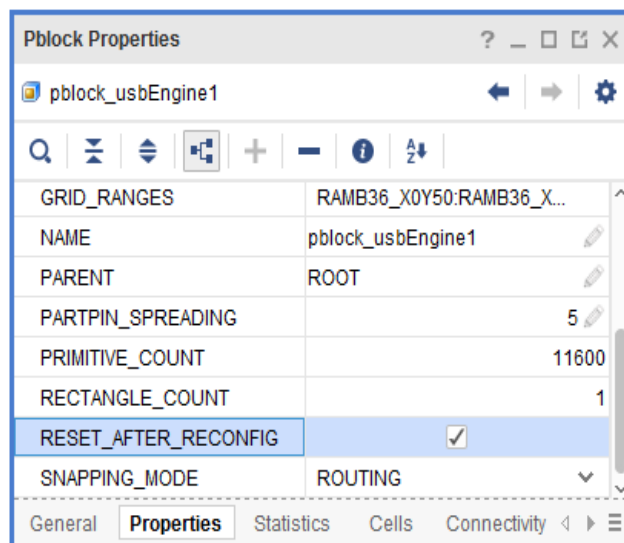
Figure 4-17: Partial Reconfiguration properties on a Pblock (7 series)
