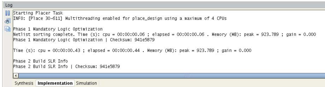
Figure 3-4: Log Window
