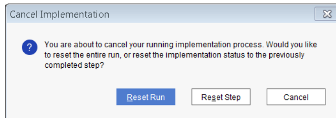
Figure 3-3: Cancel Implementation
