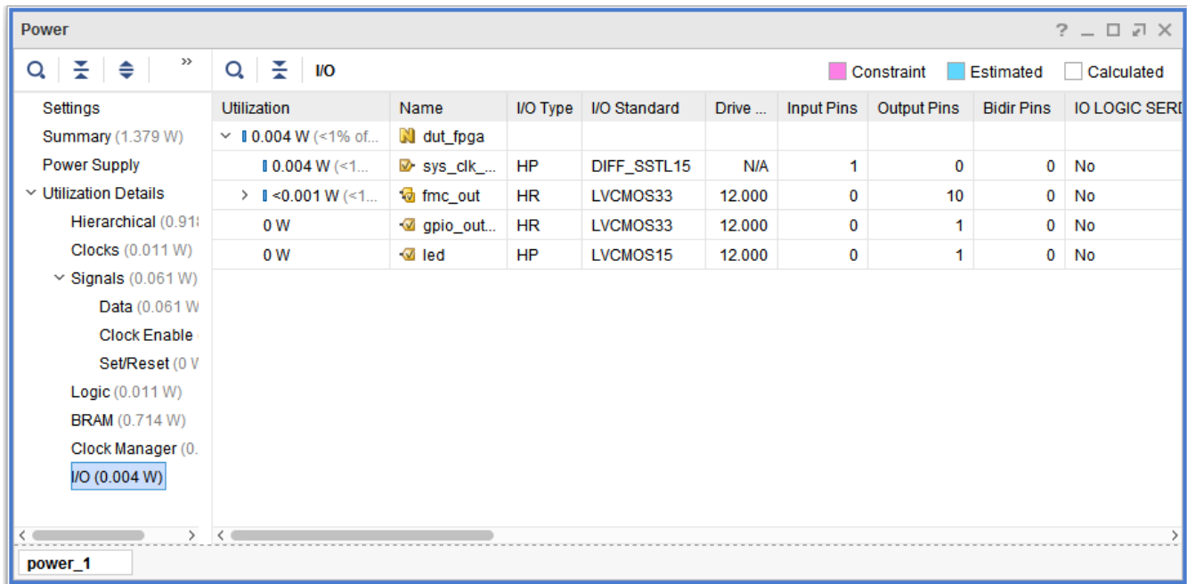
Figure 5-14: I/O View in the Power Report
