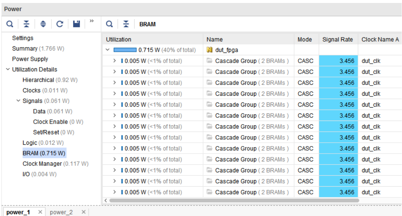
Figure 5-15: Activity Rate for a BRAM
