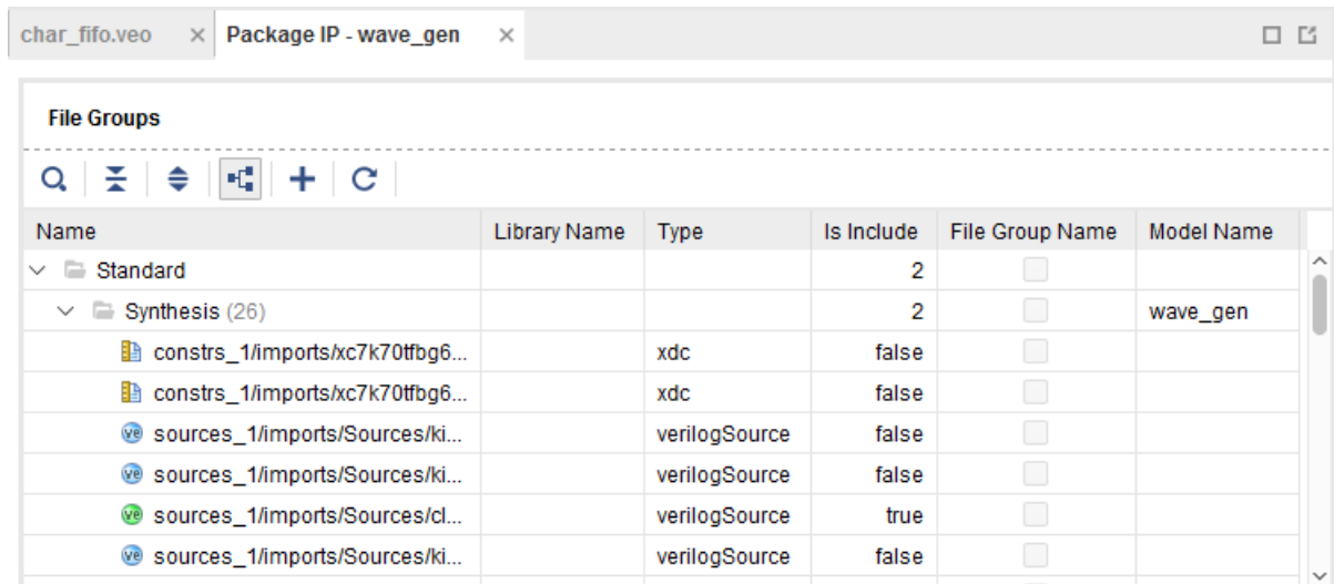
Figure 4-7: File Group List Expansion
