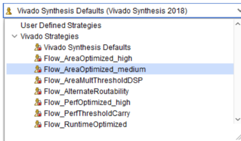
Figure 1-2: Options - Strategies
