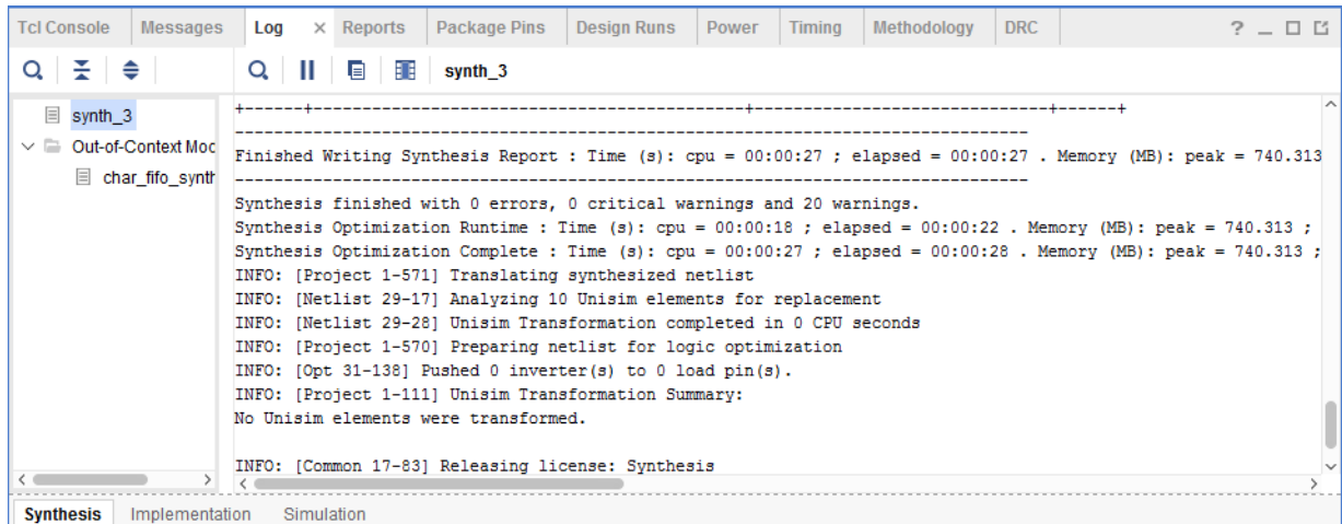
Figure 1-19: Log Window
