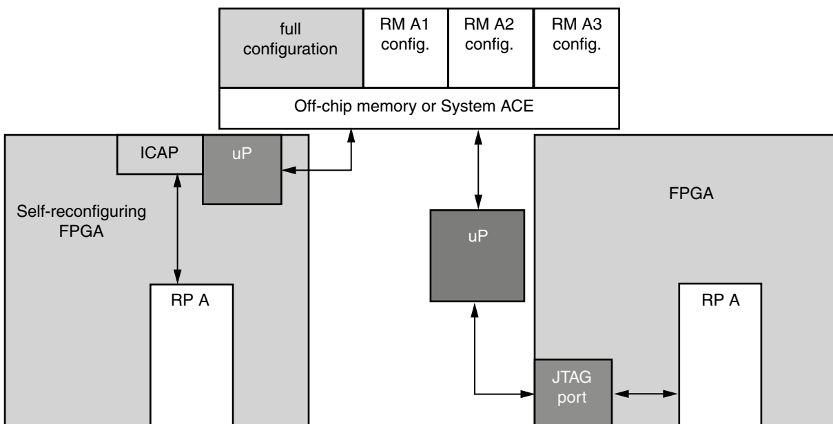
Figure 8-5: Configuring Through a Microprocessor
