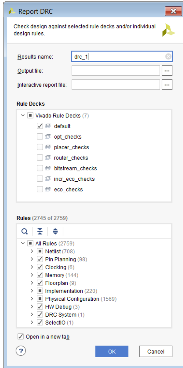
Figure 6-1: Report DRC Dialog Box
