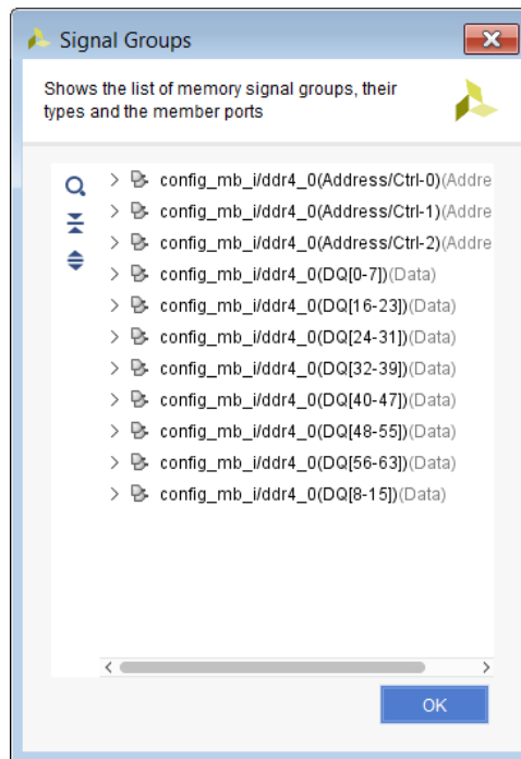
Figure 22: Showing Signal Groups
