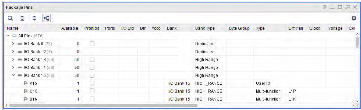
Figure 11: Package Pins Window
