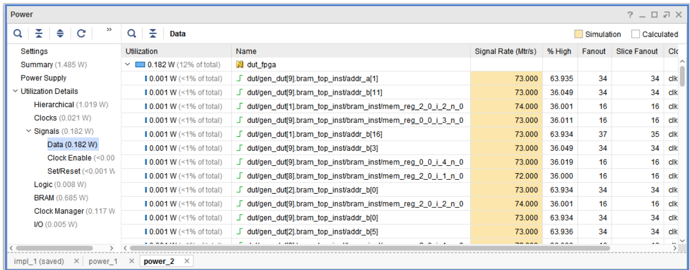
Figure 38: Power Report Signals > Data View - Simulation SAIF Data for Signal Rates
