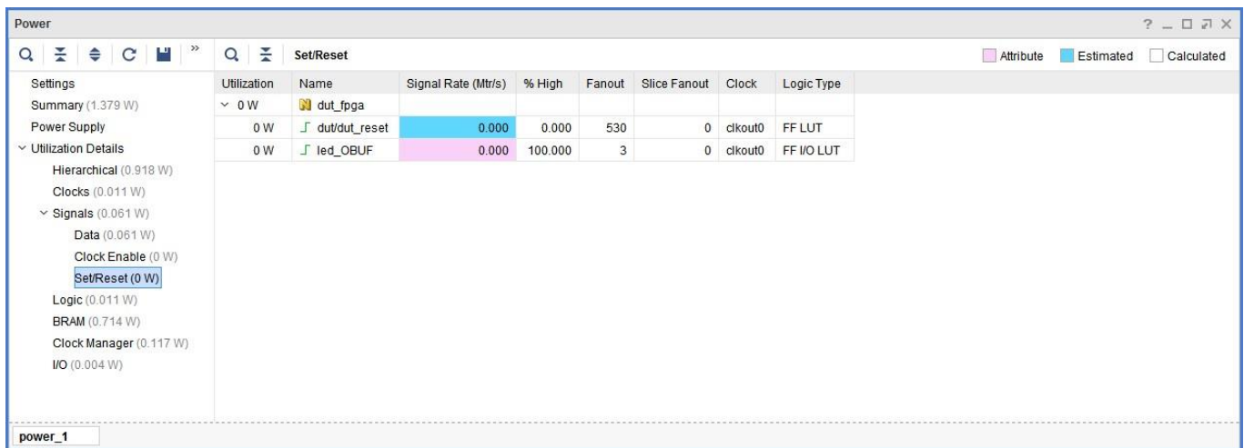
Figure 16: Power Report – Set/Reset Display
