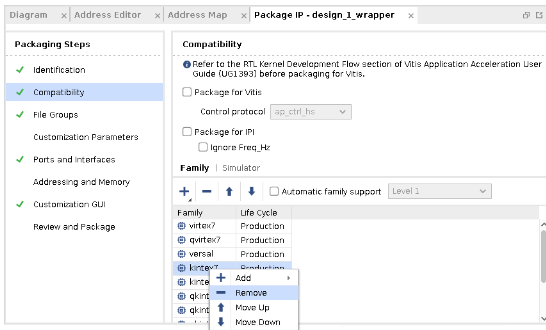
Figure 4-7: Individually Excluding Families
