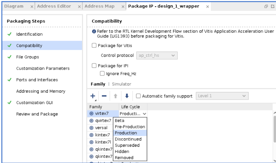
Figure 4-8: Editing the Life Cycle
