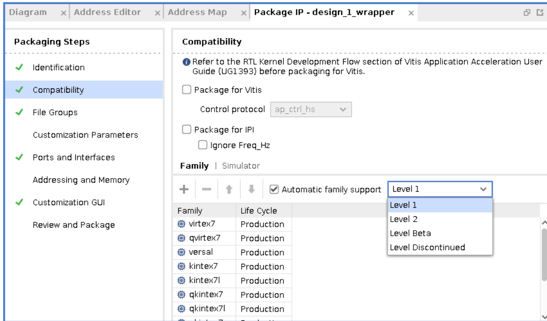
Figure 4-6: Package IP: Compatibility
