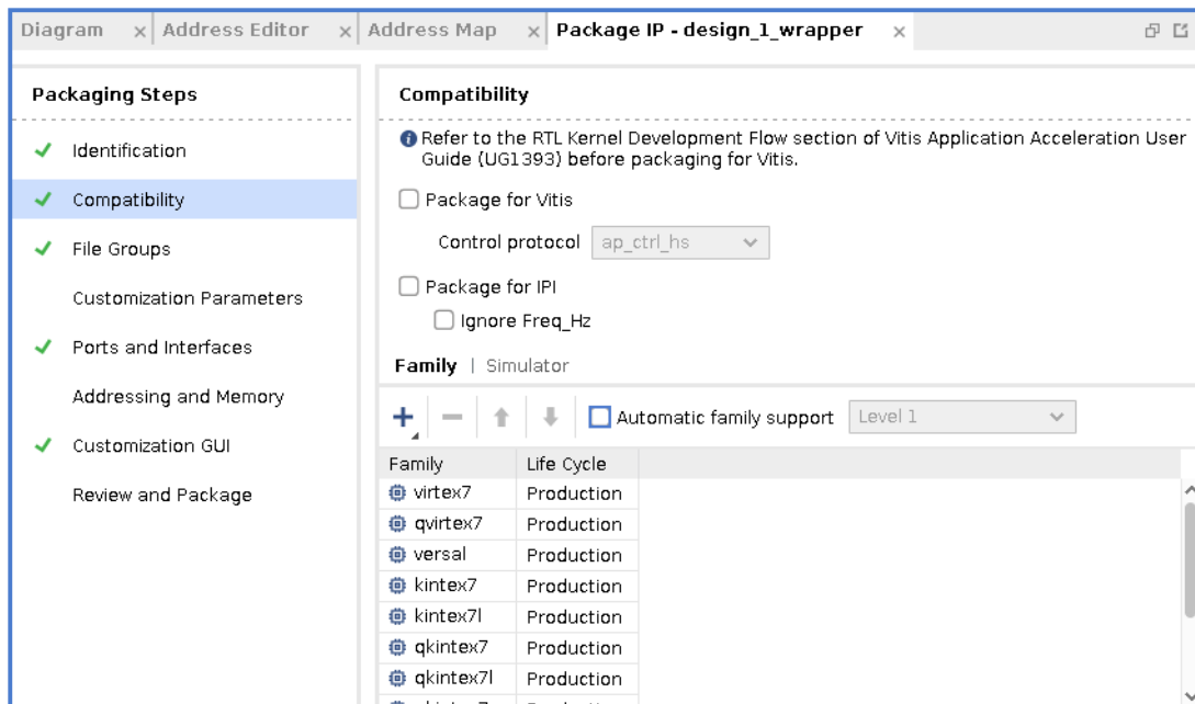
Figure 4-4: Package IP: Compatibility
