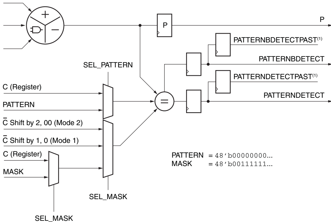
Figure 2-17: Pattern Detector Logic
