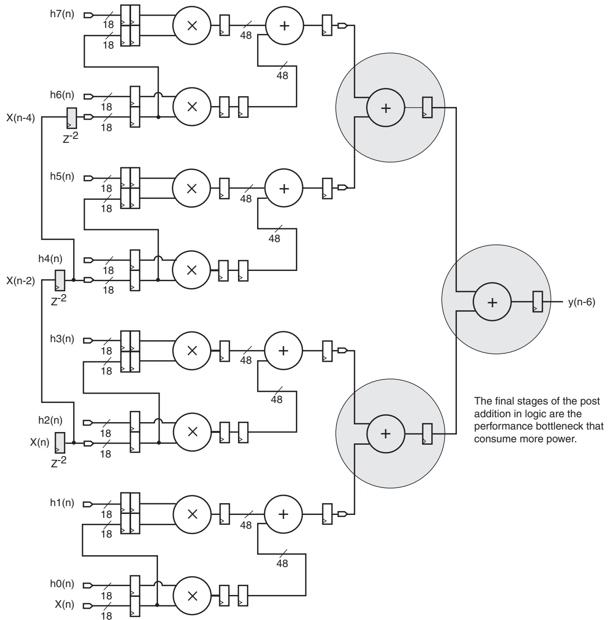
Figure 3-1: Traditional FIR Filter Adder Tree
