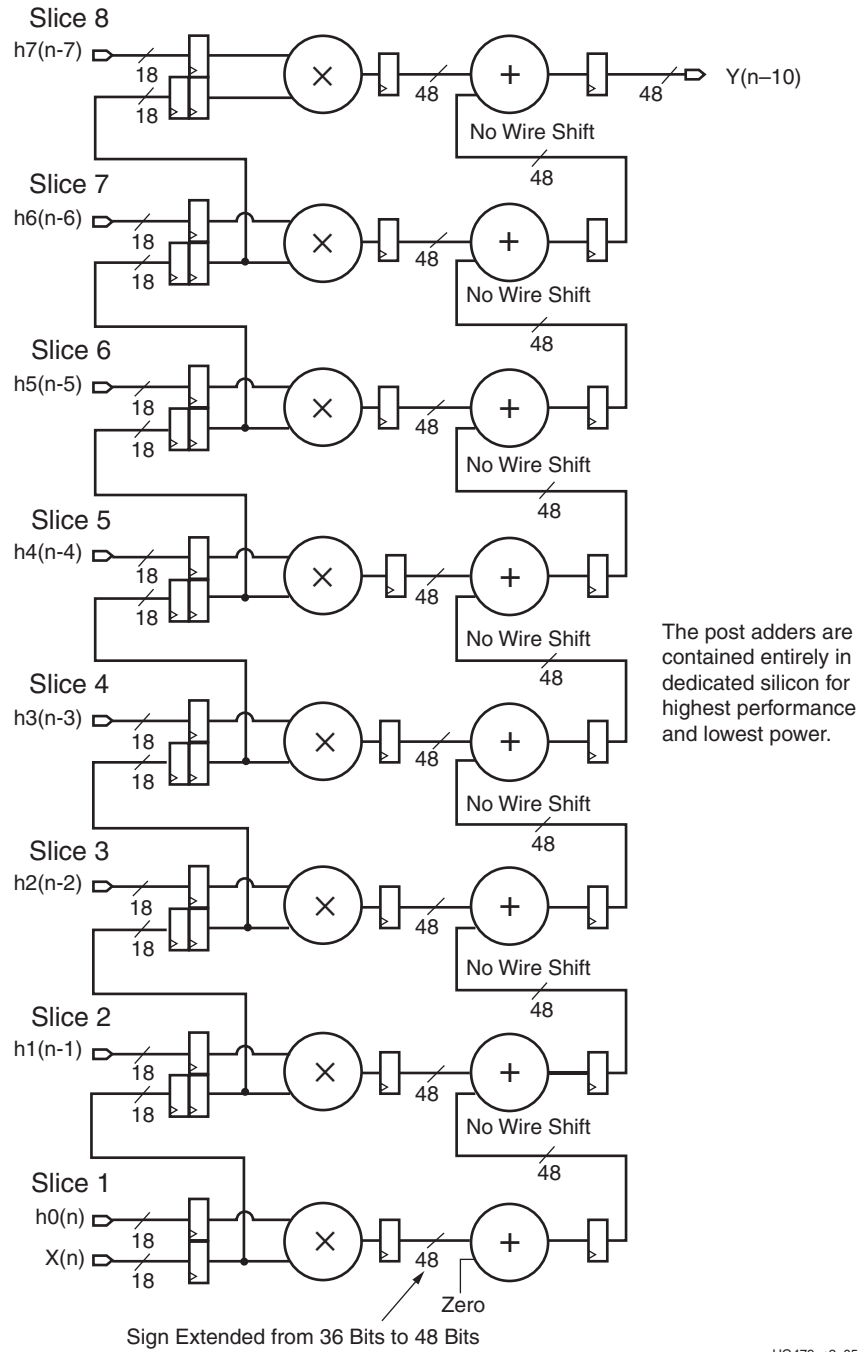
Figure 3-5: Adder Cascade
