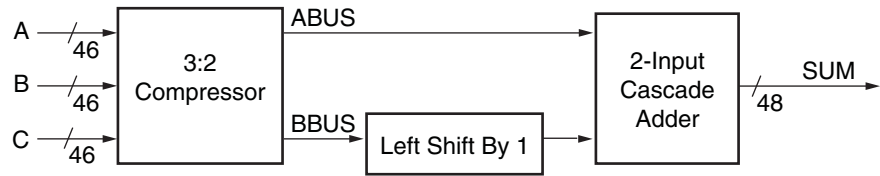
Figure 3-3: Three-Input Adder
