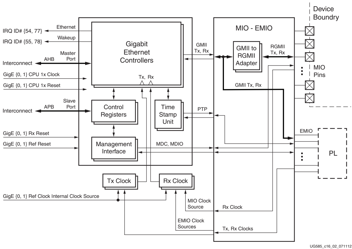
Figure 16-2: System Viewpoint
