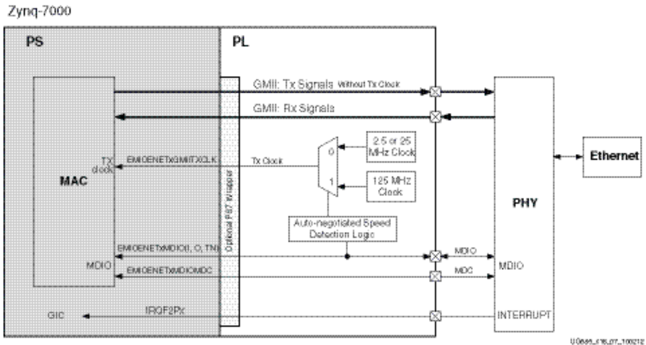
Figure 16-7: GMII Interface via EMIO Connections
