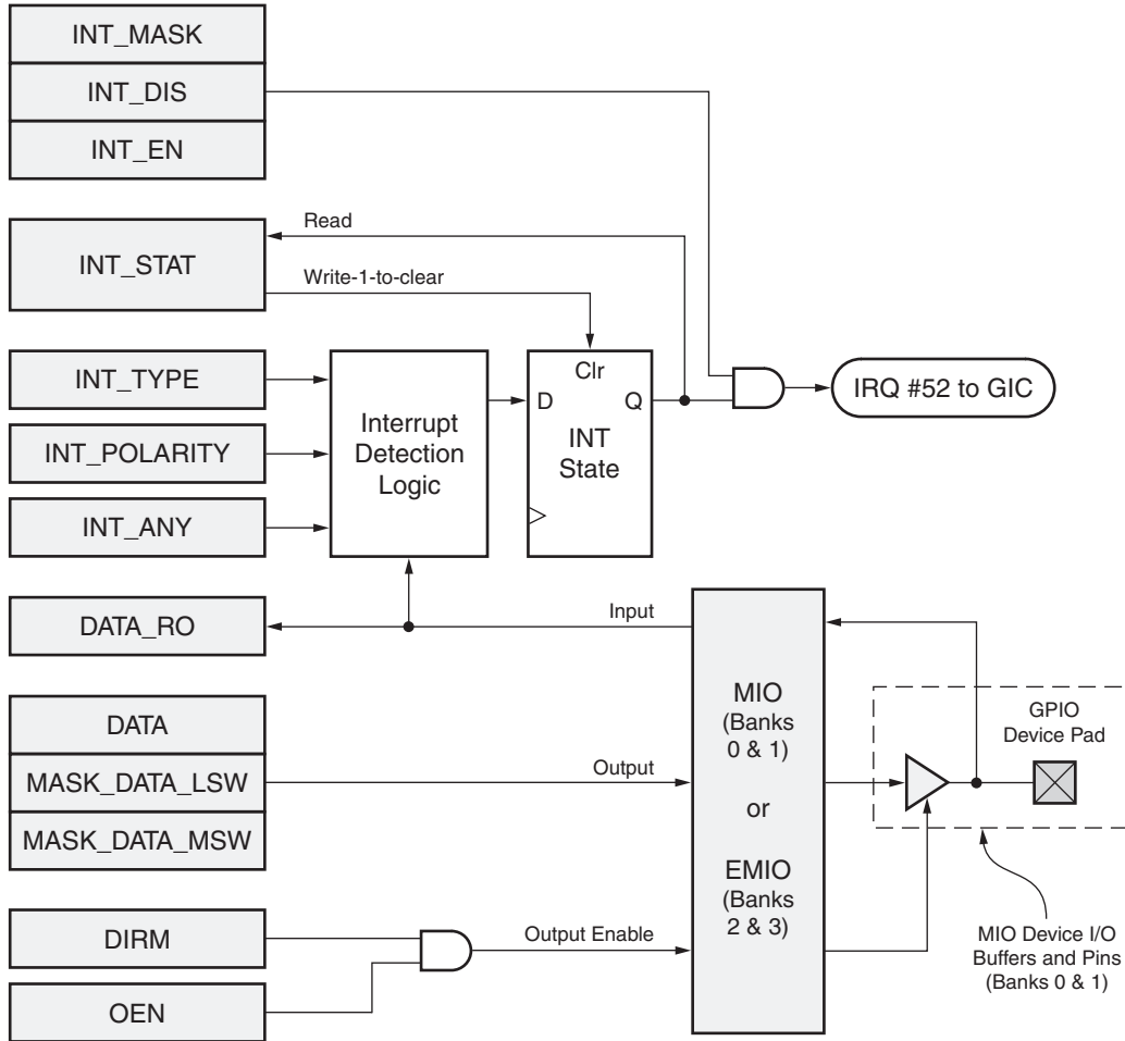
Figure 14-2: GPIO Channel
