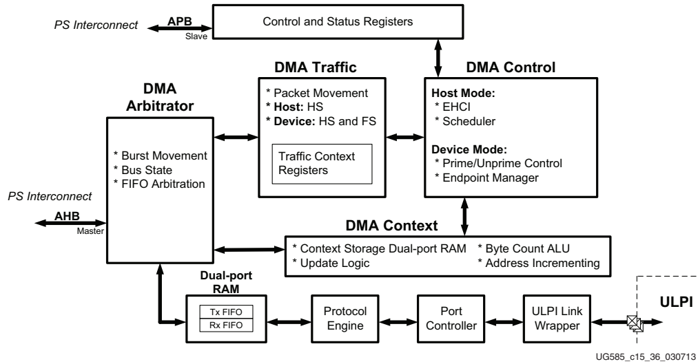
Figure 15-7: USB DMA Controller Block Diagram
