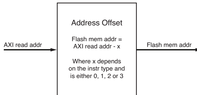
Figure 12-4: Automatic Address Offset For Word Alignment
