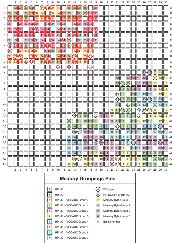
Figure 3-47: FF900/FFG900/FFV900/RF900 Packages—XC7Z035, XC7Z045, and XQ7Z045 Memory Groupings
