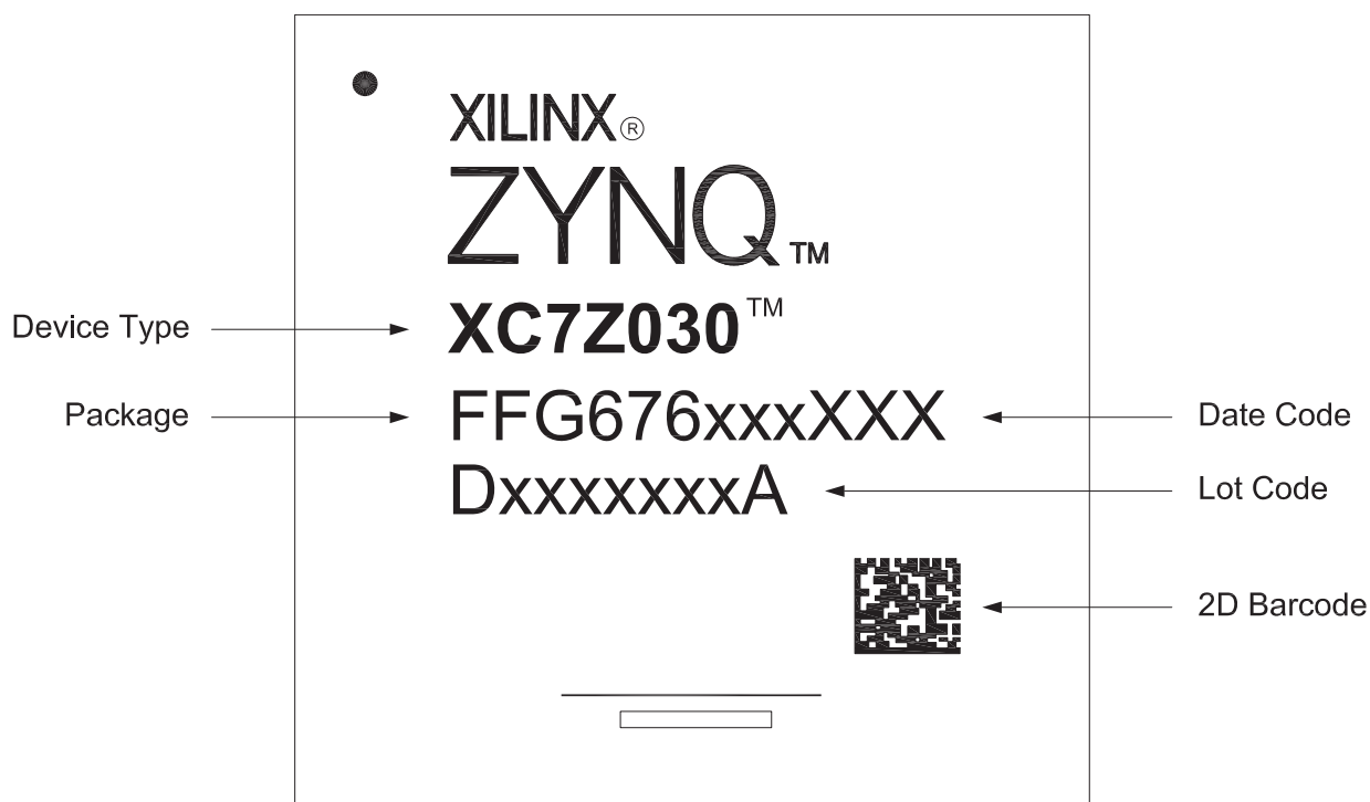
Figure 6-1: Zynq-7000 SoC Device Package Marking with 2D Bar Code
