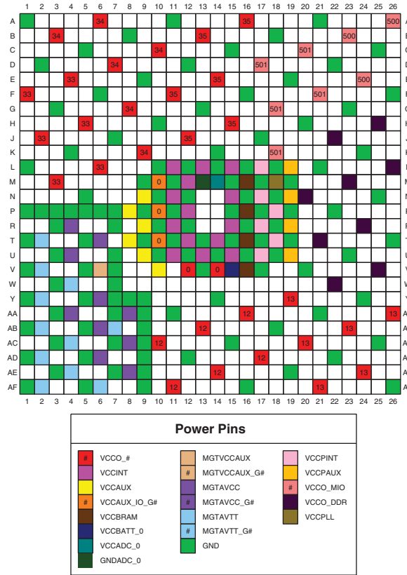
Figure 3-32: FB676/FBG676/FBV676 Packages—XC7Z030 Power and GND Placement
