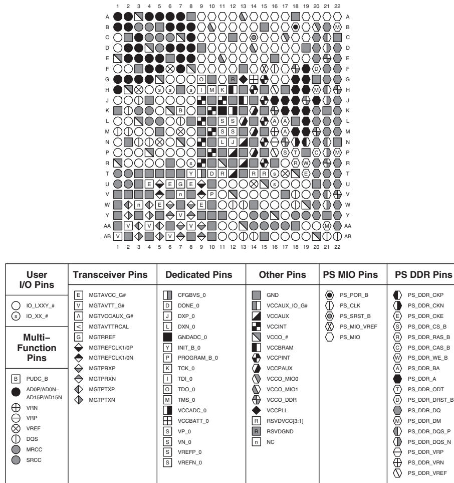
Figure 3-9: CL485/CLG485 Packages—XC7Z012S and XC7Z015 Pinout Diagram
