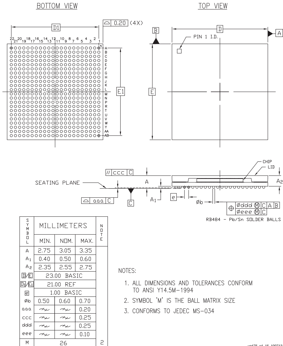
Figure 4-16: RB484 Ruggedized Flip-Chip BGA Package Specifications for XQ7Z030
