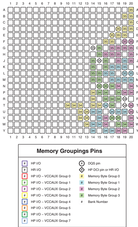
Figure 3-7: CL400/CLG400 Packages—XC7Z007S, XC7Z010, and XA7Z010 Memory Groupings
