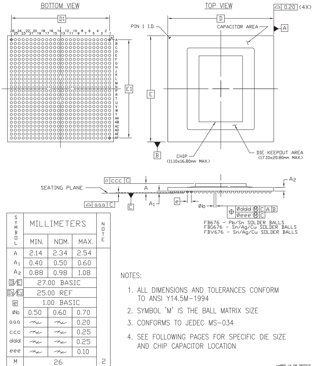
Figure 4-8: FBG676/FBV676 (XC7Z030, XC7Z035, and XC7Z045) Flip-Chip Lidless BGA Package Specifications
