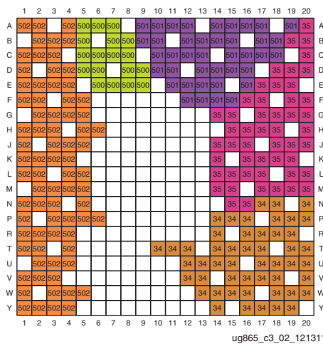
Figure 3-6: CL400/CLG400 Packages—XC7Z007S, XC7Z010, and XA7Z010 I/O Banks
