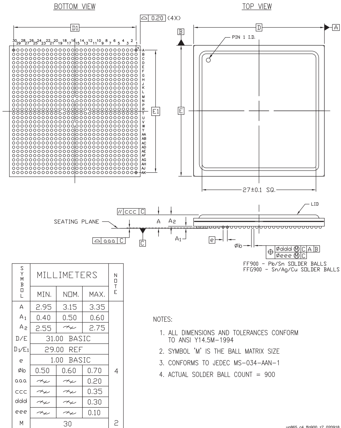
Figure 4-13: FFG900 (XC7Z035, XC7Z045, and XC7Z100) Flip-Chip BGA with Stamped Lid Package Specifications
