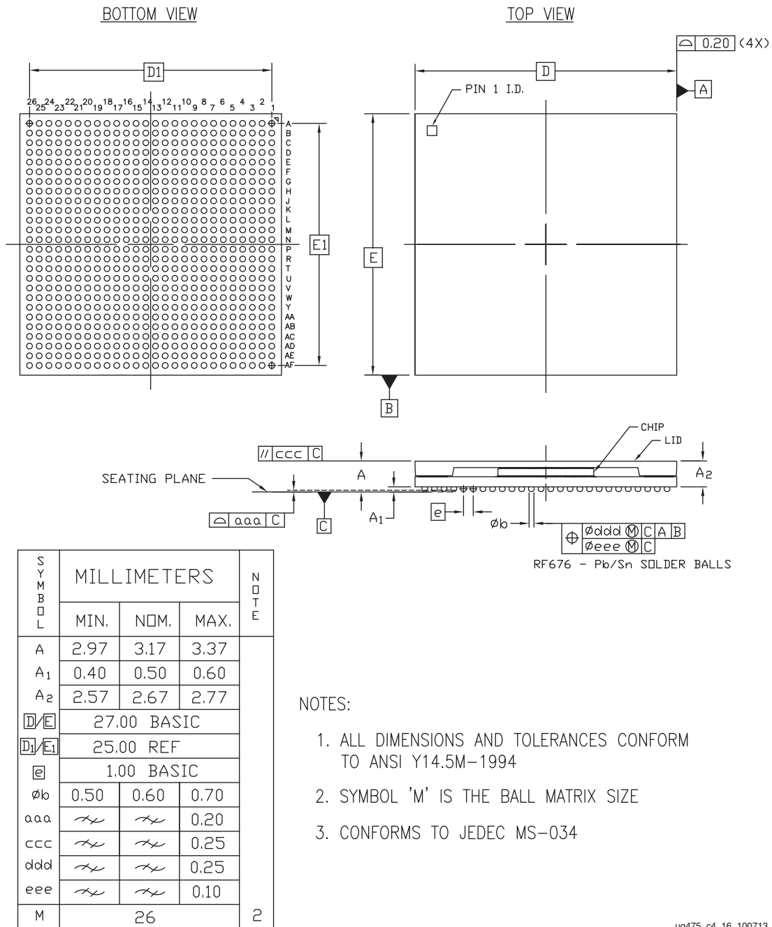
Figure 4-17: RF676/RFG676 Ruggedized Flip-Chip BGA Package Specifications for XQ7Z030 and XQ7Z045
