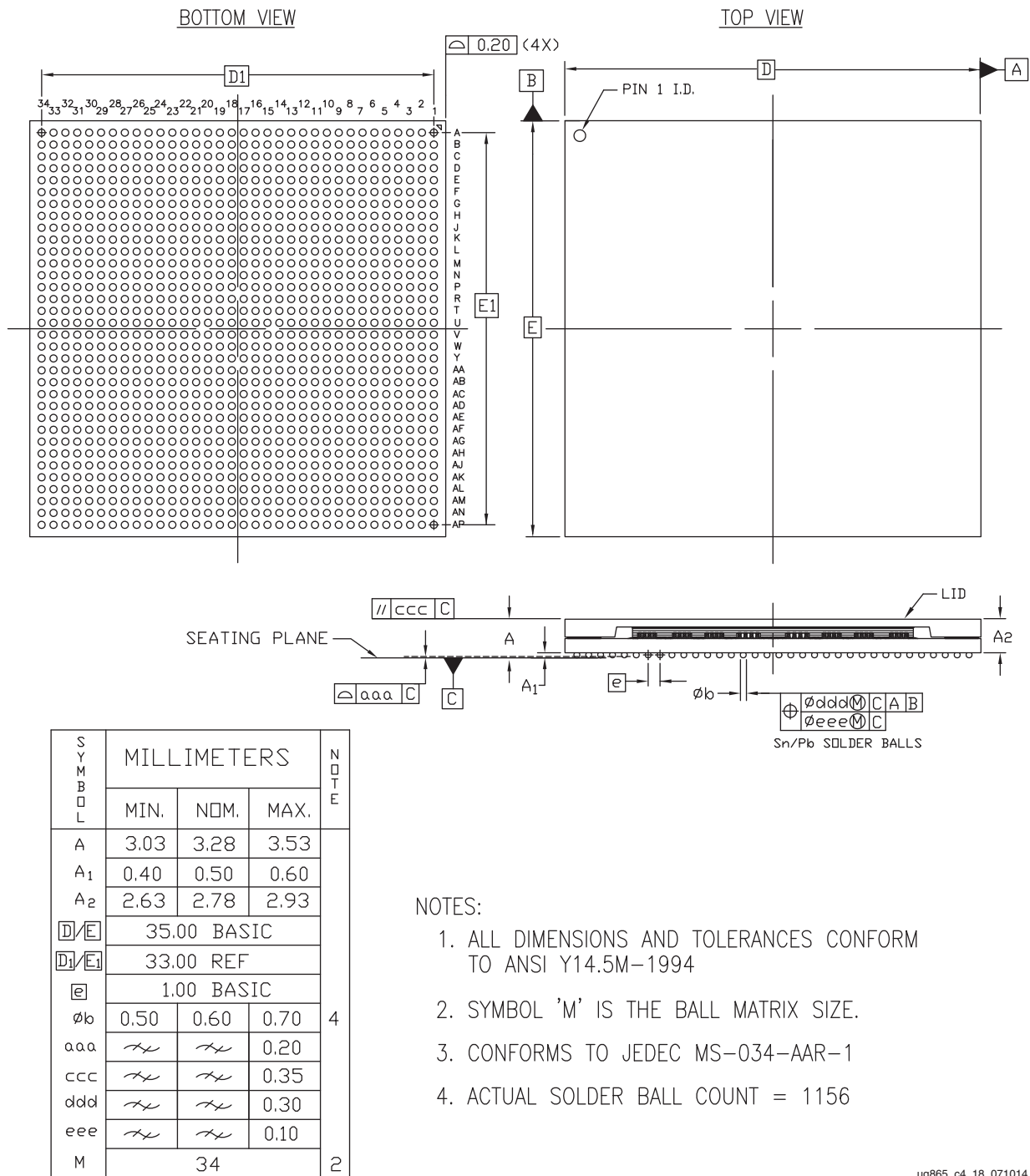
Figure 4-19: RF1156 Ruggedized Flip-Chip BGA Package Specifications for the XQ7Z100
