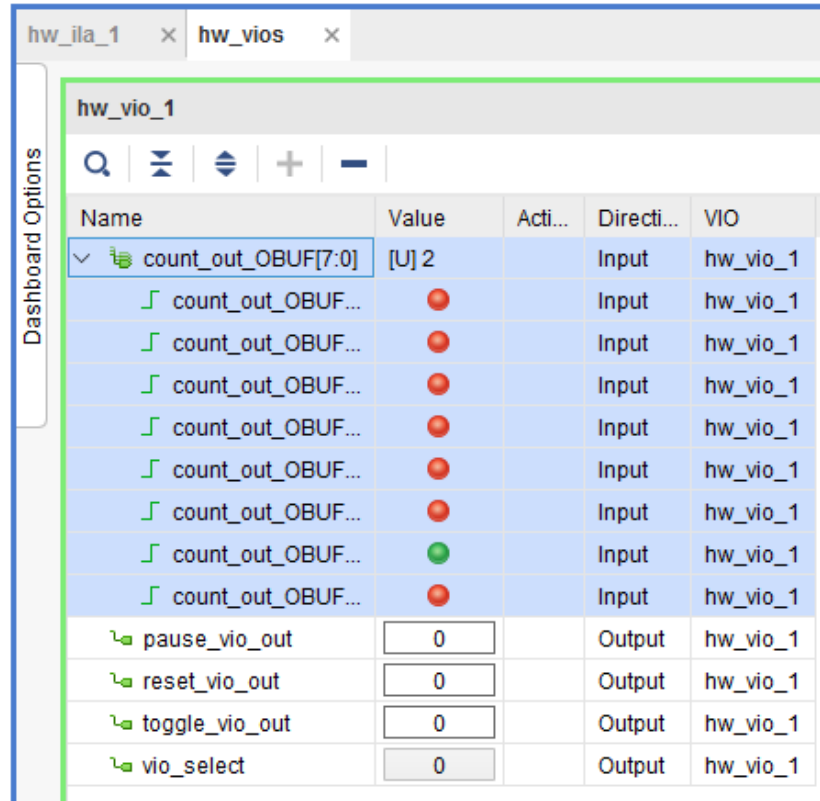
Figure 72: Initial VIO dashboard for debugging
