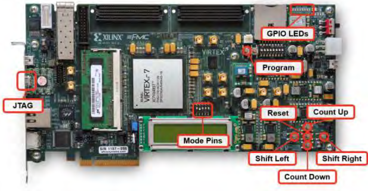
Figure 87: Push buttons, switches and connections on the VC707 demonstration board
