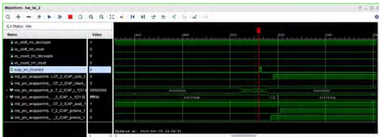
Figure 105: Waveform capture showing icap_err_inserted, PRERROR, PRDONE, and decouple asserted
