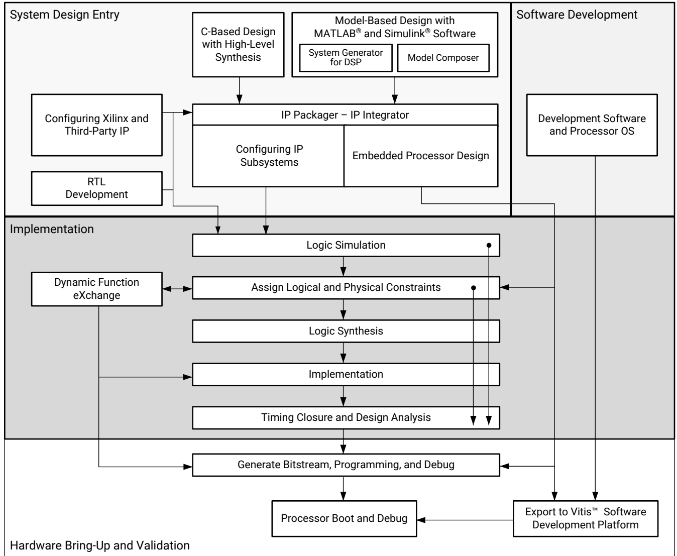
Figure 1: Vivado Design Suite High-Level Design Flow
