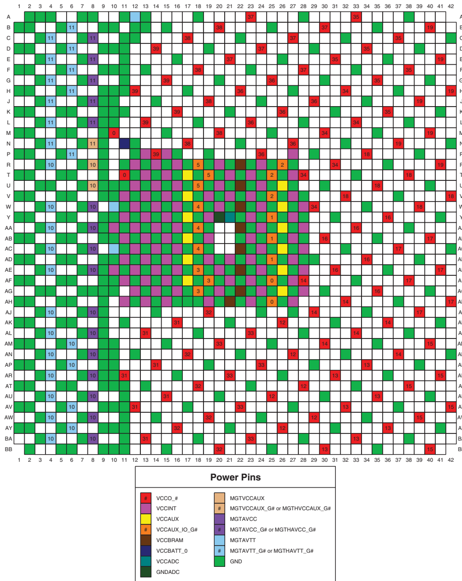
Figure 3-148: FH1761 and FHG1761 Packages—XC7V2000T Power and GND Placement
