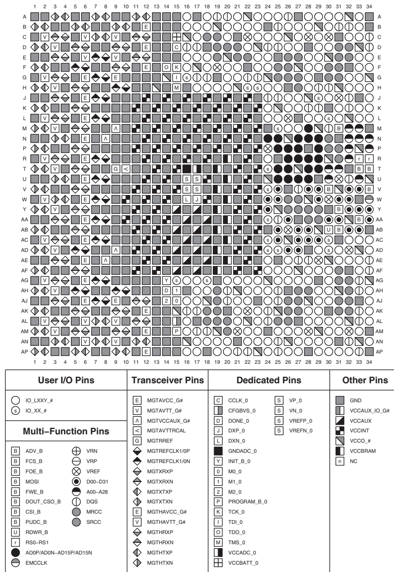
Figure 3-129: FF1156, FFG1156, and FFV1156 Packages—XC7K420T and XC7K480T Pinout Diagram
