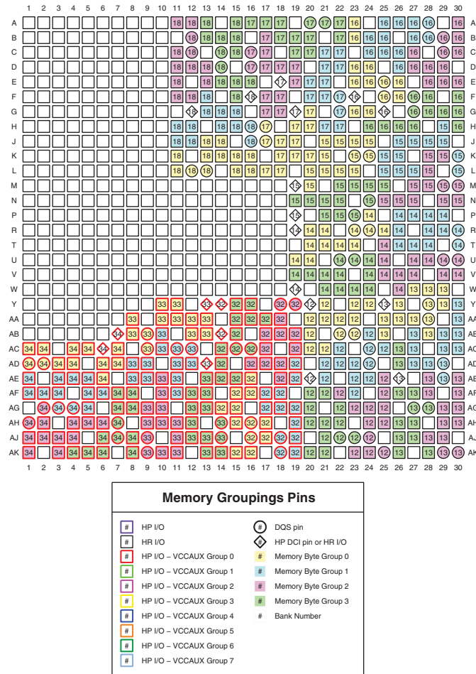
Figure 3-119: FF900, FFG900, FFV900, and RF900 Packages—XC7K325T and XC7K410T Memory Groupings
