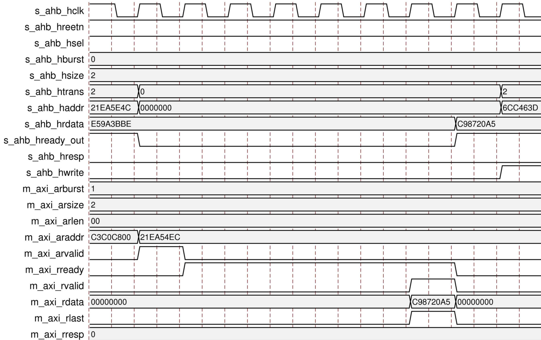
Figure 3-2: Read Transfer with Burst Type SINGLE
