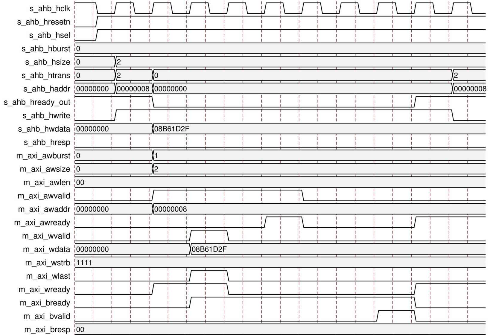
Figure 3-1: Write Transfer with Burst Type SINGLE
