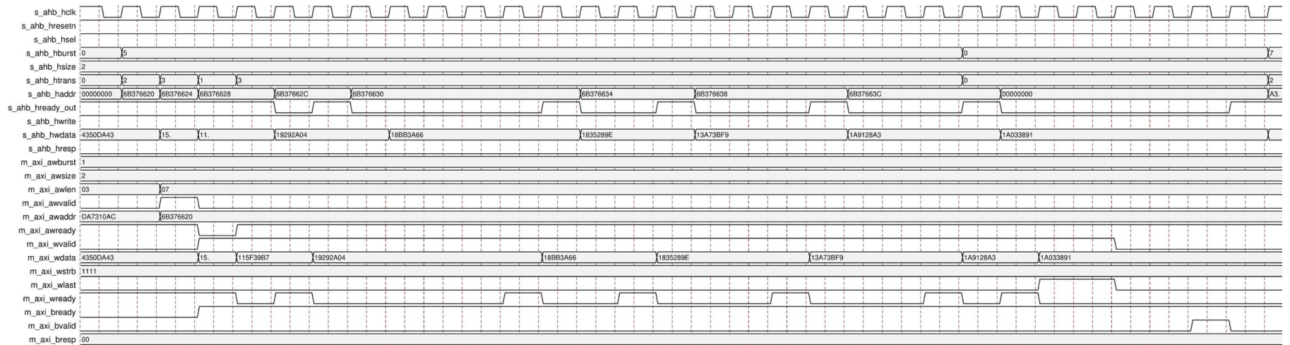
Figure 3-4: Write Transfer with Burst Type INCR8
