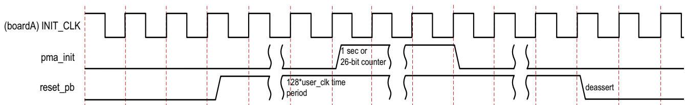
Figure 3-3: Aurora 64B/66B Duplex Normal Operation Reset Sequence
