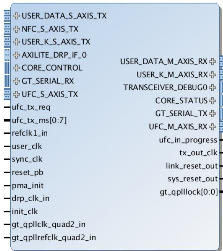
Figure 2-4: Aurora 64B/66B IP Symbol
