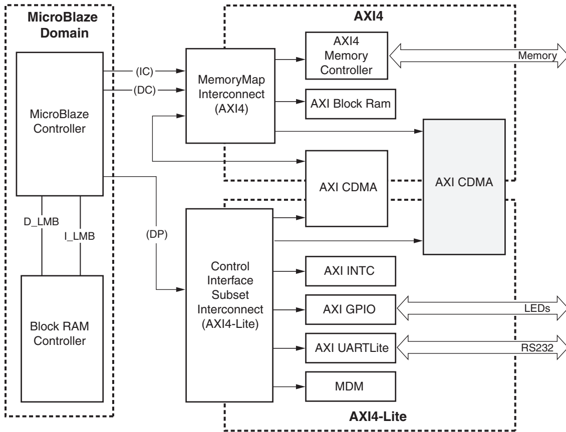
Figure 20: Virtex-6 and Spartan-6 FPGA System Configuration Diagram
