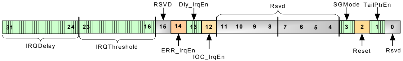
Figure 4: CDMACR Register
