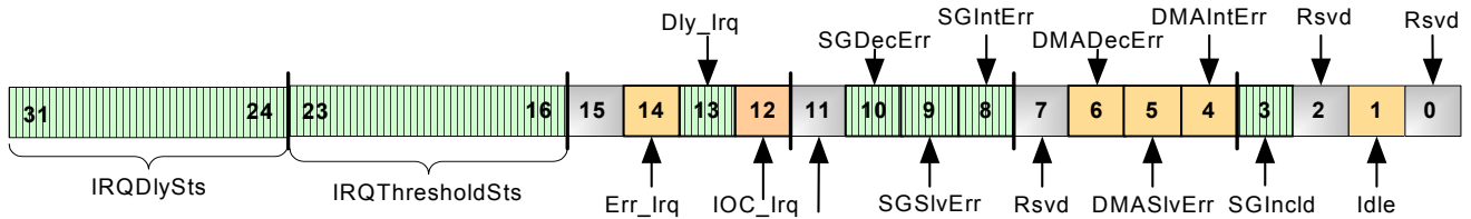
Figure 5: CDMASR Register
