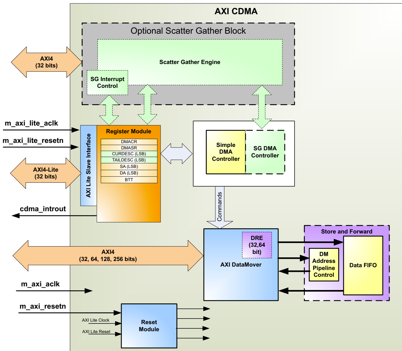
Figure 1: AXI CDMA Block Diagram
