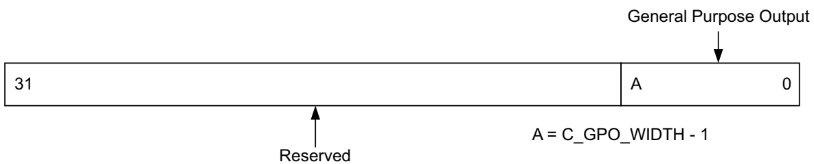
Figure 2-13: General Purpose Output Register (GPO)
