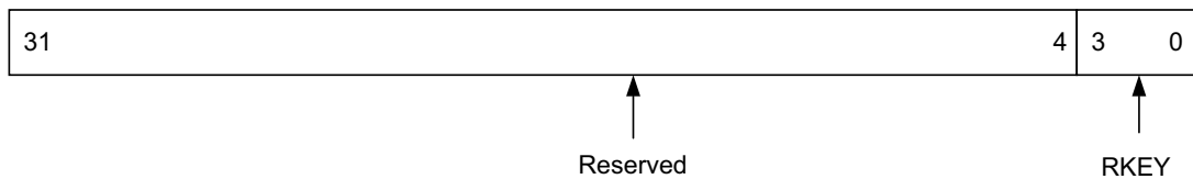
Figure 2-3: Soft Reset Register (SOFTR)
