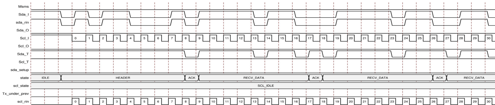
Figure 3-5: Slave Mode – Transmitting Data
