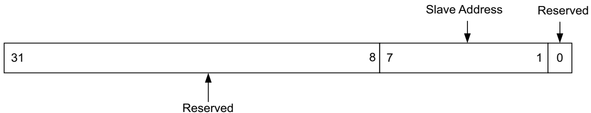
Figure 2-8: Slave Address Register (ADR)
