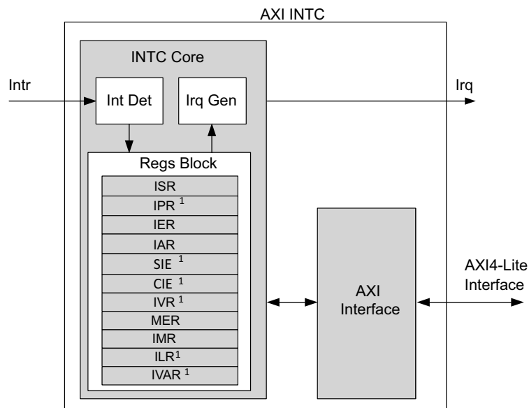
Figure 1-1: AXI INTC Core Block Diagram
