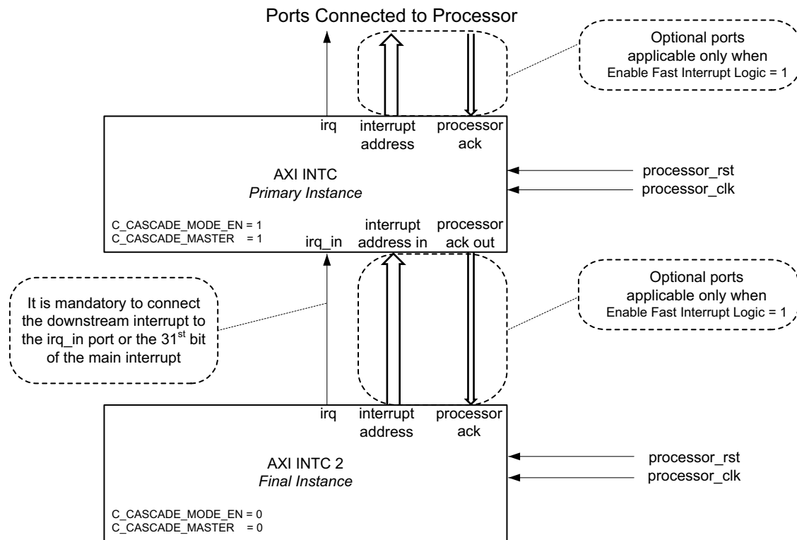
Figure 3-1: Cascade Mode
