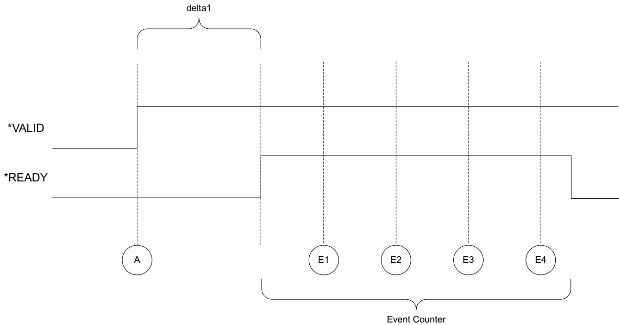
Figure C-20: GEN_AFTER_VALID_EVENTS/RAND_AFTER_VALID_EVENTS
