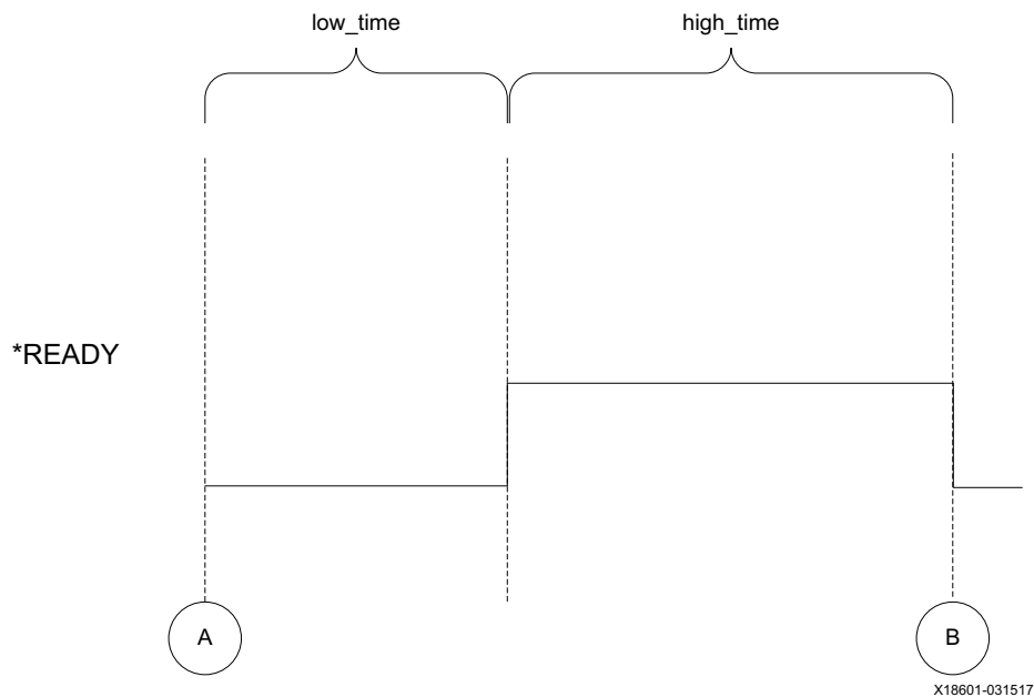
Figure C-17: GEN_OSC/RAND_OSC
