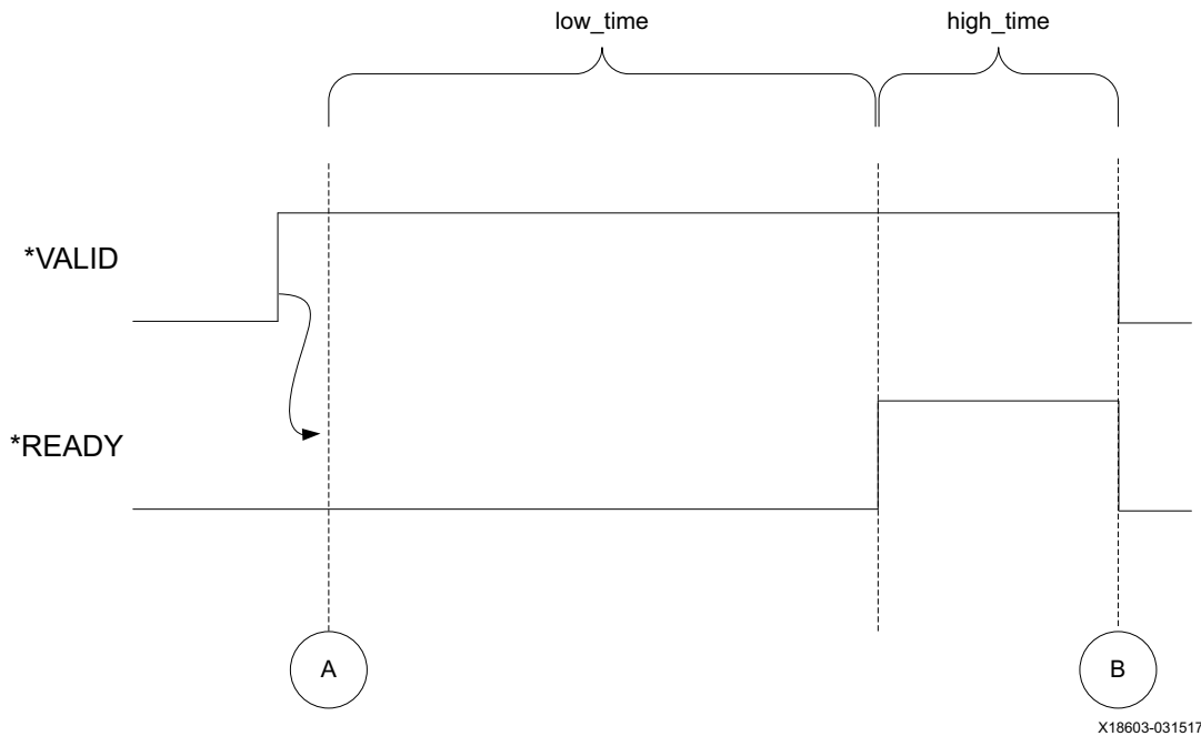
Figure C-16: GEN_SINGLE/RAND_SINGLE
