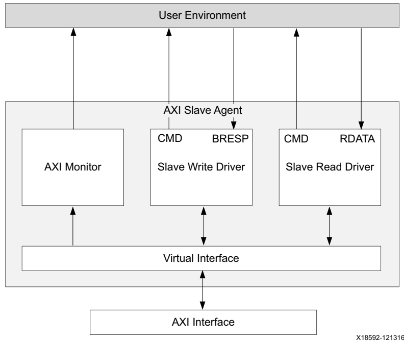
Figure C-8: AXI Slave VIP Agent
