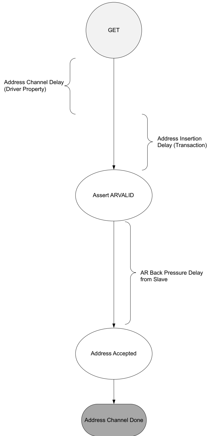
Figure C-4: Read Command Diagram
