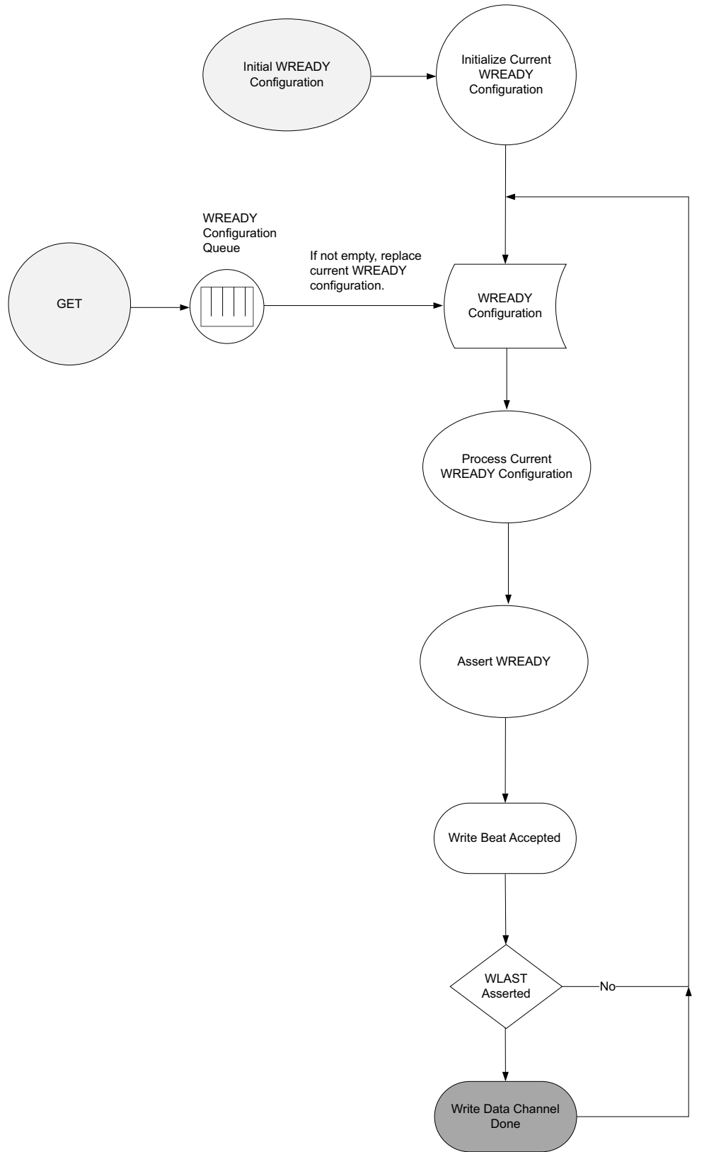
Figure C-12: WREADY Timing Flow
