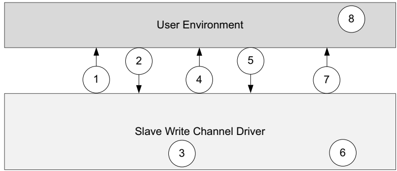
Figure C-10: Write Transaction Flow
