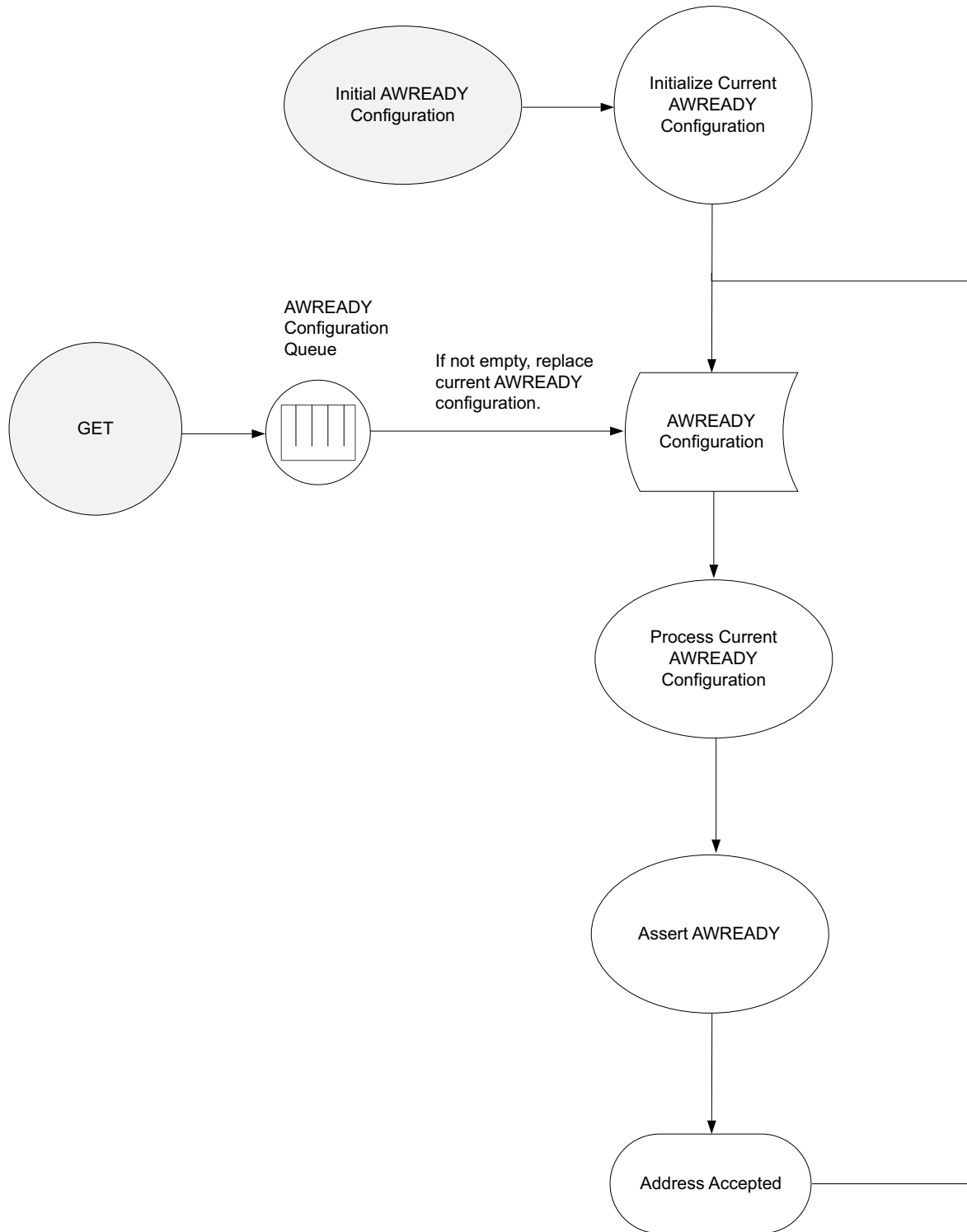
Figure C-11: AWREADY Timing Flow
