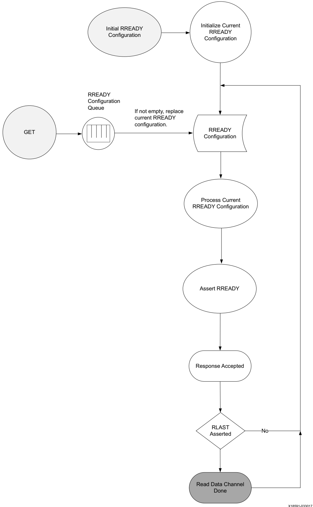
Figure C-7: RREADY Data Flow
