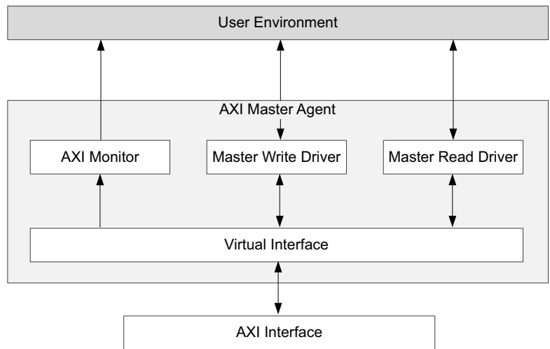
Figure C-1: AXI Master VIP Agent
