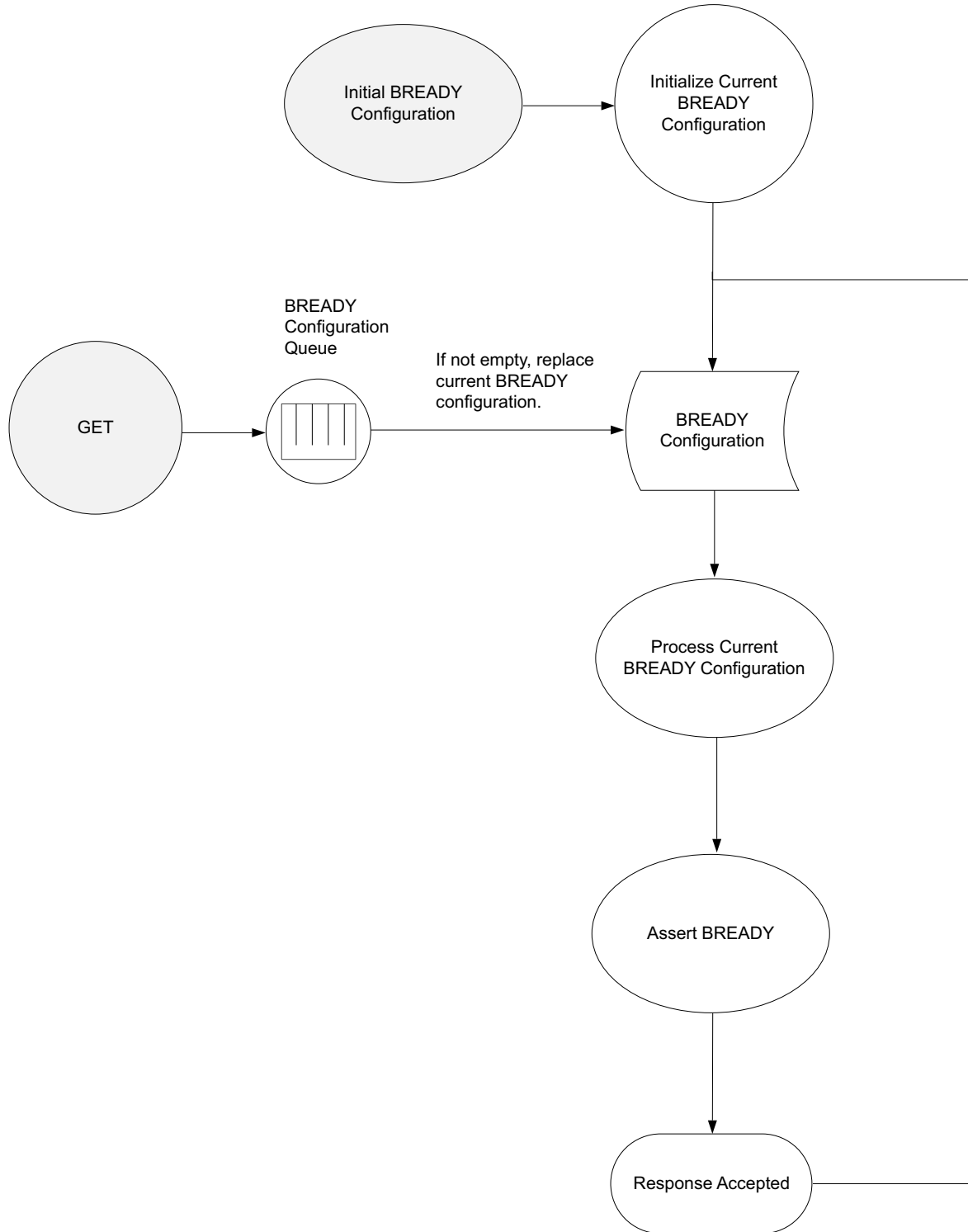
Figure C-6: BREADY Data Flow
