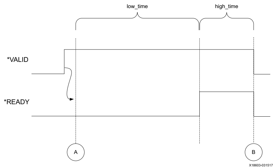
Figure C-21: GEN_AFTER_VALID_OSC/RAND_AFTER_VALID_OSC
