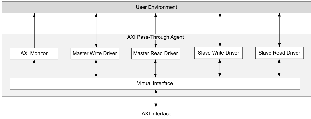
Figure C-15: AXI Pass-Through VIP Agent
