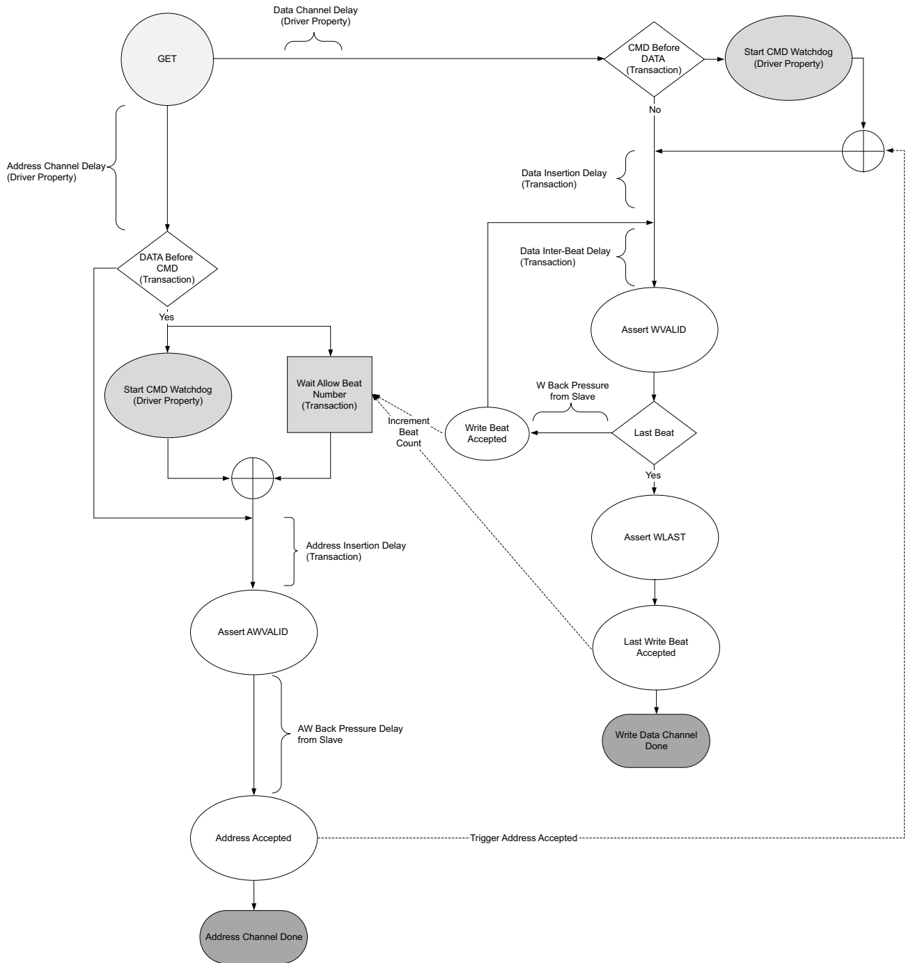
Figure C-2: Write Command and Data Flow
