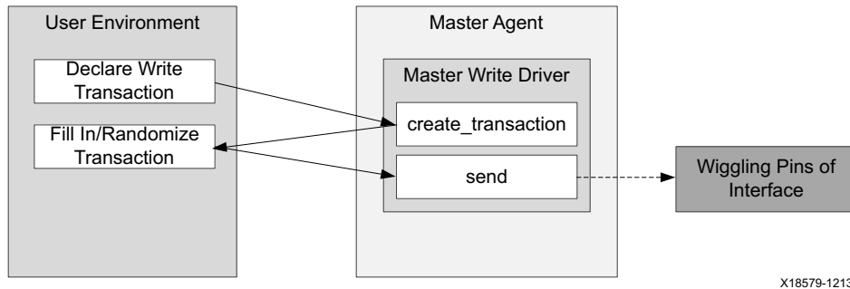
Figure 4-5: Write Transaction Flow
