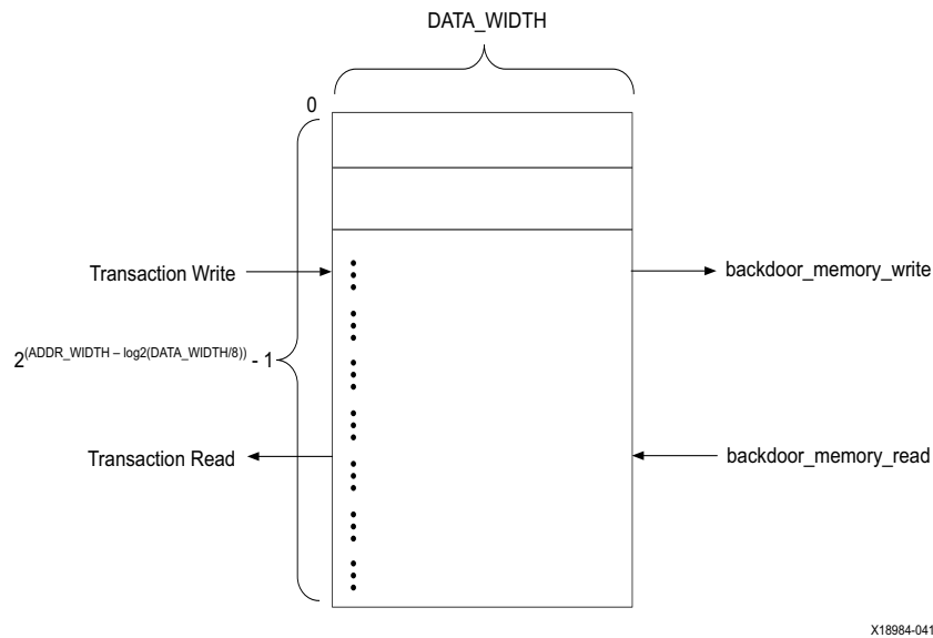
Figure 4-8: Memory Model
