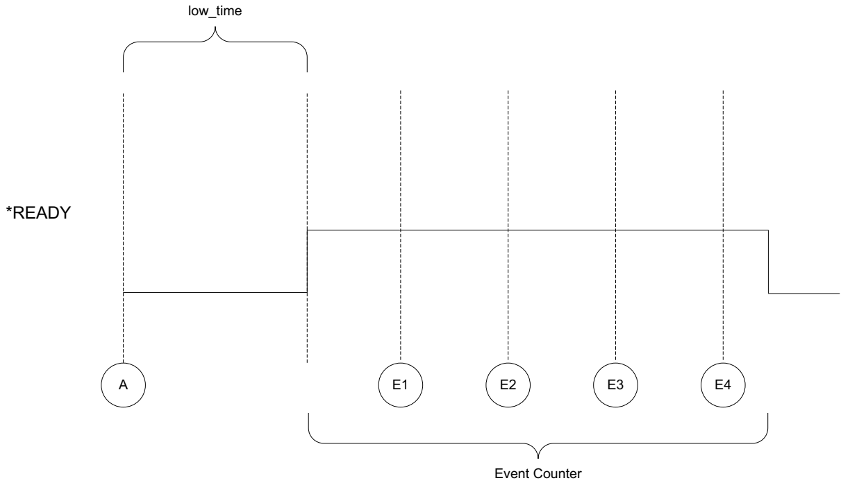
Figure C-18: GEN_EVENTS/RAND_EVENTS
