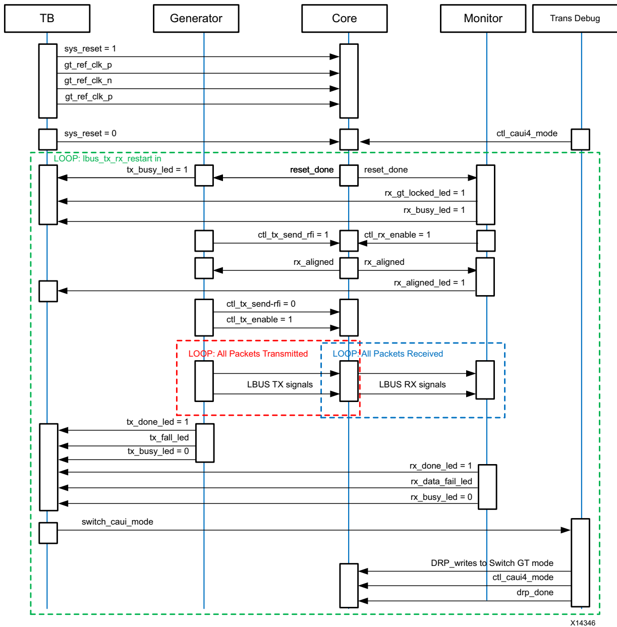
Figure 5-19: Simulation Use Case for Runtime Selectable Mode
