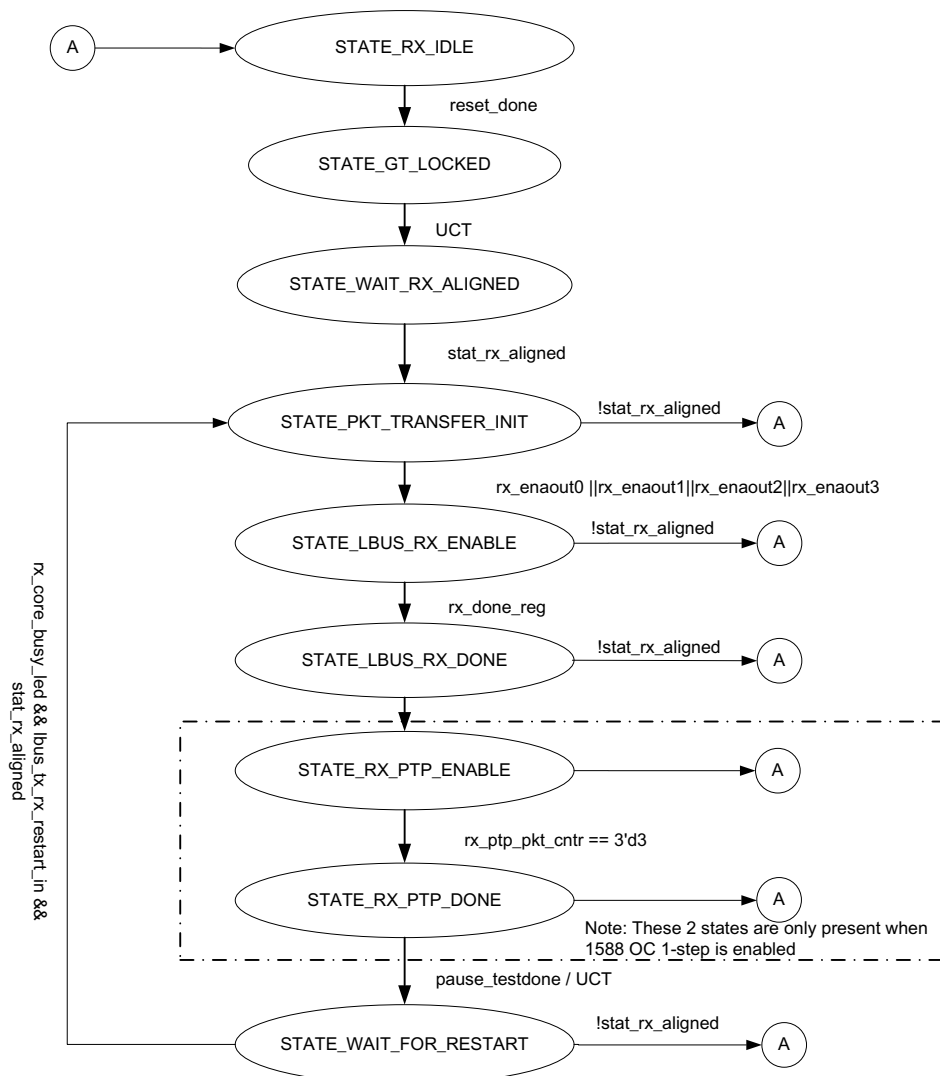
Figure 5-8: State Transition Diagram for Packet Monitor
