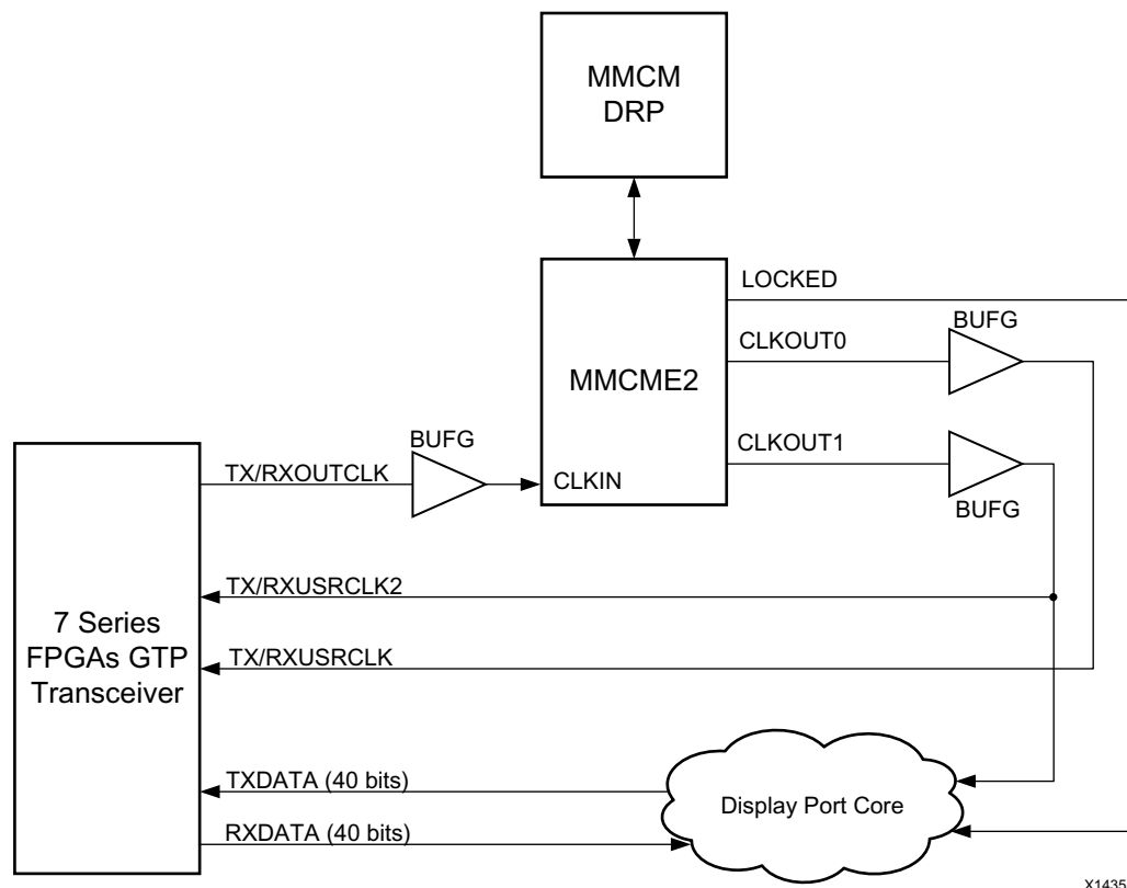
Figure 3-32: 32-Bit GT Interface
