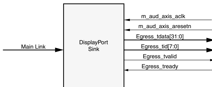
Figure 3-15: Audio Data Interface of DisplayPort Sink System
