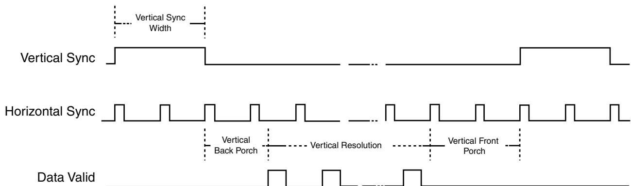
Figure 3-17: User Interface Vertical Timing
