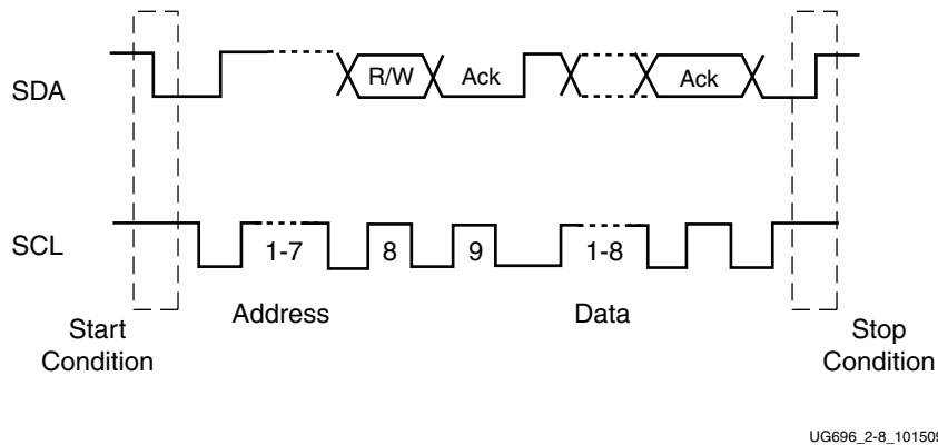
Figure 3-29: I2C Transaction
