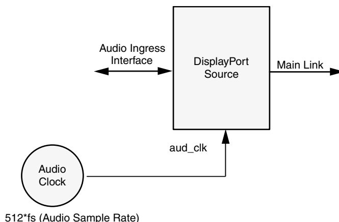
Figure 3-9: Source: Audio Clocking
