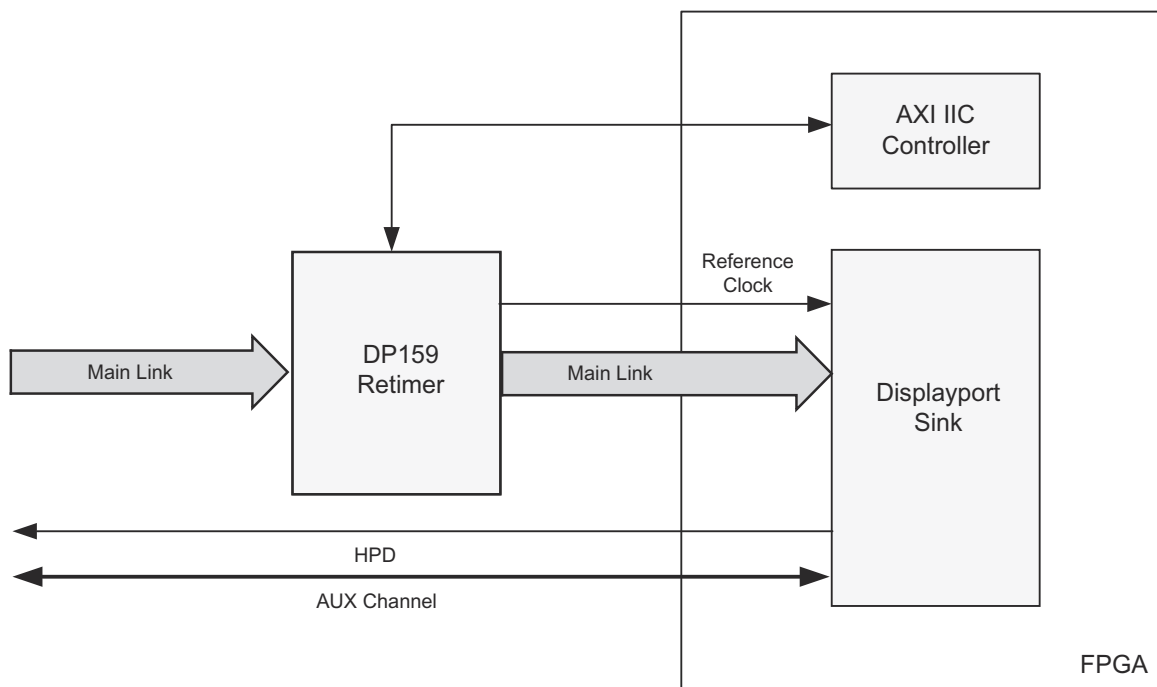
Figure 3-10: DP159 Retimer
