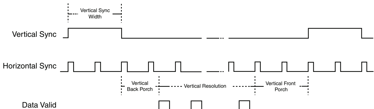
Figure 3-24: User Interface Vertical Timing
