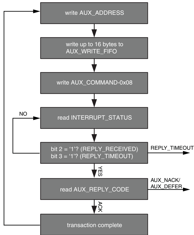
Figure 3-3: AUX Write Transaction
