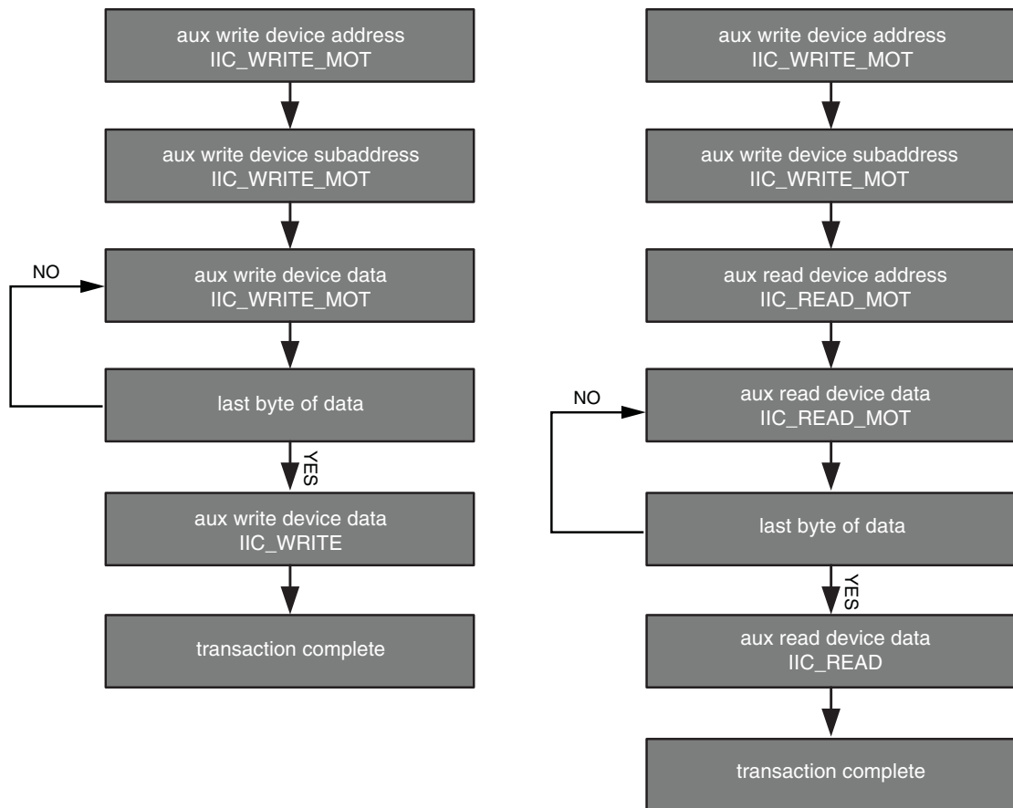
Figure 3-5: Commanded I2C Device Transactions, Write (Left) and Read (Right)
