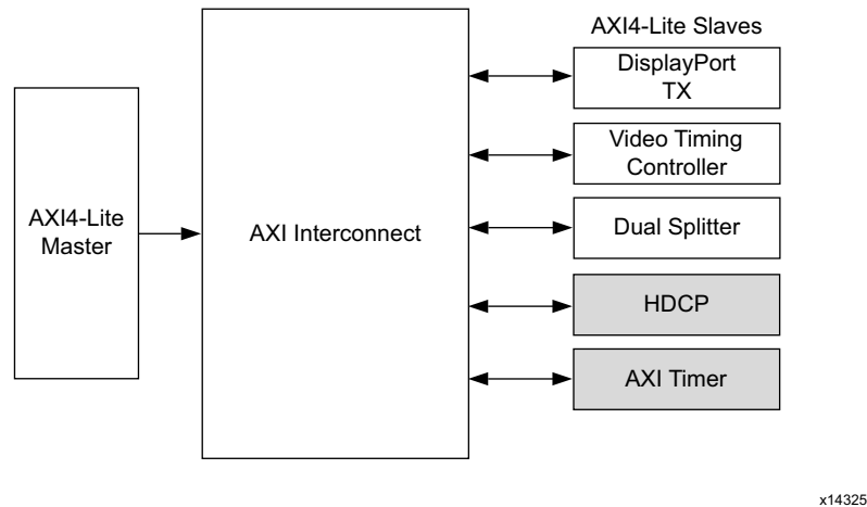
Figure 2-12: AXI4-Lite Interconnect within DisplayPort TX Subsystem
