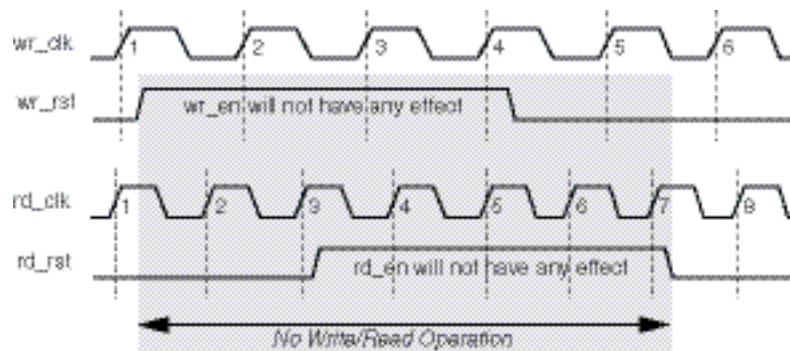
Figure 3-37: Synchronous Reset: FIFO with Independent Clock - wr_rst then rd_rst
