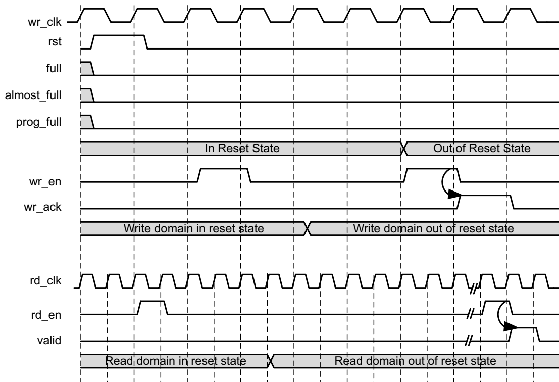
Figure 3-32: Block RAM, Distributed RAM, Shift RAM with Full Flags Reset Value of 0
