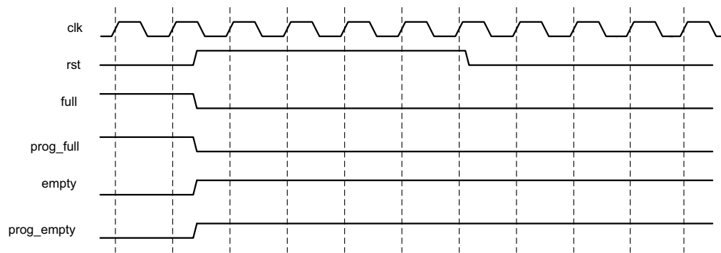
Figure 3-33: Built-in FIFO, Asynchronous Reset Behavior
