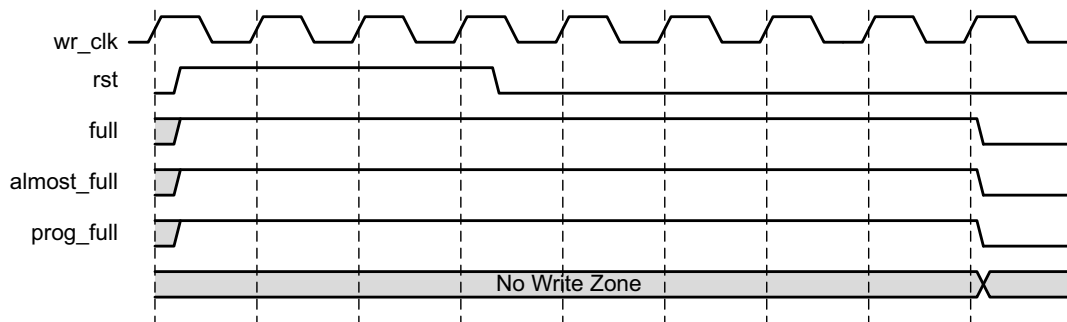
Figure 3-31: Block RAM, Distributed RAM, Shift RAM with Full Flags Reset Value of 1 for the Reset Pulse of More Than One Clock
