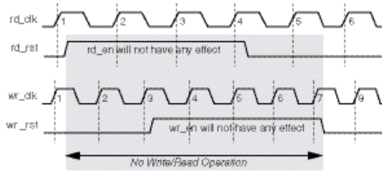
Figure 3-38: Synchronous Reset: FIFO with Independent Clock - rd_rst then wr_rst
