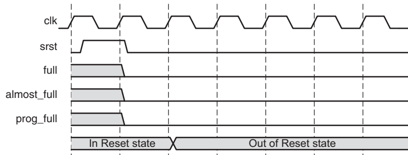
Figure 3-36: Synchronous Reset: FIFO with a Common Clock
