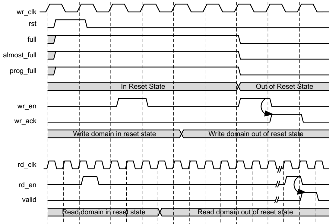
Figure 3-30: Block RAM, Distributed RAM, Shift RAM with Full Flags Reset Value of 1 for the Reset Pulse of One Clock
