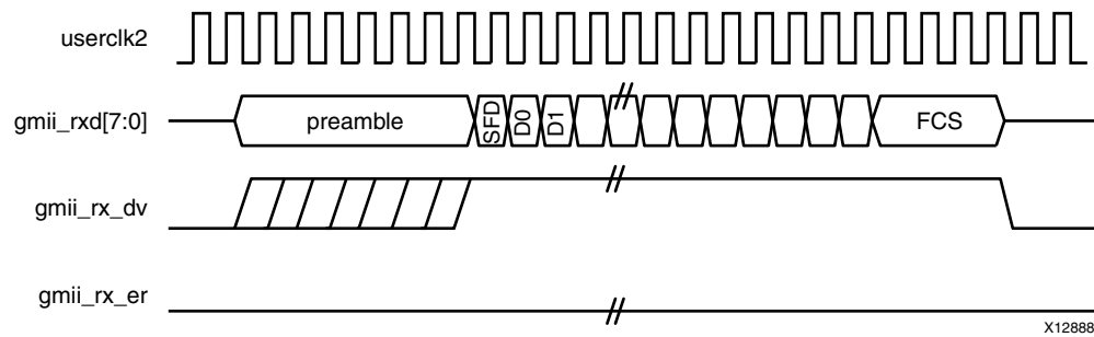
Figure 3-37: GMII Frame Reception at 1/2.5 Gb/s
