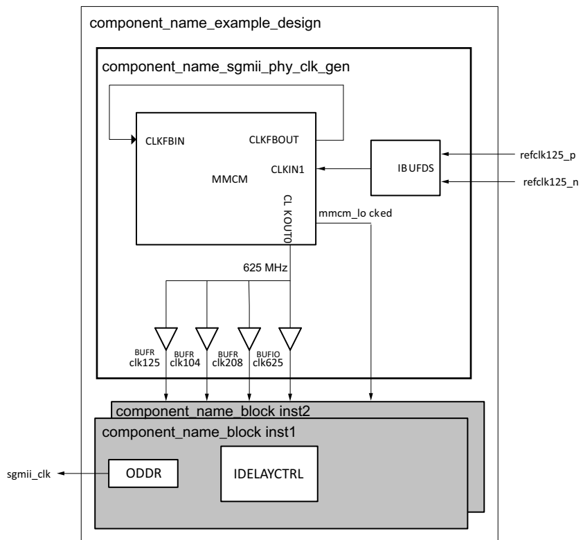
Figure 3-20: Synchronous LVDS Implementation Cloning Logic Using BUFR/BUFRIO
