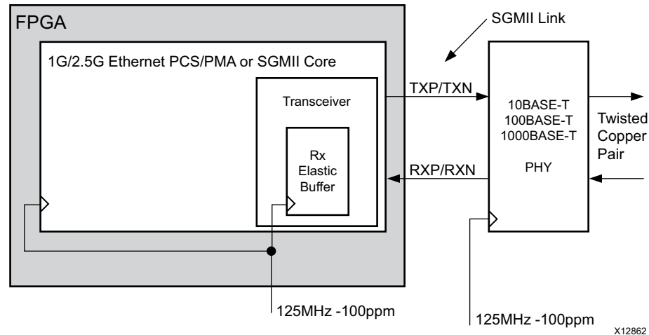
Figure 3-10: SGMII Implementation using Separate Clock Sources
