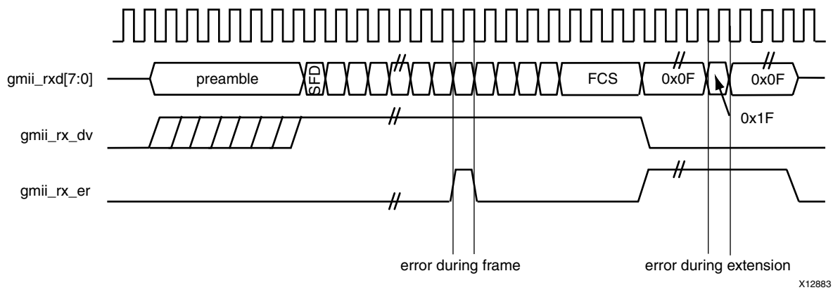
Figure 3-32: GMII Frame Reception with Errors
