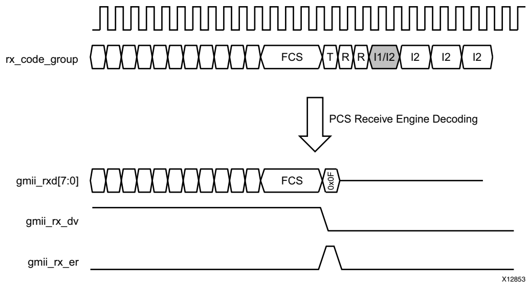
Figure C-8: 100BASE-X Reception State Machine Operation (Odd Case)
