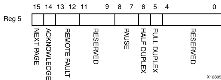
Figure 2-13: MDIO Register 5: Auto-Negotiation Link Partner Base
