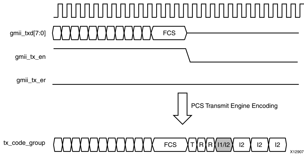
Figure C-7: 100BASE-X Transmit State Machine Operation (Even Case)
