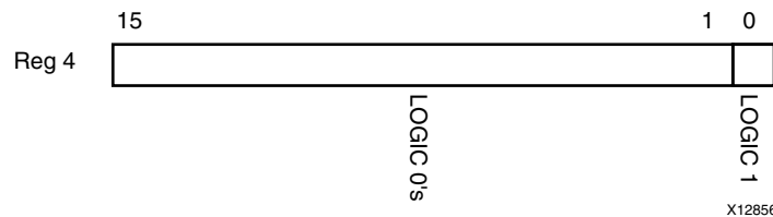
Figure 2-26: MDIO Register 4: SGMII Auto-Negotiation Advertisement
