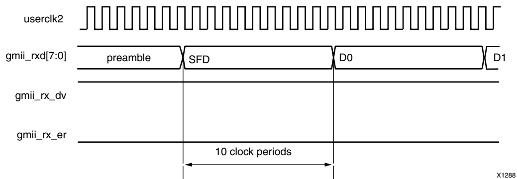
Figure 3-38: GMII Data Reception at 100 Mb/s
