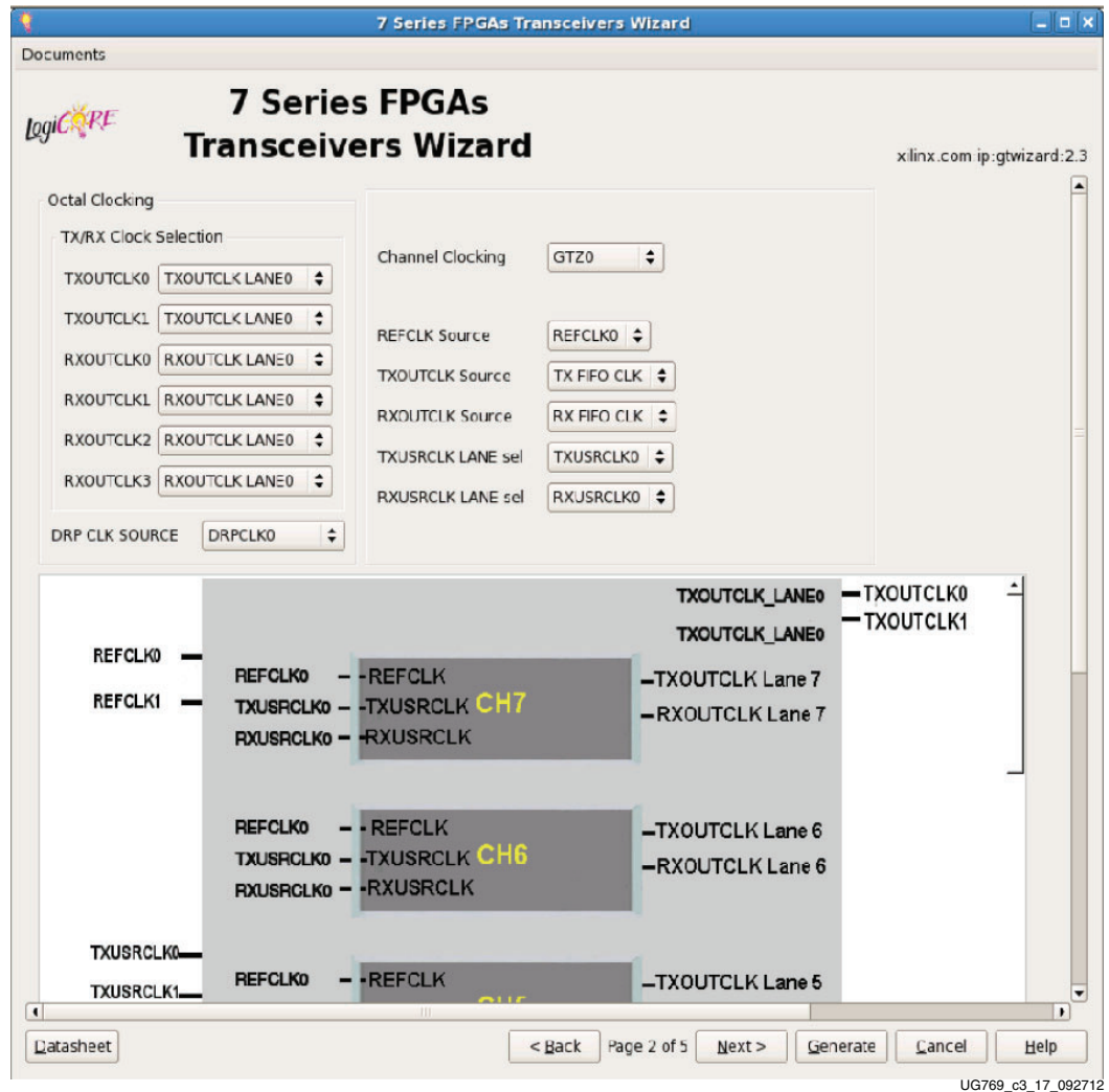
Figure 3-8: Octal and Channel Clocking—GTZ Page 2
