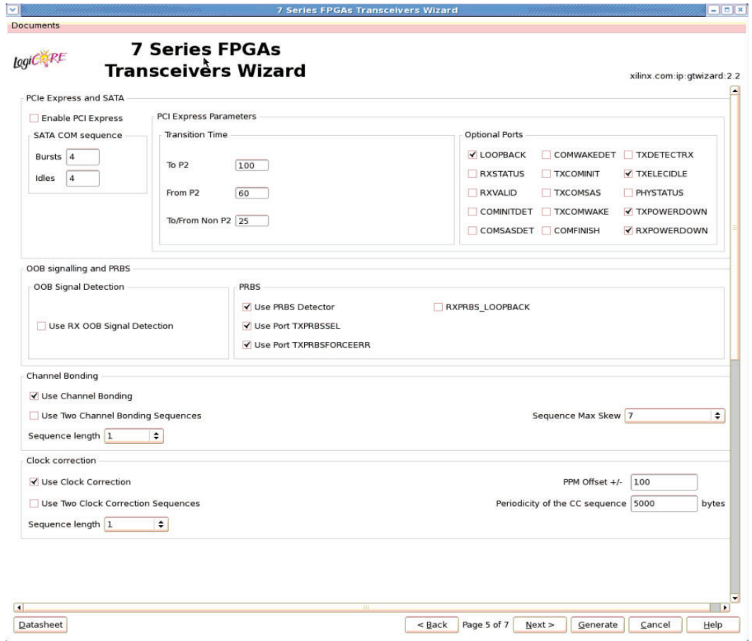
Figure 3-17: PCI Express, SATA, OOB, PRBS, Channel Bonding, and Clock Correction Selection—Page 5
