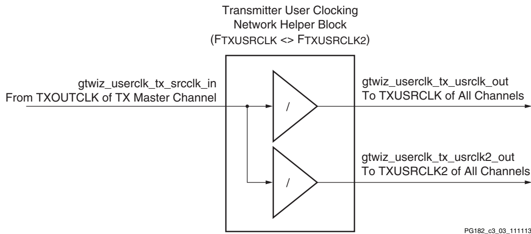
Figure 3-3: Transmitter User Clocking Network Helper Block (with Two BUFG_GT Primitives)
