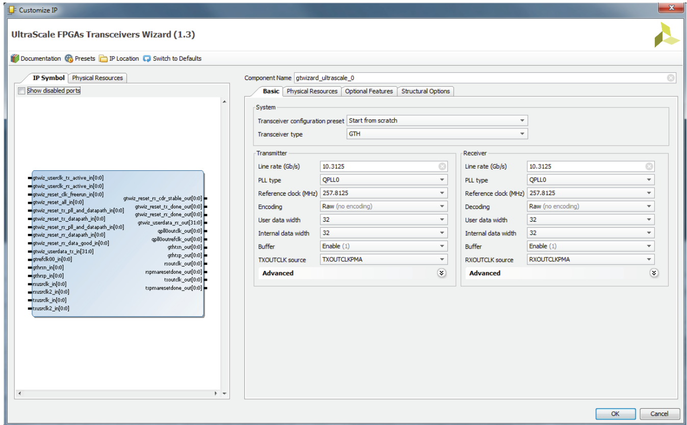
Figure 4-1: Basic Tab
