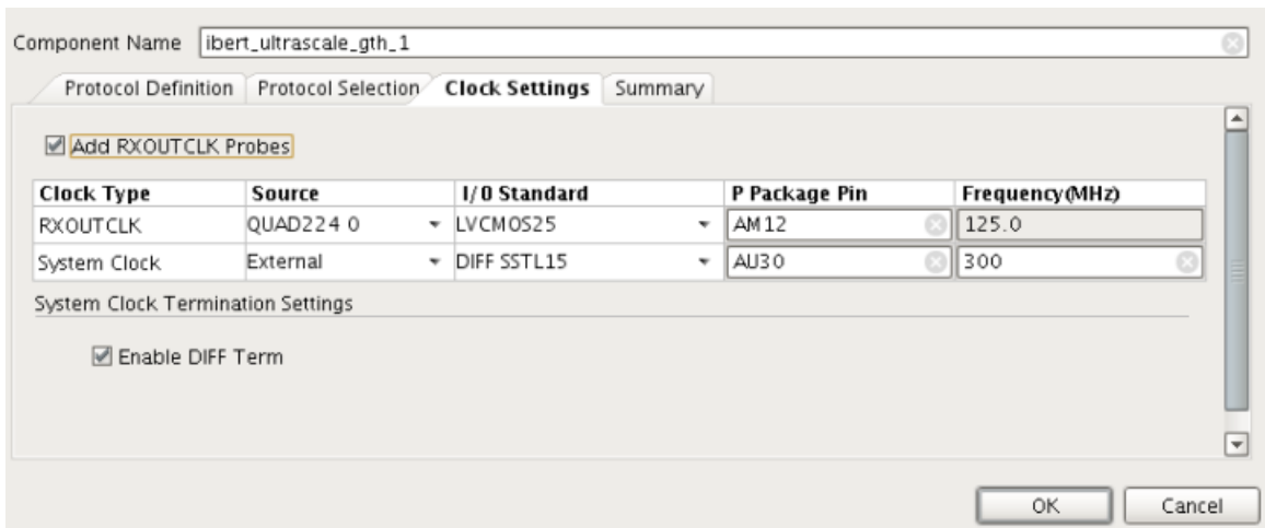
Figure 4-3: Vivado Customize IP Dialog Box – Clock Settings
