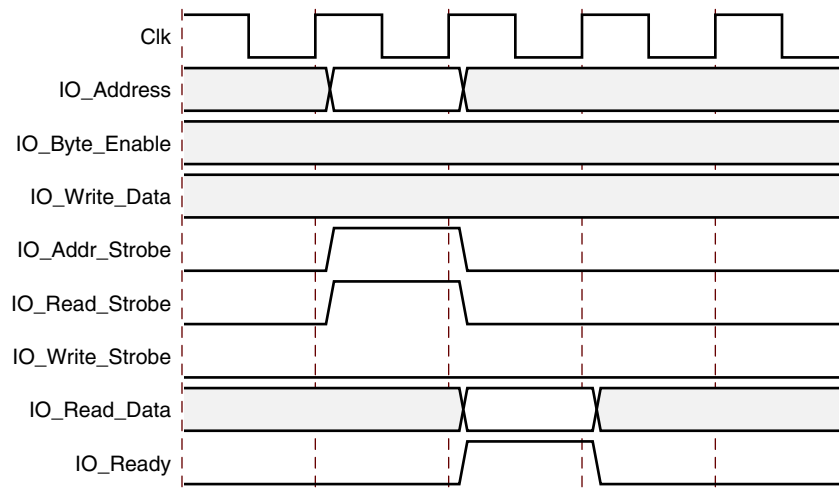
Figure 3-2: I/O Bus Read
