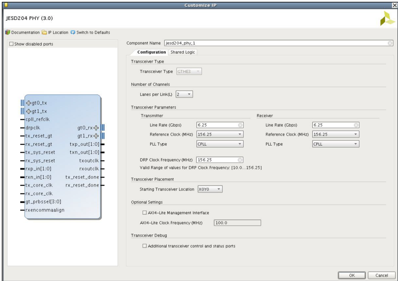
Figure 4-1: Configuration Tab
