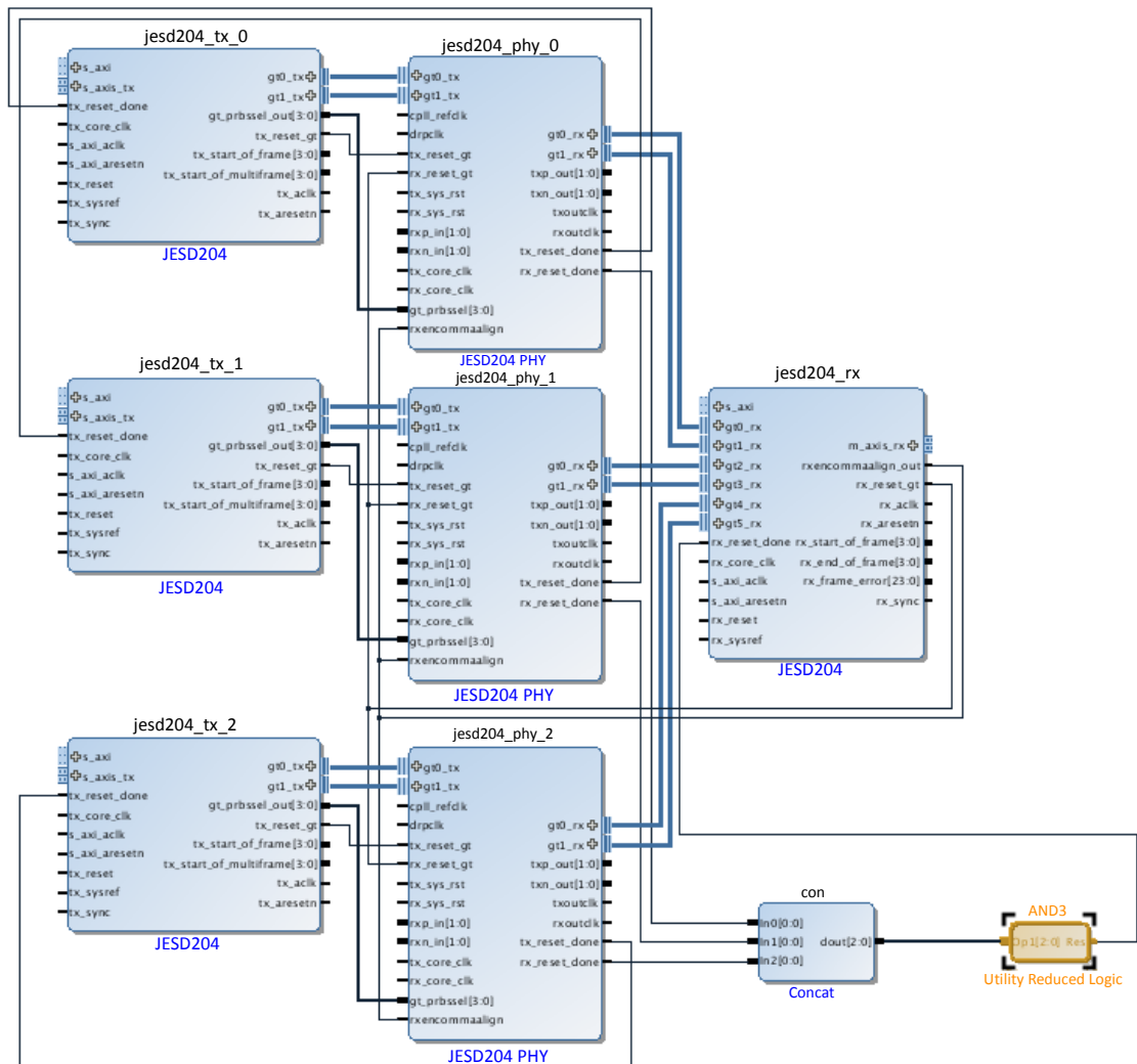
Figure 1-4: IP Integrator Example Design
