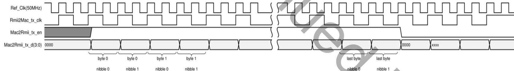
Figure 3-4: MII to RMII Transmit Transaction at 100 Mb/s
