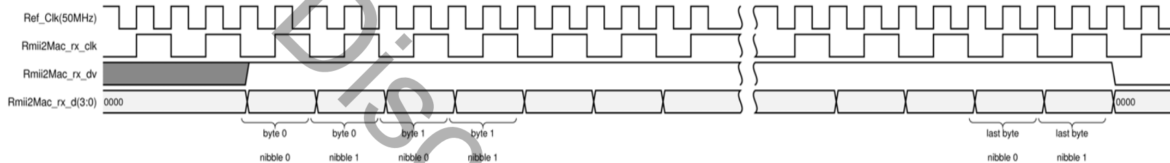
Figure 3-3: RMII to MII Receive Transaction at 100 Mb/s
