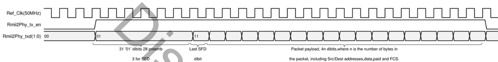
Figure 3-5: RMII to PHY Transmit Transaction at 100 Mb/s
