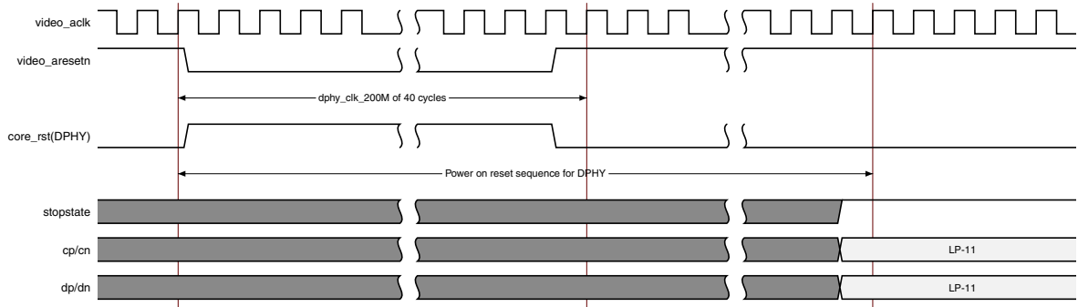
Figure 3-6: MIPI CSI-2 RX Reset
