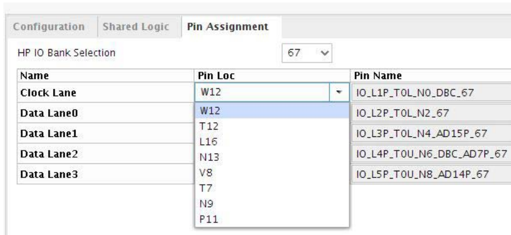
Figure 3-5: Subsystem Customization Screen - Pin Assignment
