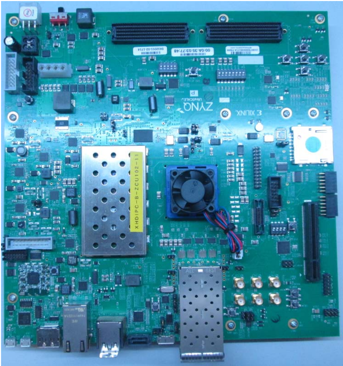
Figure 5-5: ZCU 102 Board
