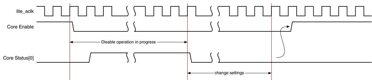
Figure 3-7: Core Programming Sequence
