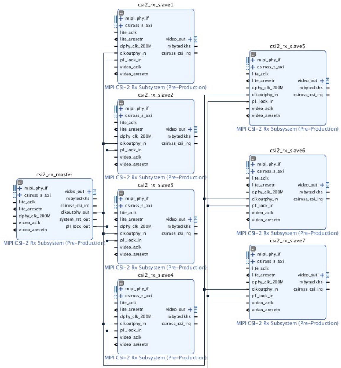
Figure 3-4: MIPI CSI-2 RX Subsystem Core Shared Logic Use Case for Single I/O Bank
