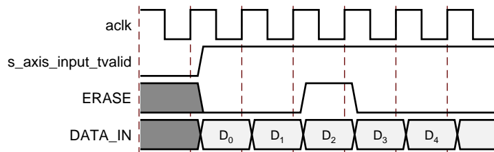
Figure 3-10: ERASE Timing
