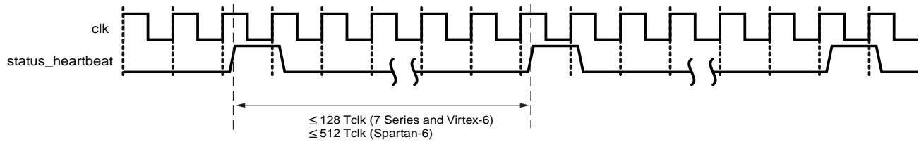
Figure 3-4: Status Interface Heartbeat Switching Characteristics
