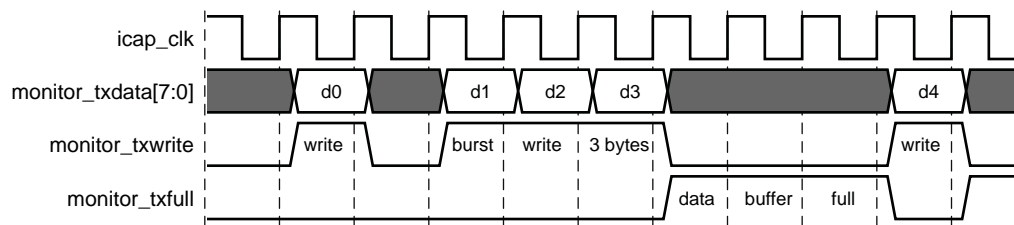
Figure 3-24: Monitor Interface Transmit Protocol
