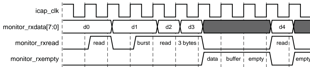
Figure 3-25: Monitor Interface Receive Protocol
