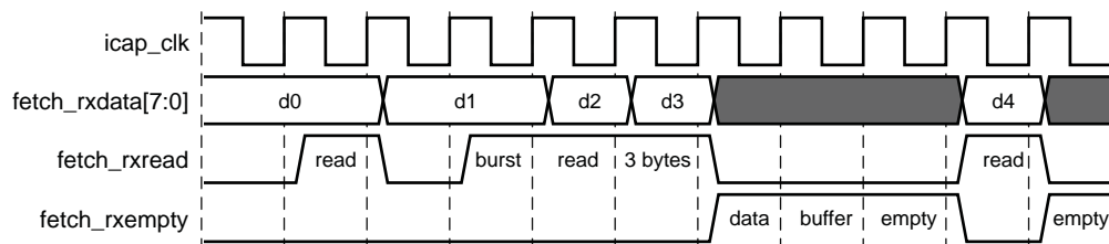
Figure 3-27: Fetch Interface Receive Protocol
