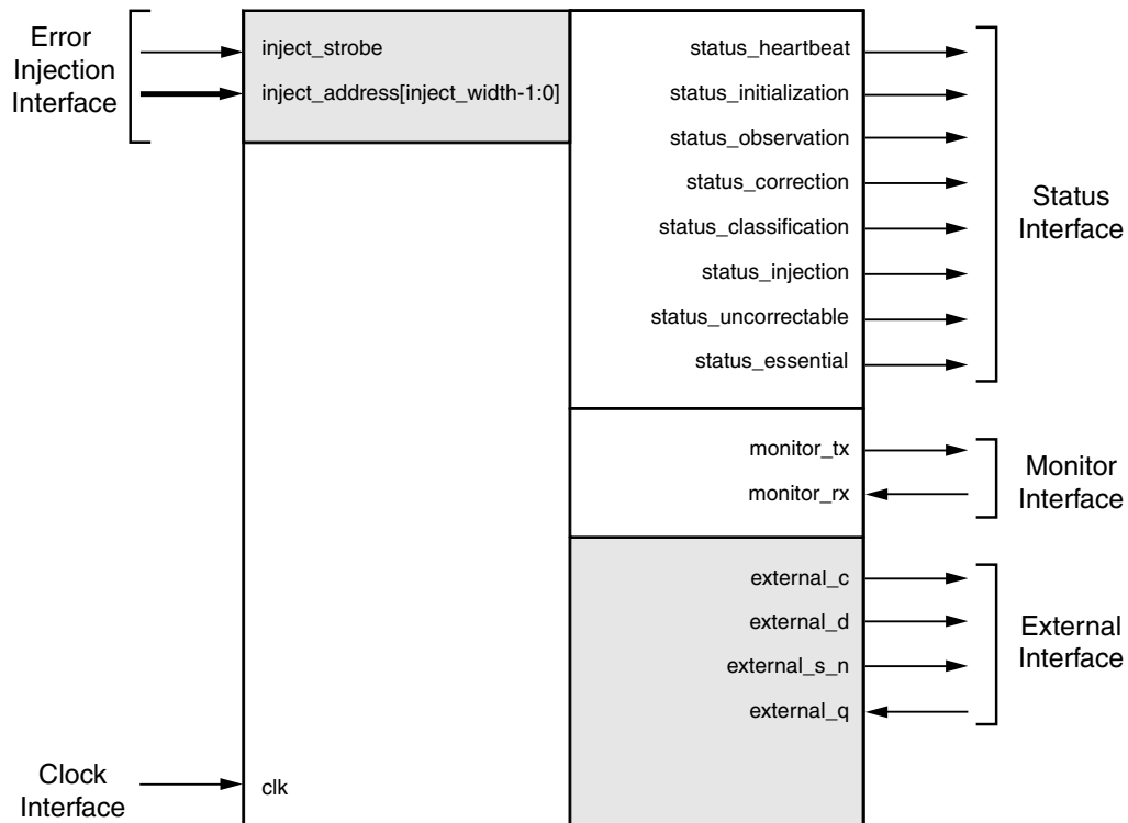
Figure 6-2: Example Design Ports
