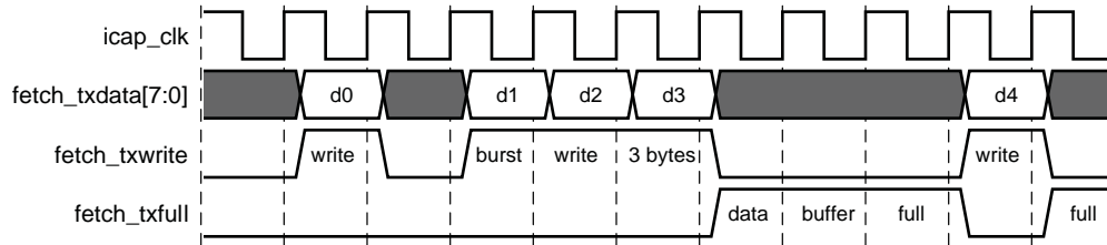
Figure 3-26: Fetch Interface Transmit Protocol
