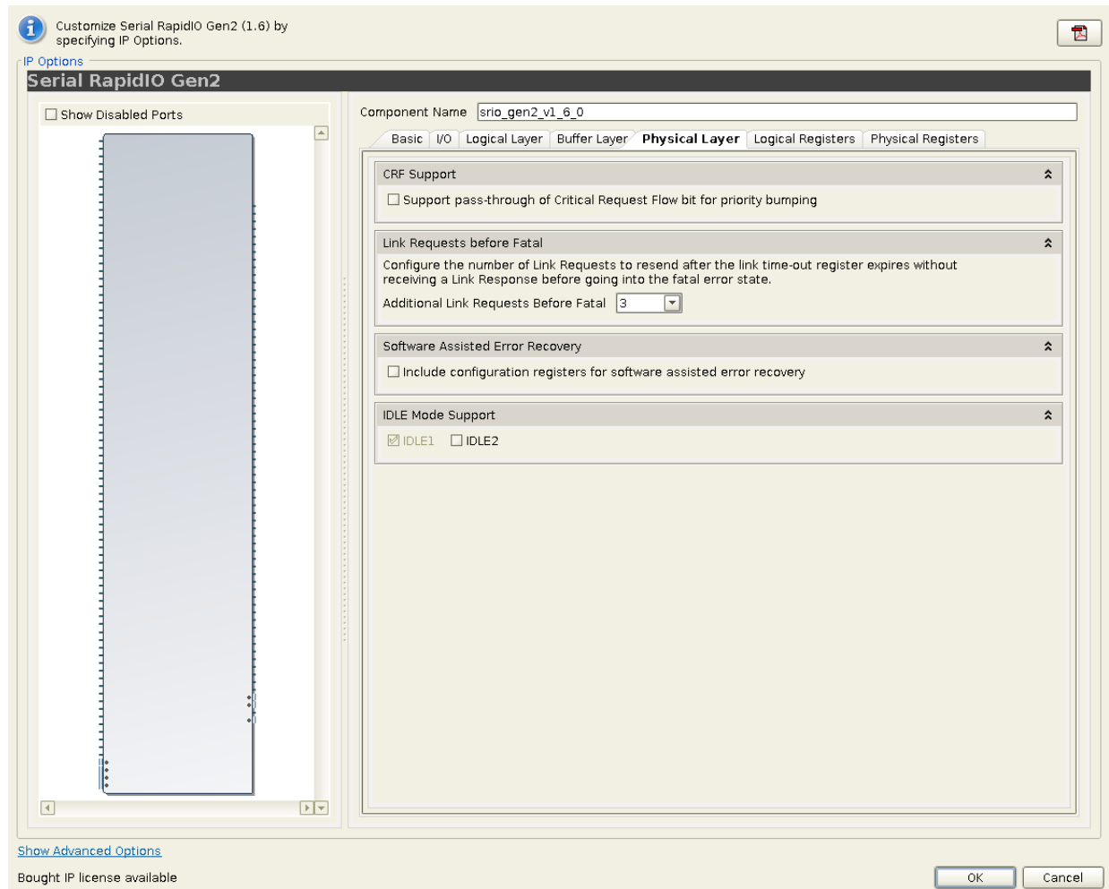
Figure 4-6: Advanced Mode: Physical Layer Tab
