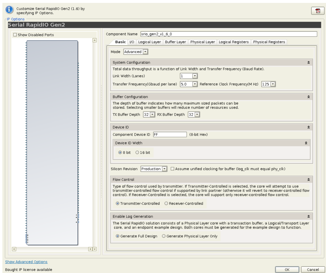
Figure 4-2: Advanced Mode: Basic Tab
