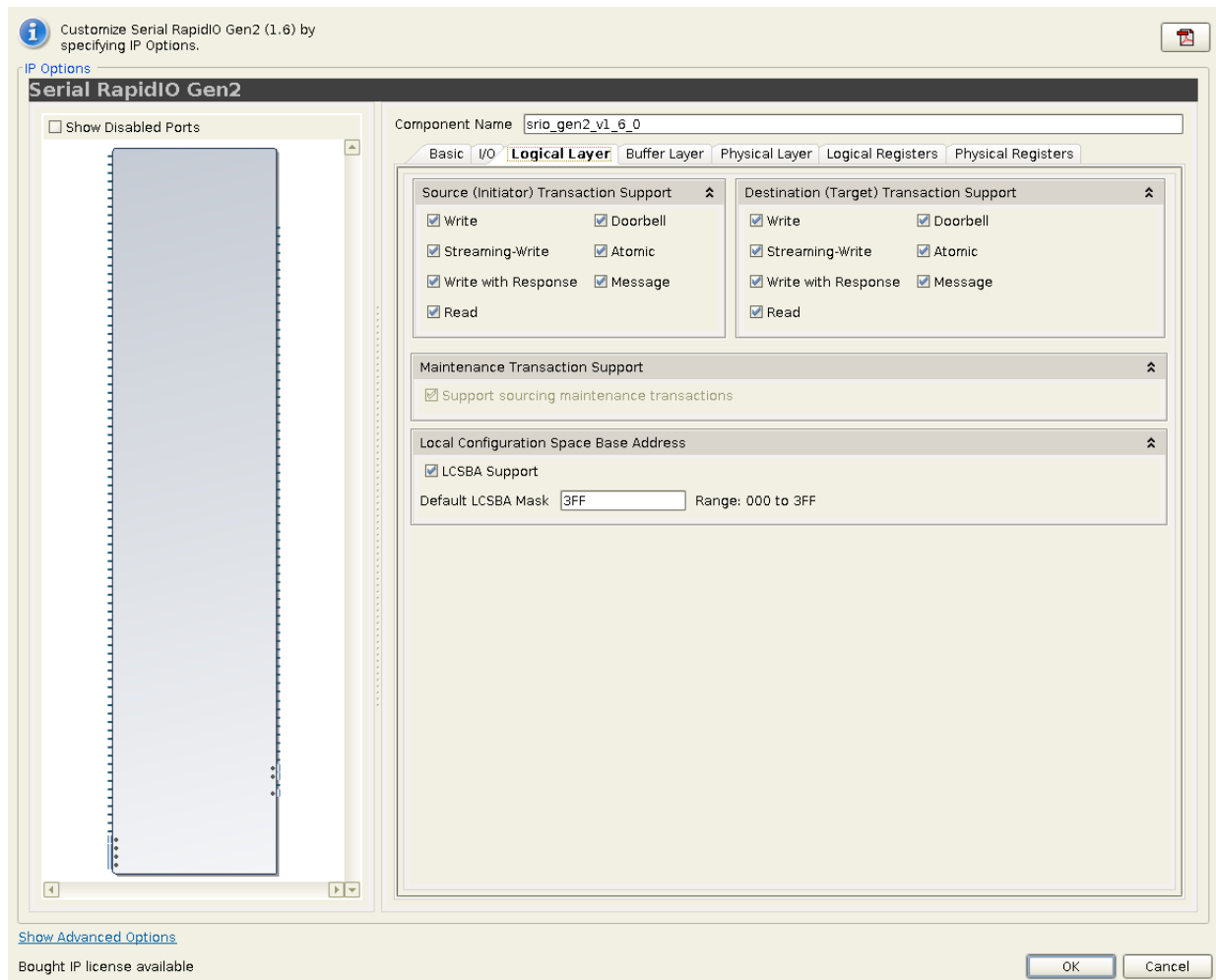
Figure 4-4: Advanced Mode: Logical Layer Tab
