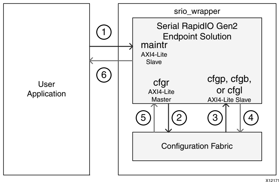
Figure 3-12: Local MAINTENANCE Transaction Flow
