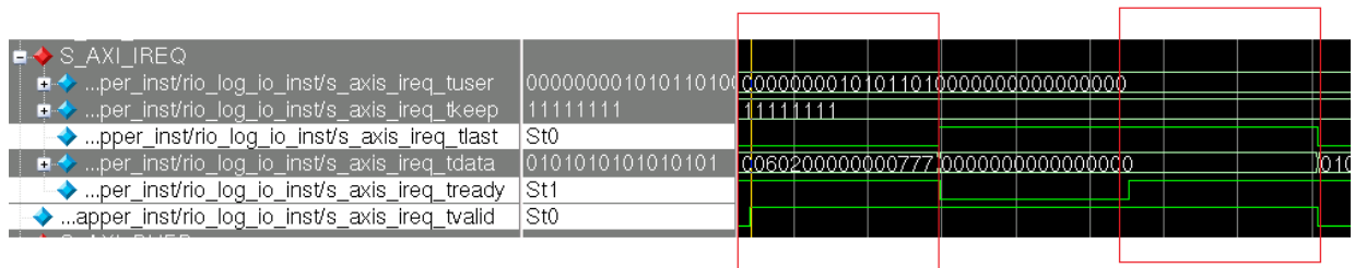
Figure C-7: SWRITE Packet Transmission on IREQ Interface
