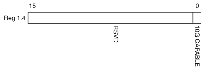
Figure 2-30: PCS Speed Ability Register
