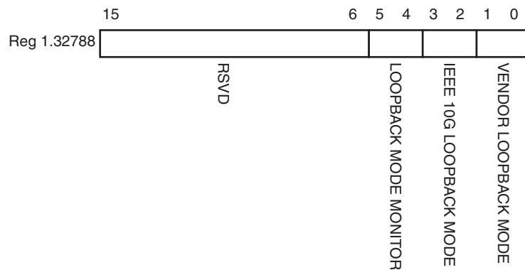
Figure 2-25: Vendor-Specific PMA Loopback Control Register
