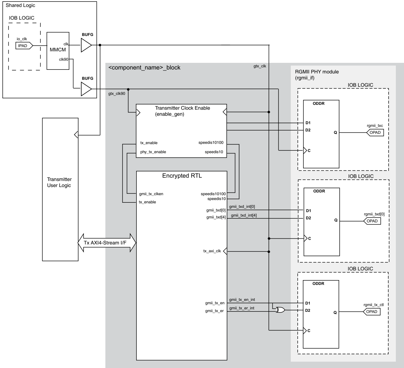
Figure 3-68: Tri-Speed RGMII Transmitter Logic and Clock Logic for 7 Series Devices Using HR I/O
