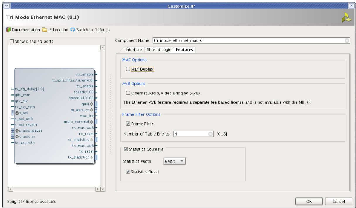
Figure 4-3: Vivado Customize IP IDE – Features Tab
