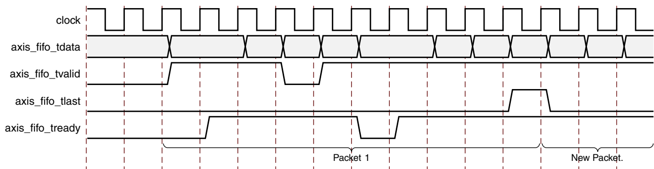
Figure 8-2: Frame Transfer across AXI4-Stream Interface
