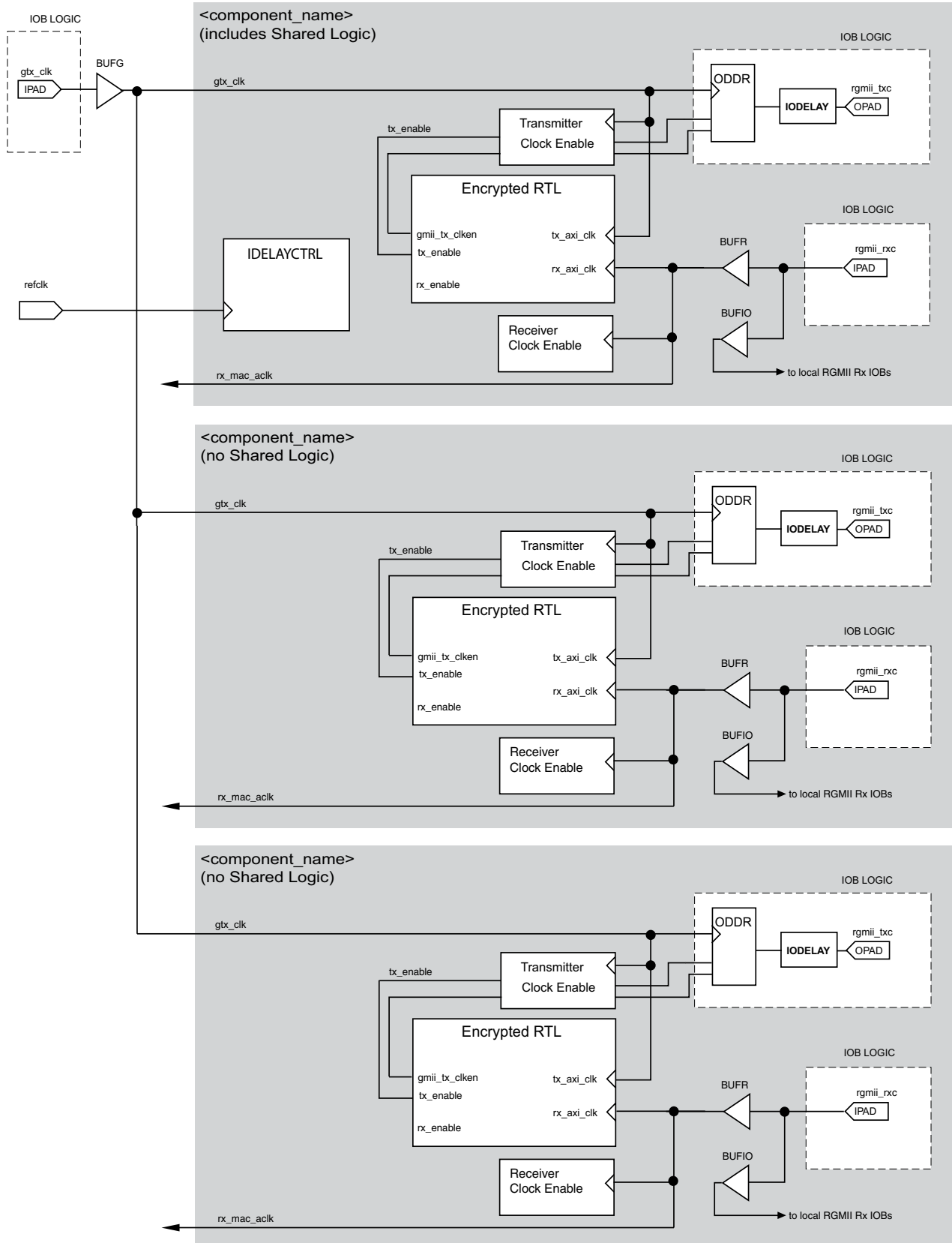
Figure 3-70: Clock Resource Sharing for Tri-Speed RGMII in 7 Series Using HP I/O
