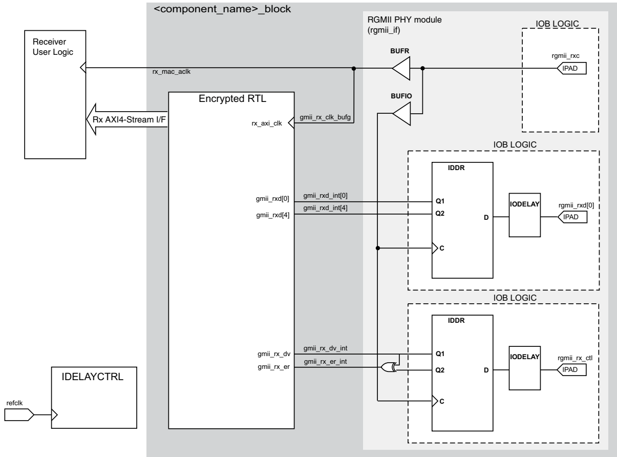
Figure 3-61: 1 Gb/s RGMII Receiver Logic and Clock Logic for 7 Series Devices
