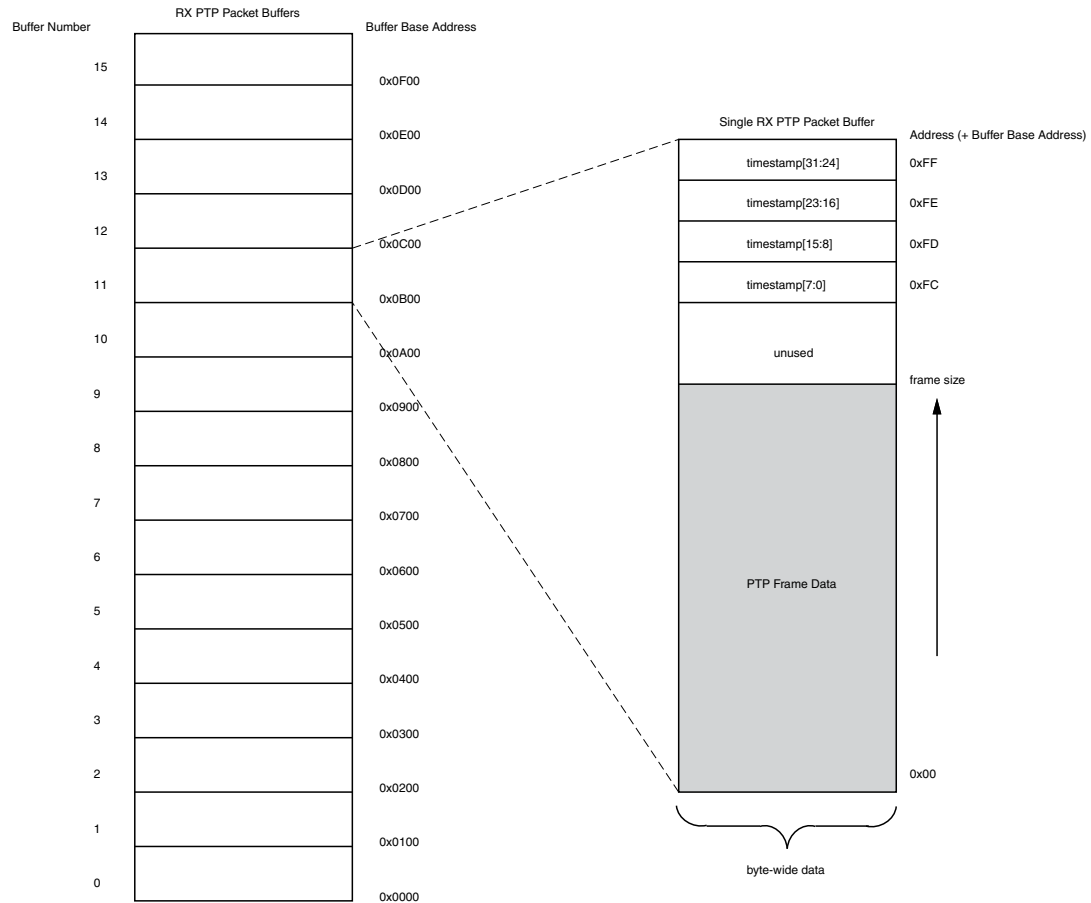
Figure 3-47: RX PTP Packet Buffer
