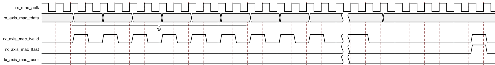
Figure 3-13: Normal Frame Reception at 10/100 Mb/s
