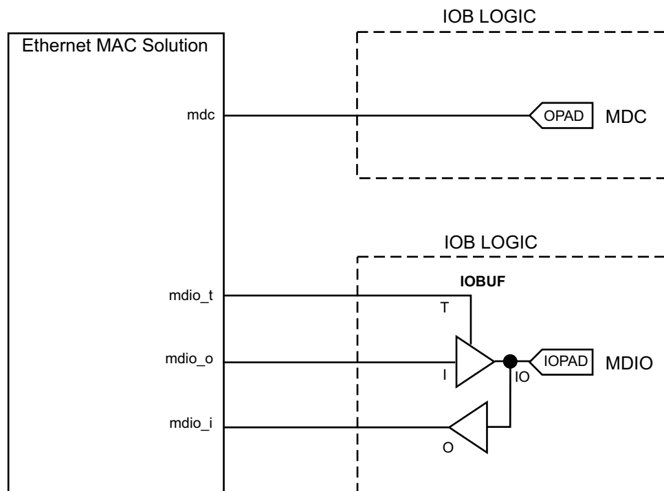
Figure 3-53: External MDIO Interface
