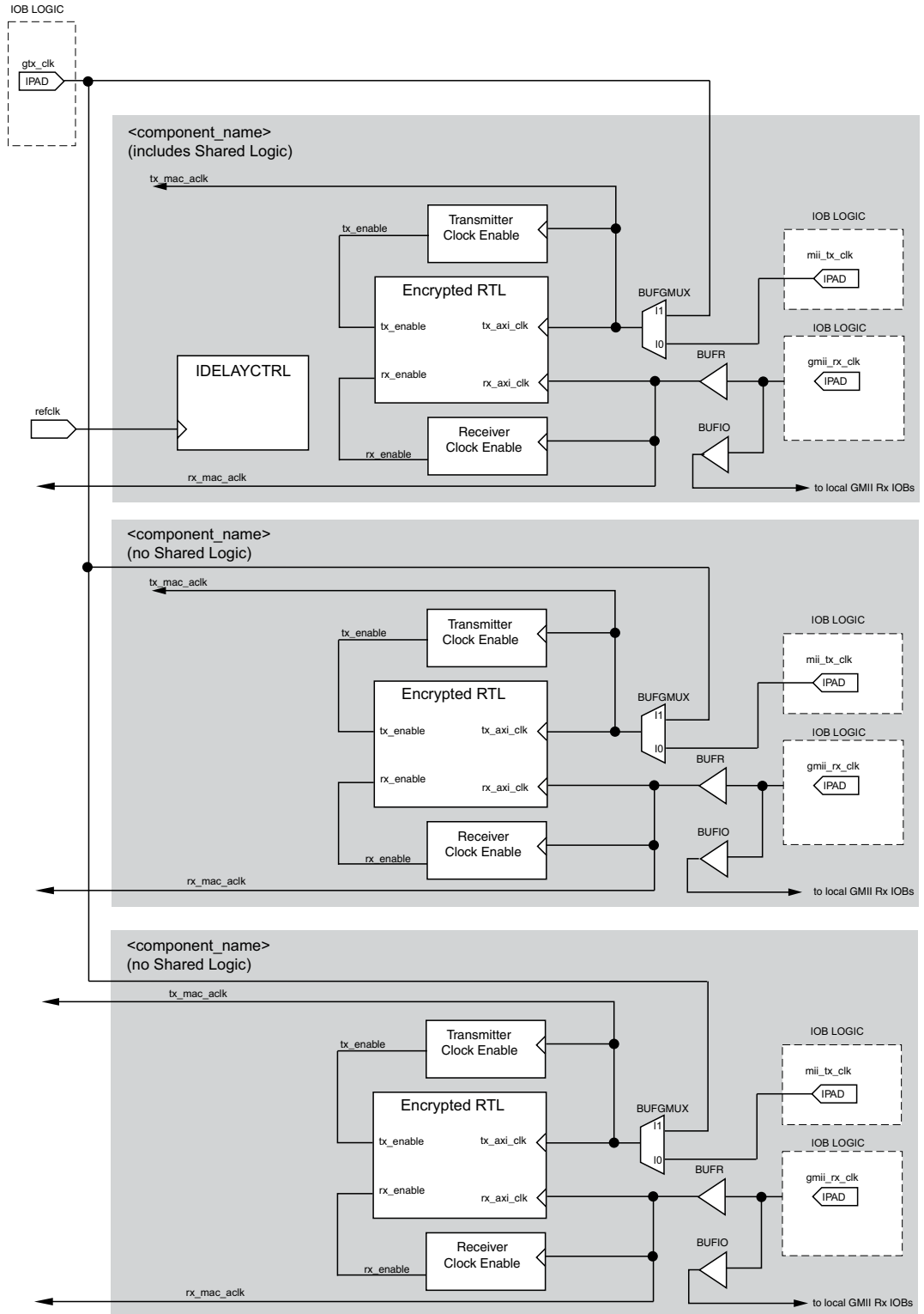
Figure 3-66: Clock Resource Sharing for Tri-Speed GMII in 7 Series Devices
