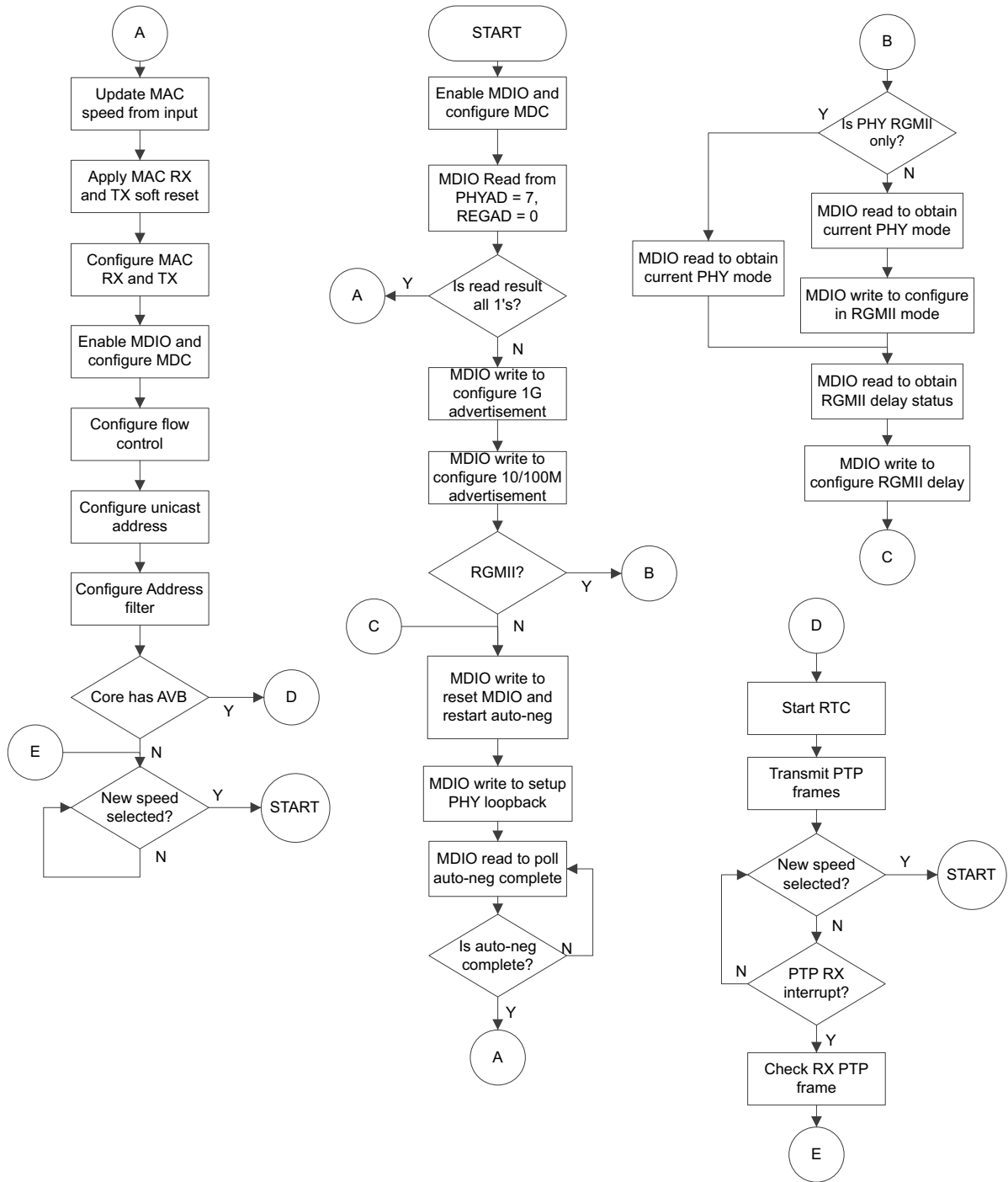
Figure 8-5: State Machine Flow Diagram
