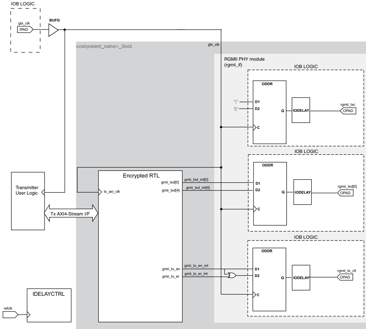
Figure 3-59: 1 Gb/s RGMII Transmitter Logic and Clock Logic for 7 Series Using HP I/O
