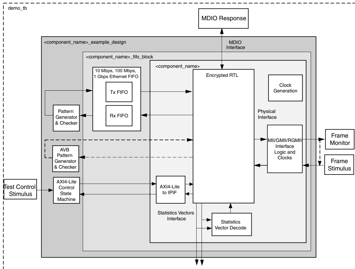
Figure 9-1: Demonstration Test Bench
