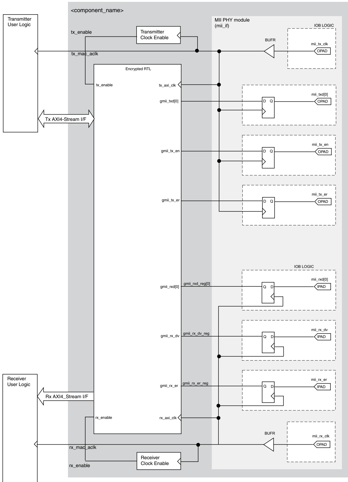
Figure 3-55: MII Transmitter, Receiver and Clock Logic For All Devices
