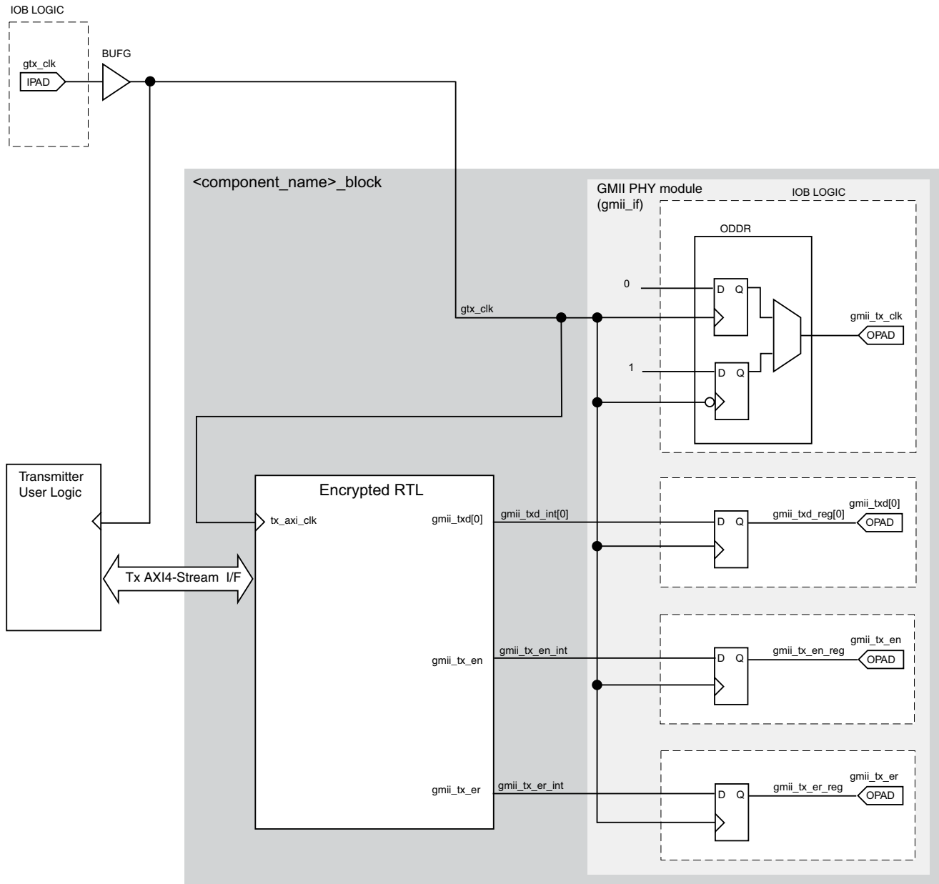
Figure 3-56: 1 Gb/s GMII Transmitter Logic and Clock Logic
