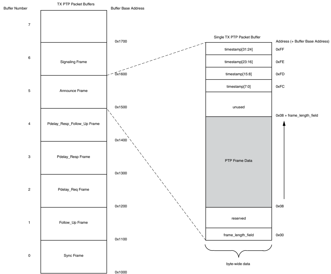
Figure 3-46: TX PTP Packet Buffer Structure
