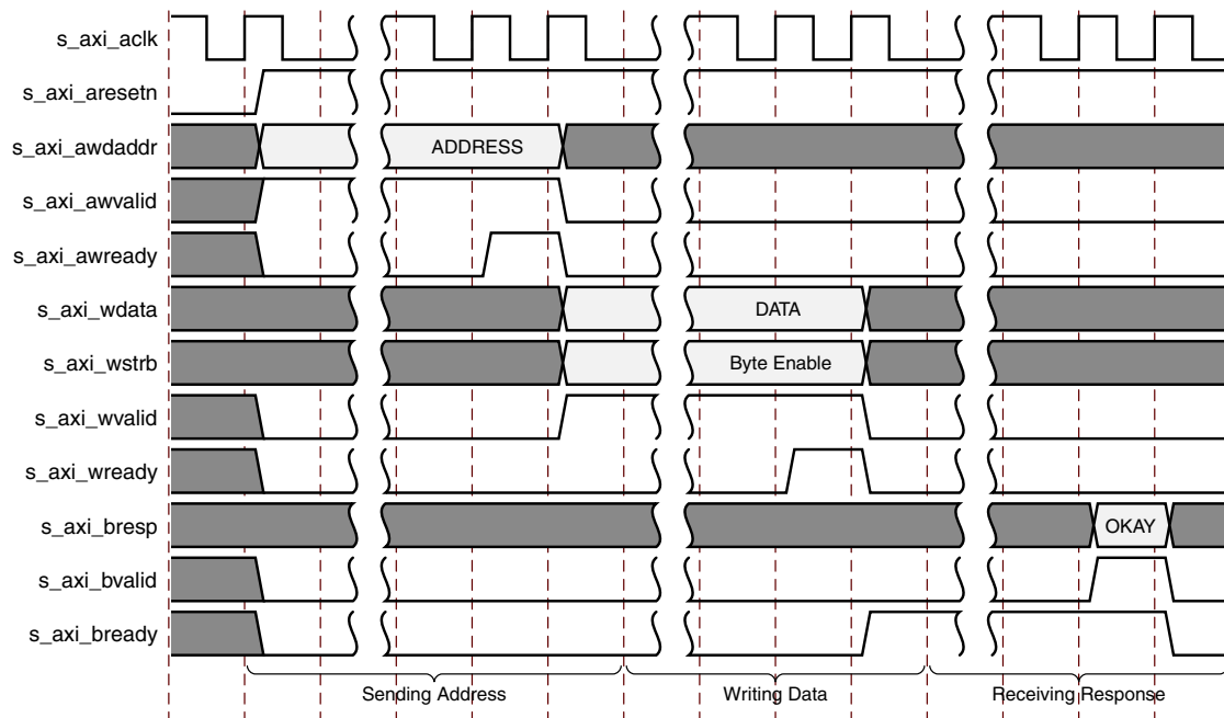
Figure 3-48: Management Register Write Timing
