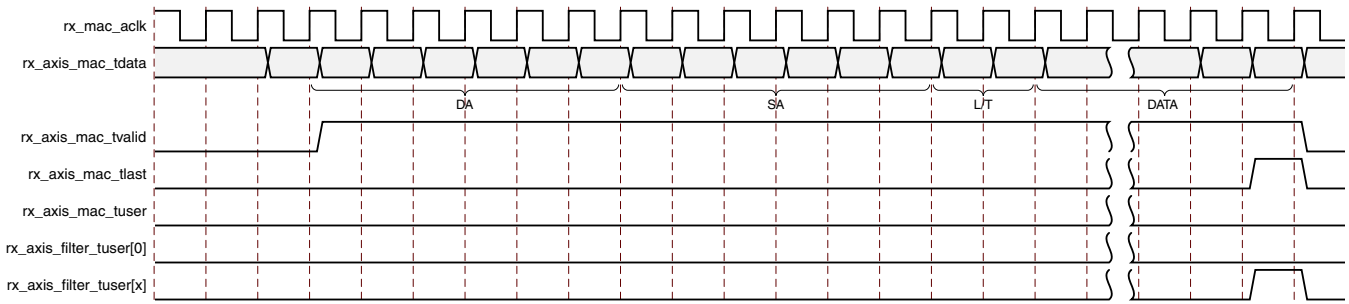
Figure 3-36: Received Frame with a Match on Filter 0
