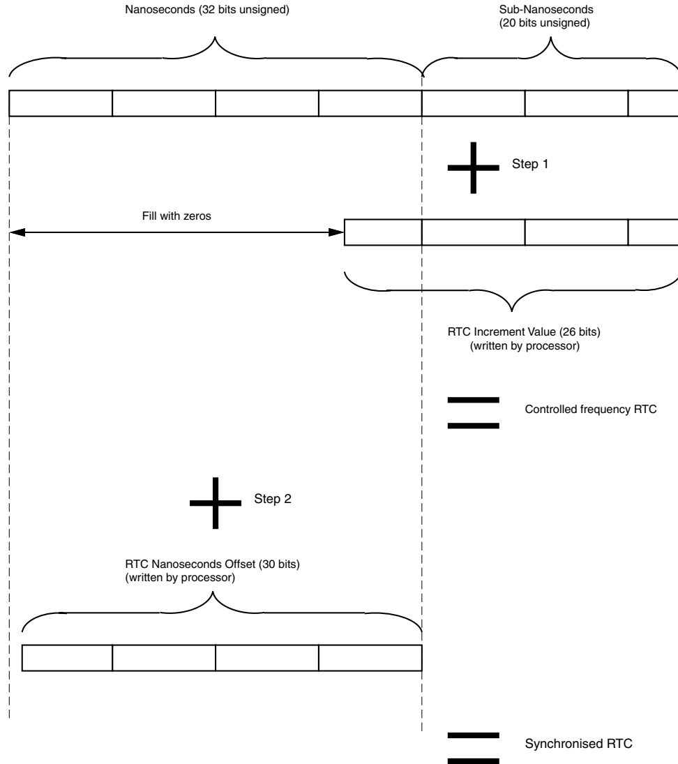
Figure 3-44: Increment of Sub-Nanoseconds and Nanoseconds Field
