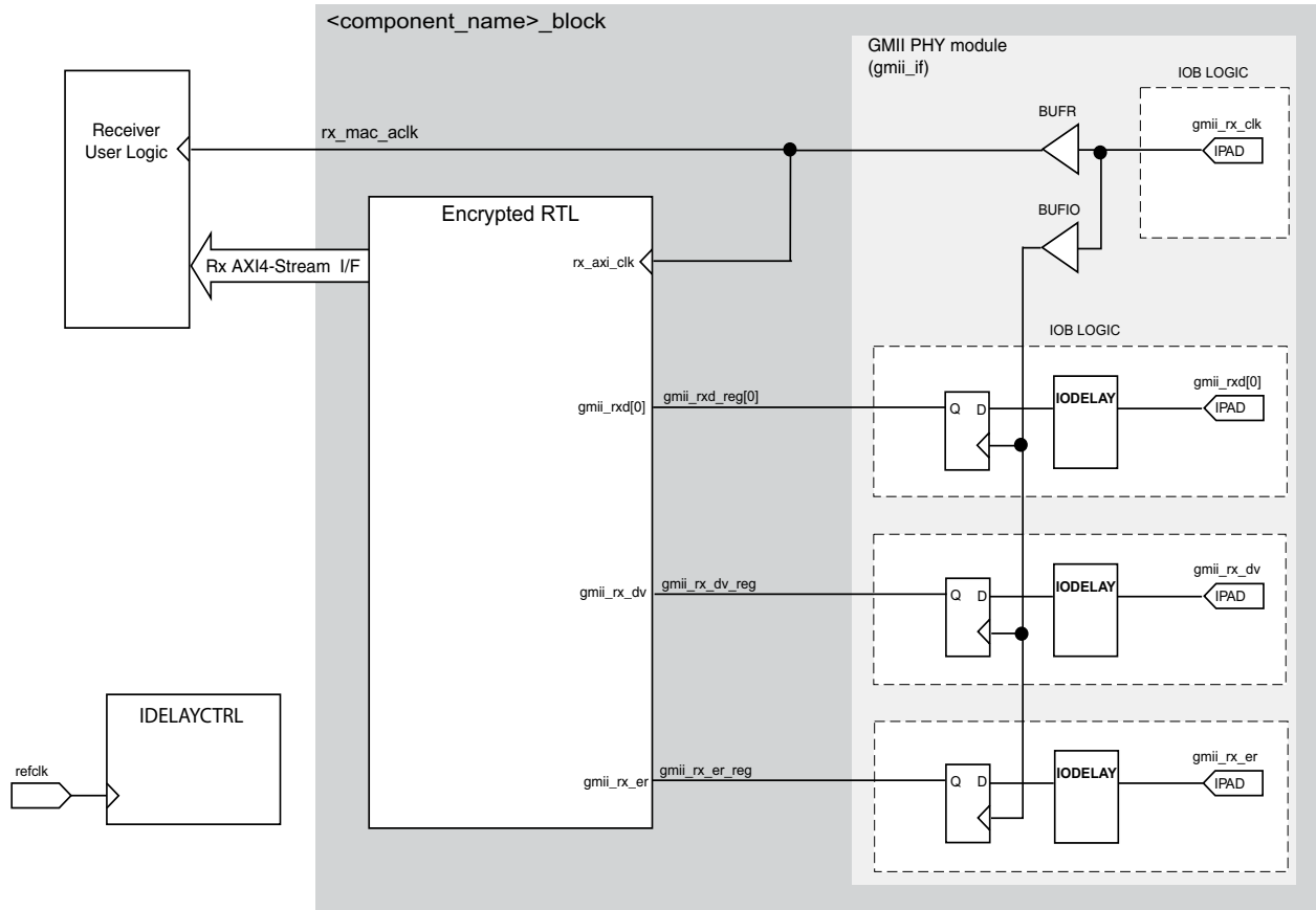
Figure 3-57: 1 Gb/s GMII Receiver Logic and Clock Logic for 7 Series Devices
