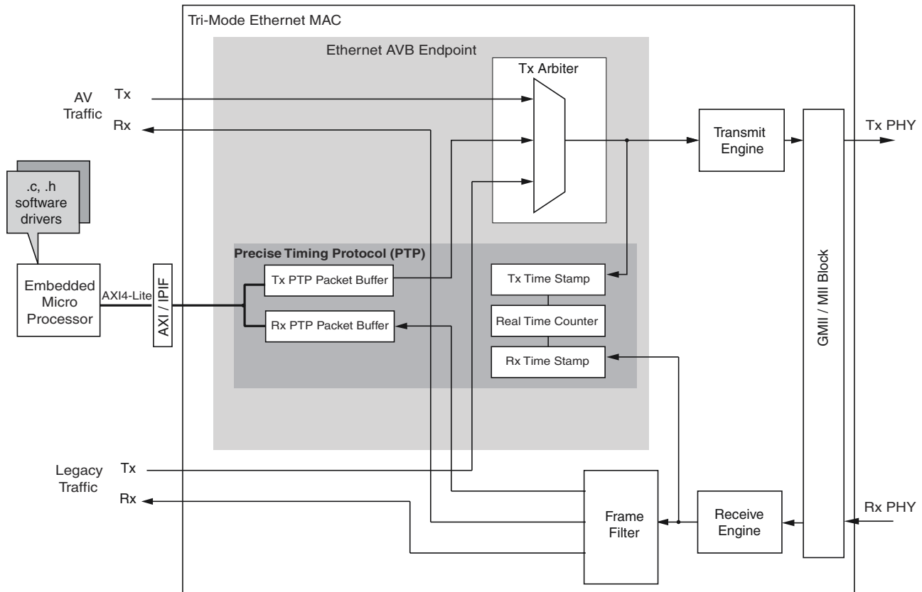
Figure 3-40: Ethernet AVB Endpoint Data Path
