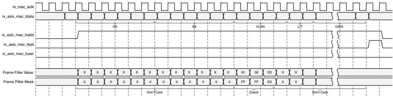
Figure 3-39: Filtering of VLAN Frames with VLAN Priority of 7
