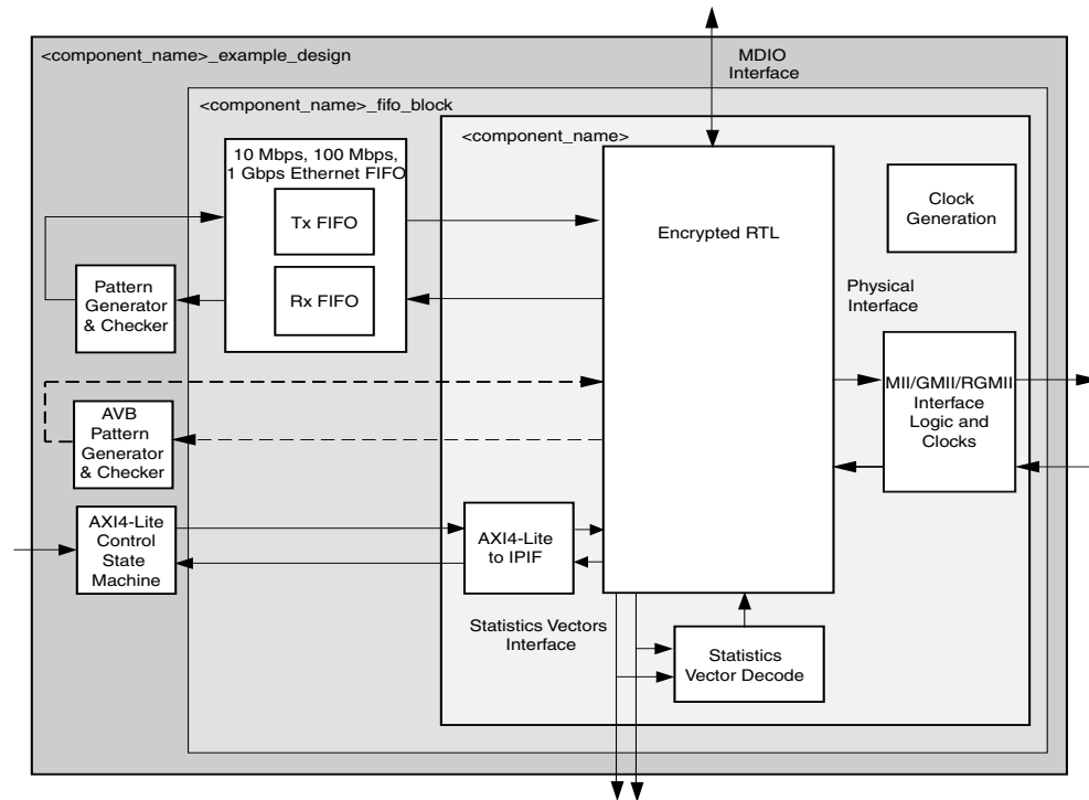
Figure 8-1: HDL Example Design
