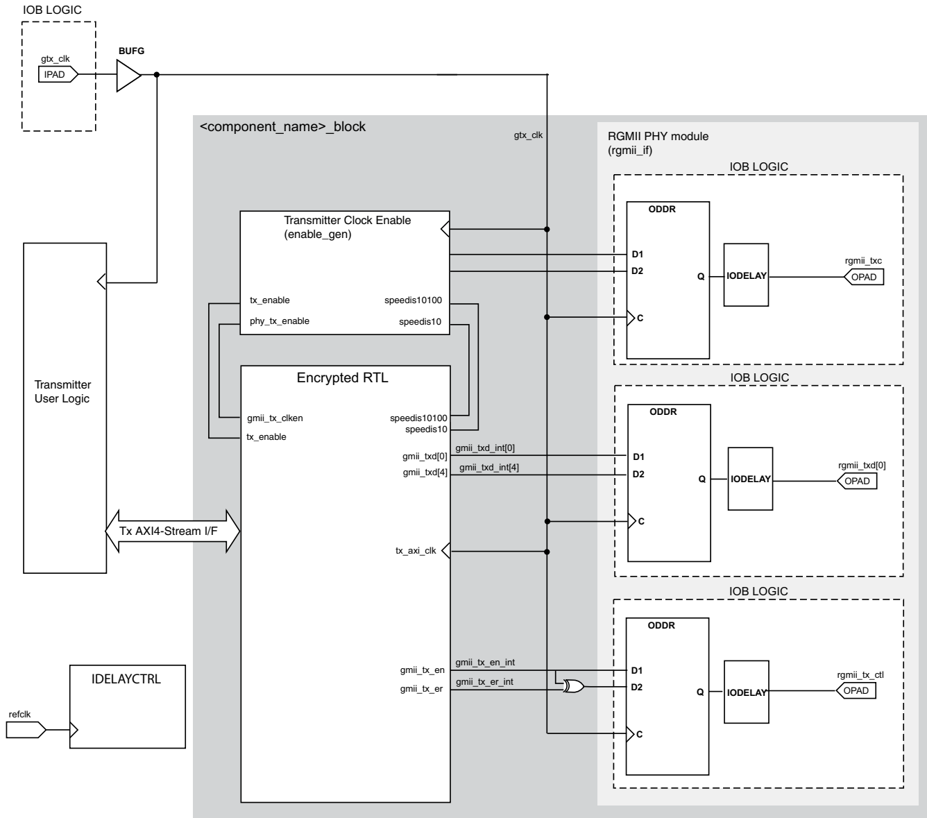
Figure 3-67: Tri-Speed RGMII Transmitter Logic and Clock Logic for 7 Series Devices
