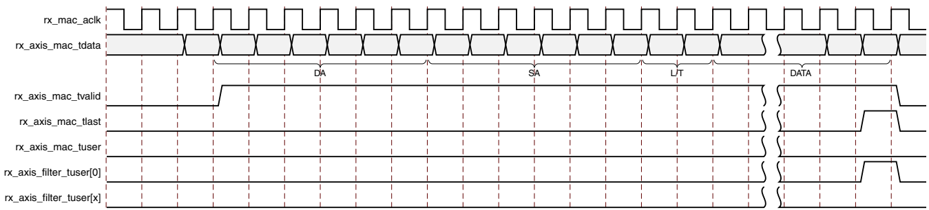
Figure 3-37: Received Frame with No Match on Configurable Frame Filters
