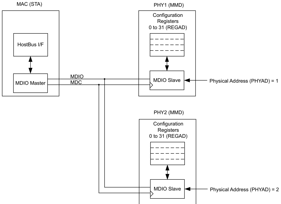
Figure 3-50: A Typical MDIO-Managed System
