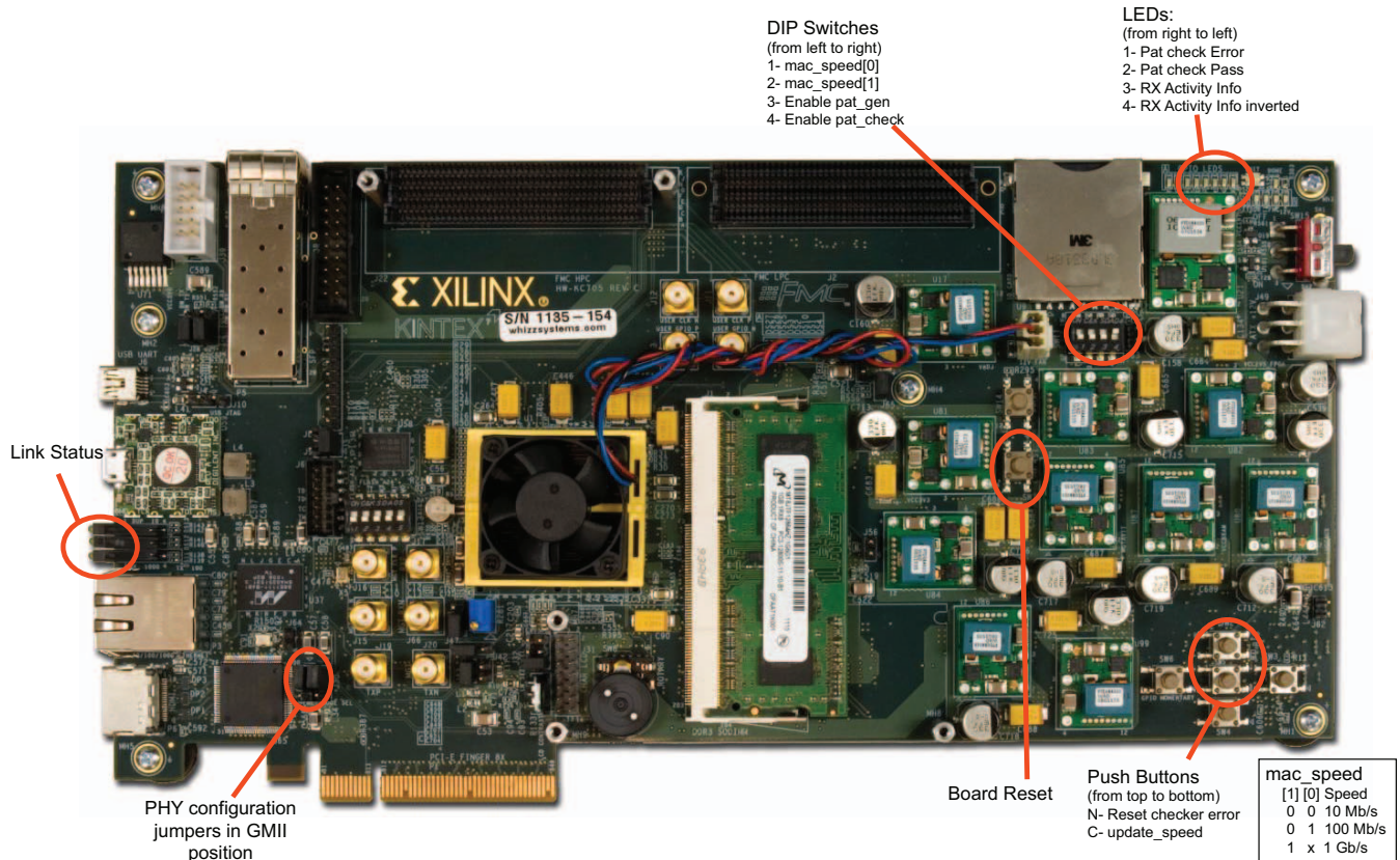
Figure 8-6: KC705 Board Connectivity
