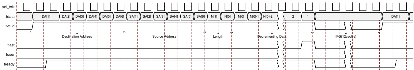
Figure 8-4: Pattern Generator Frame Structure
