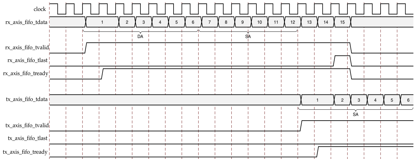
Figure 8-3: Modification of Frame Data by Address Swap Module
