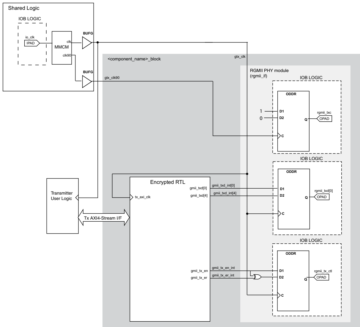
Figure 3-60: 1 Gb/s RGMII Transmitter Logic and Clock Logic for 7 Series Using HR I/O
