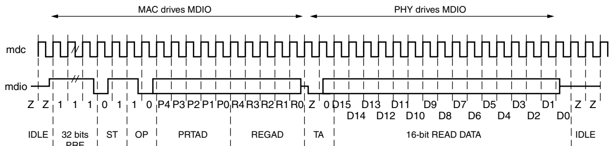
Figure 3-52: MDIO Read Transaction
