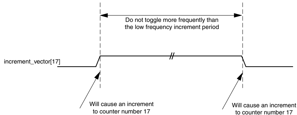
Figure 3-35: Increment Vector Timing Diagram
