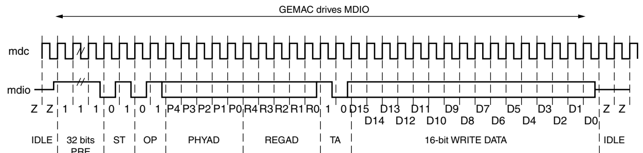
Figure 3-51: MDIO Write Transaction
