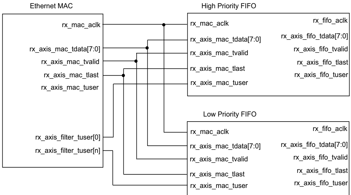
Figure 3-38: Priority FIFO Connections
