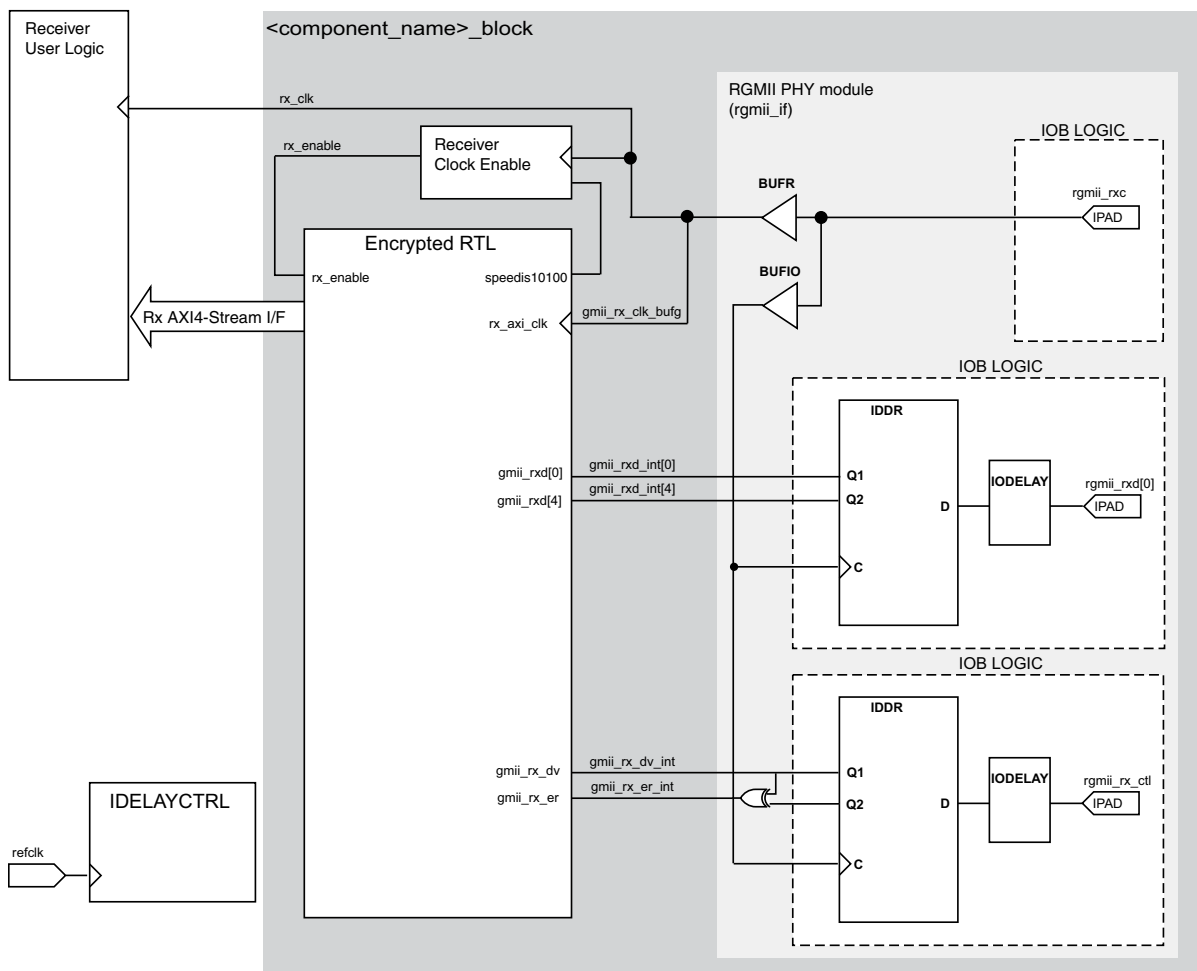
Figure 3-69: Tri-Speed RGMII Receiver Logic and Clock Logic for 7 Series Devices
