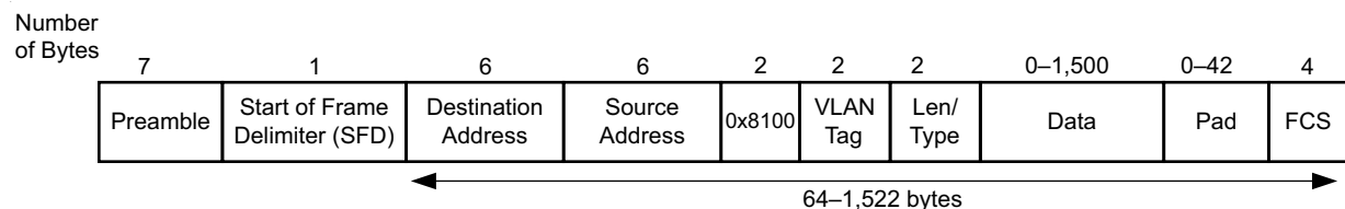
Figure 3-11: Ethernet VLAN Frame Format
