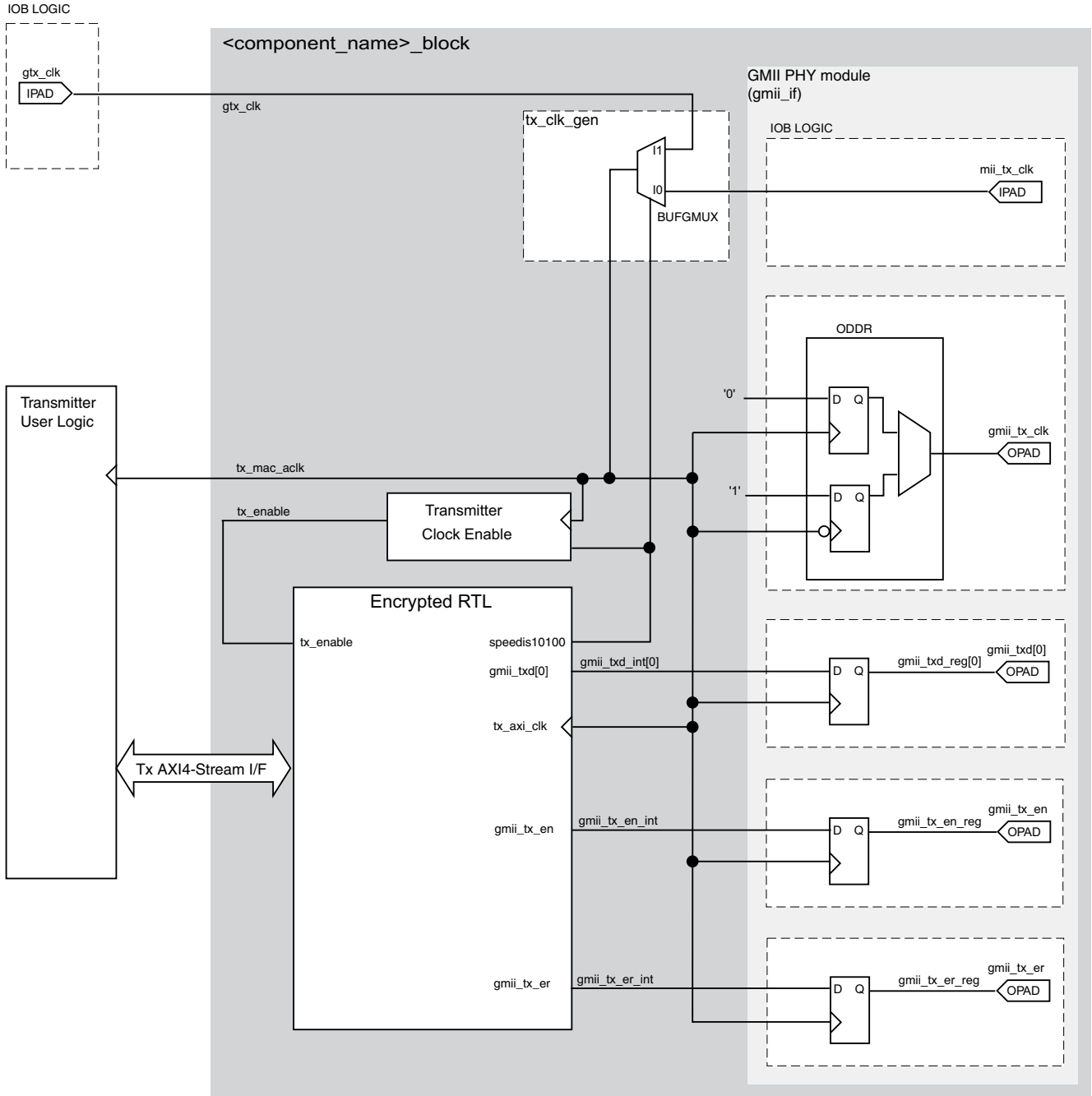
Figure 3-64: Tri-Speed GMII Transmitter Logic and Clock Logic
