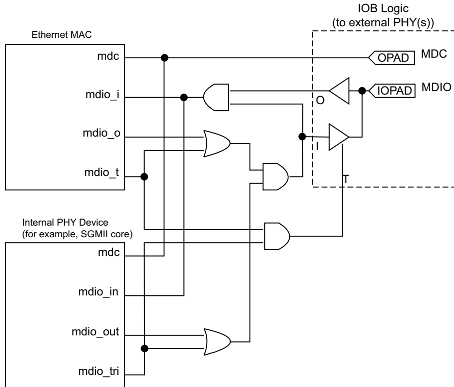
Figure 3-54: Internal and External MDIO Interfaces
