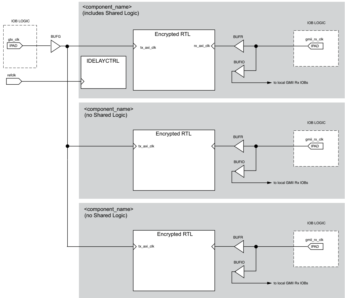
Figure 3-58: Clock Resource Sharing for 1 Gb/s GMII in 7 Series Devices
