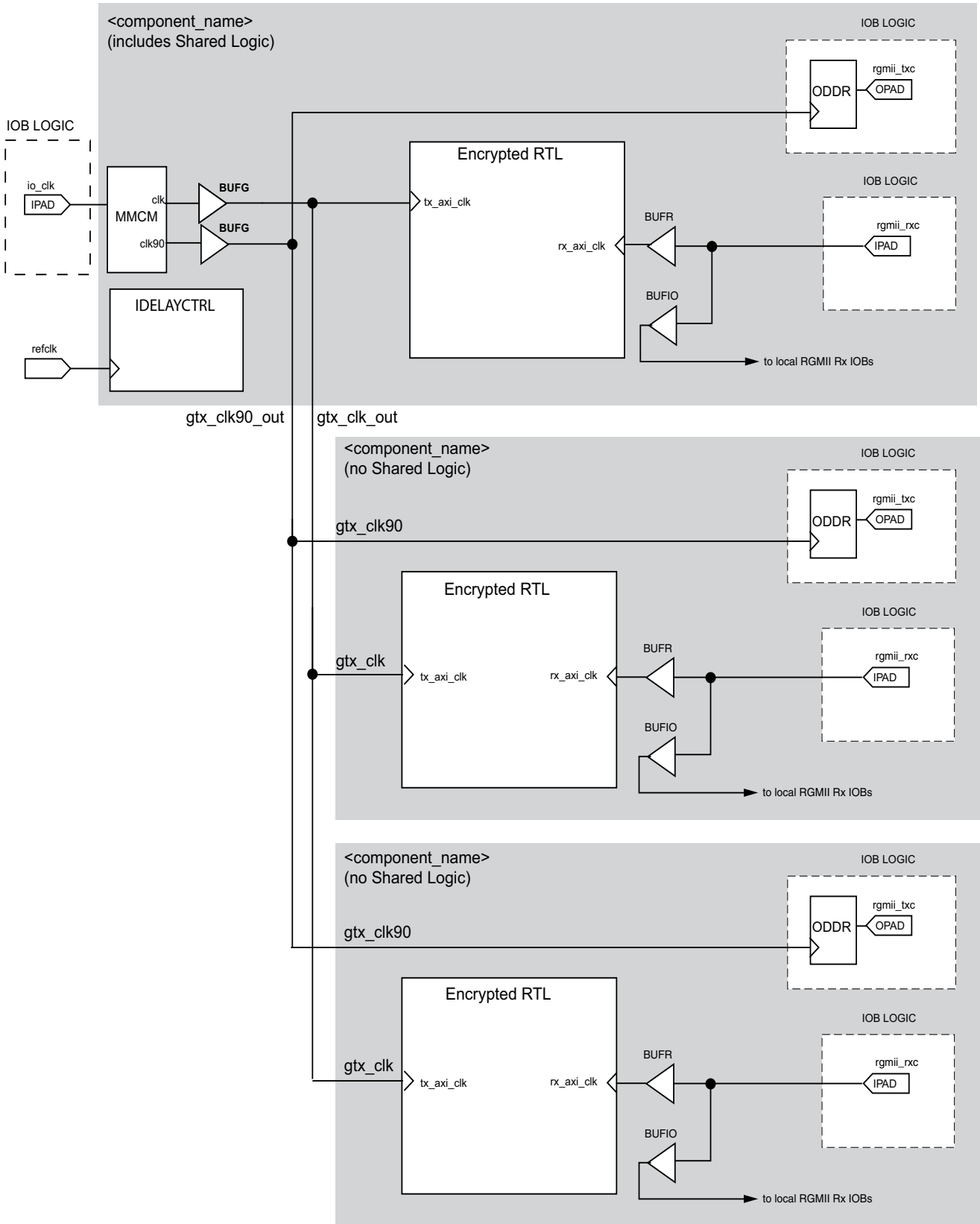
Figure 3-63: Clock Resource Sharing for 1 Gb/s RGMII in 7 Series Using HR I/O
