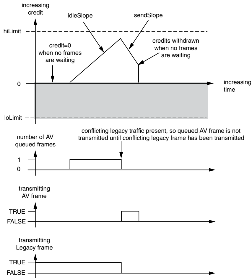
Figure 3-42: Credit-Based Shaper Operation
