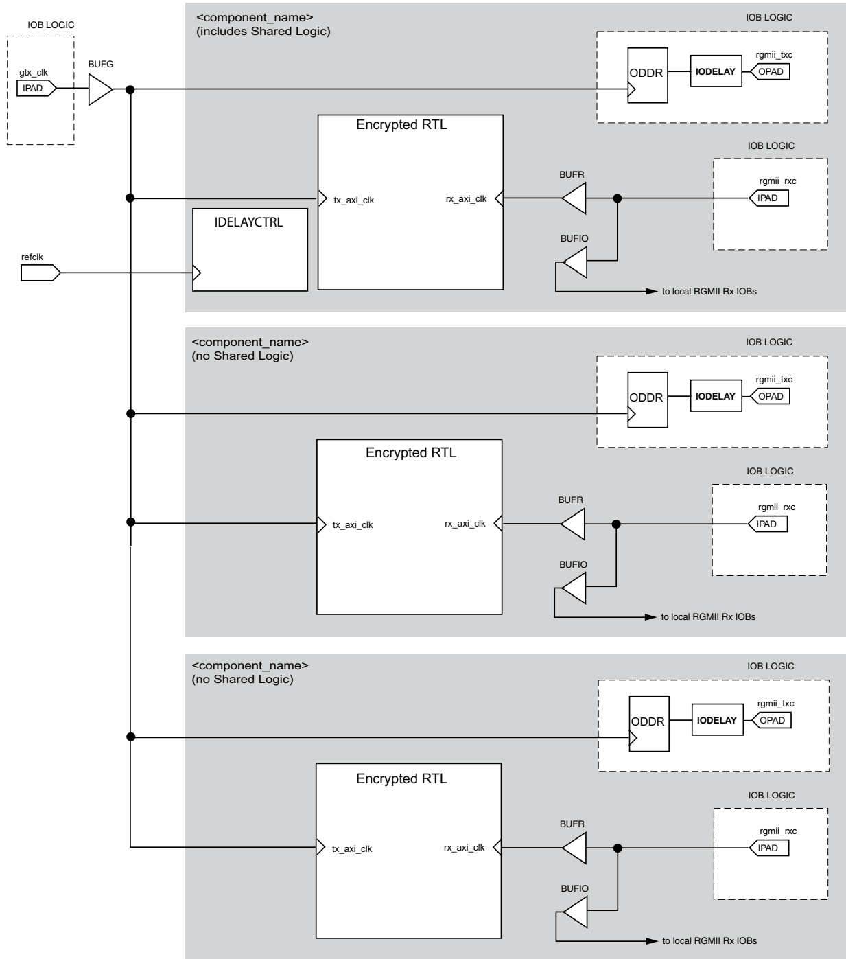
Figure 3-62: Clock Resource Sharing for 1 Gb/s RGMII in 7 Series Using HP I/O
