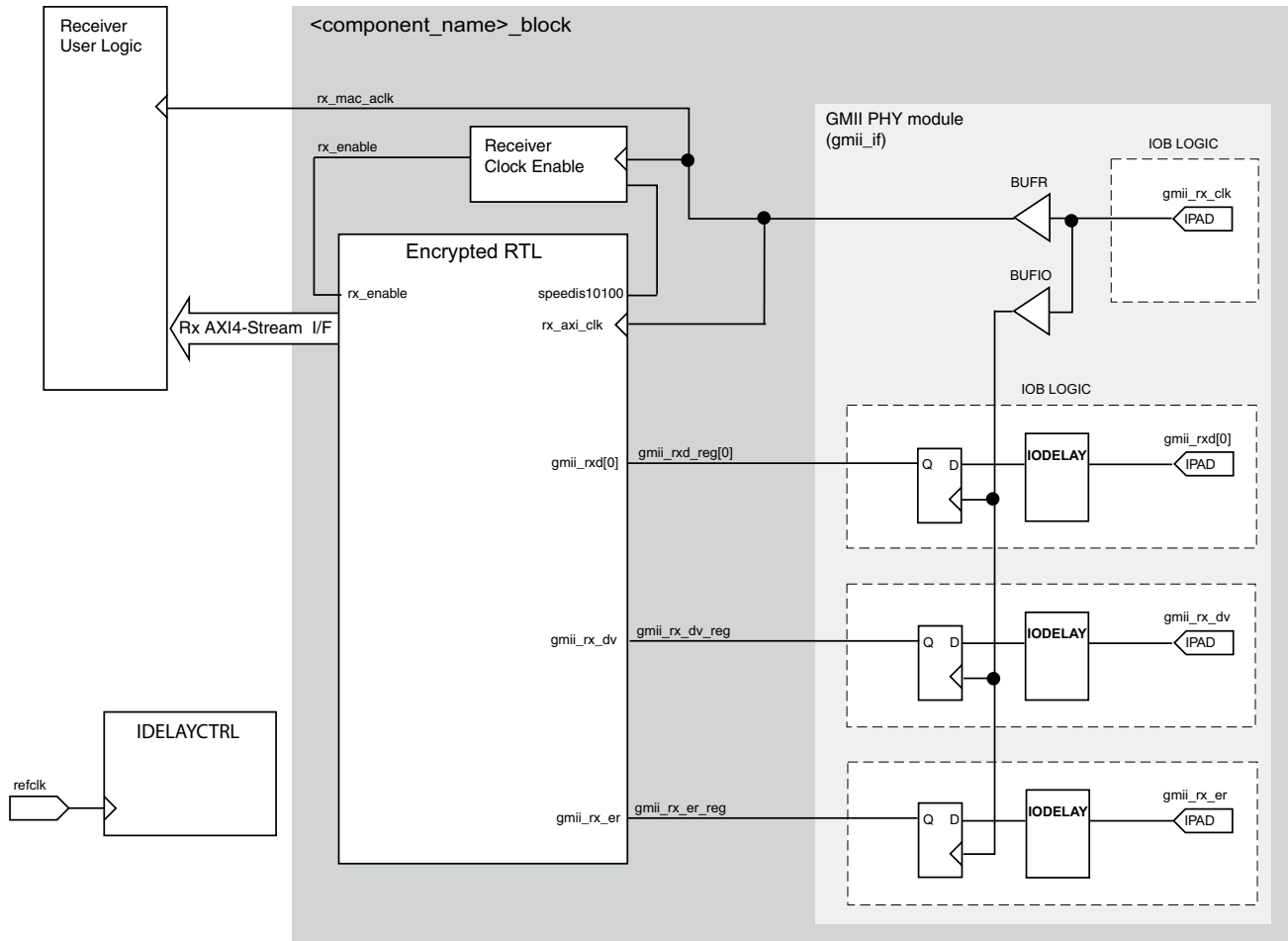
Figure 3-65: Tri-Speed GMII Receiver Logic and Clock Logic for 7 Series Devices
