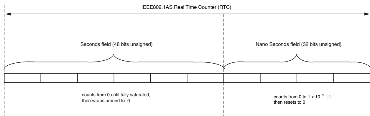
Figure 3-43: Real-Time Clock (RTC)
