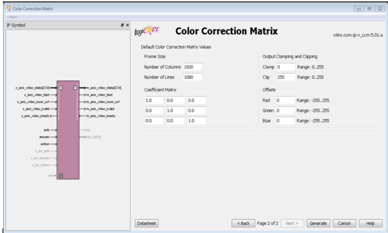
Figure 8-2: Screen 2
