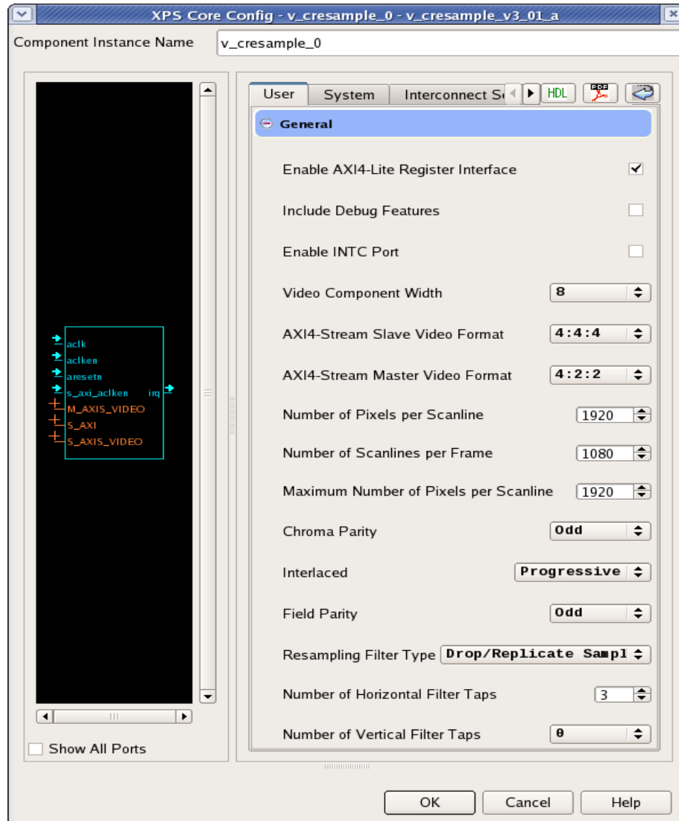
Figure 8-2: EDK pCore GUI
