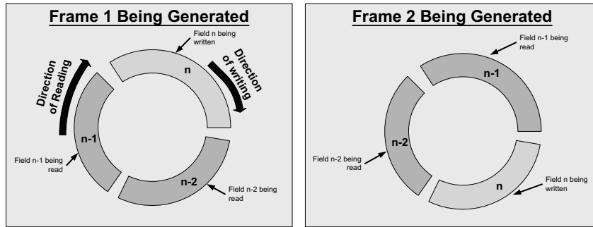
Figure 4-3: Triple Buffer Usage
