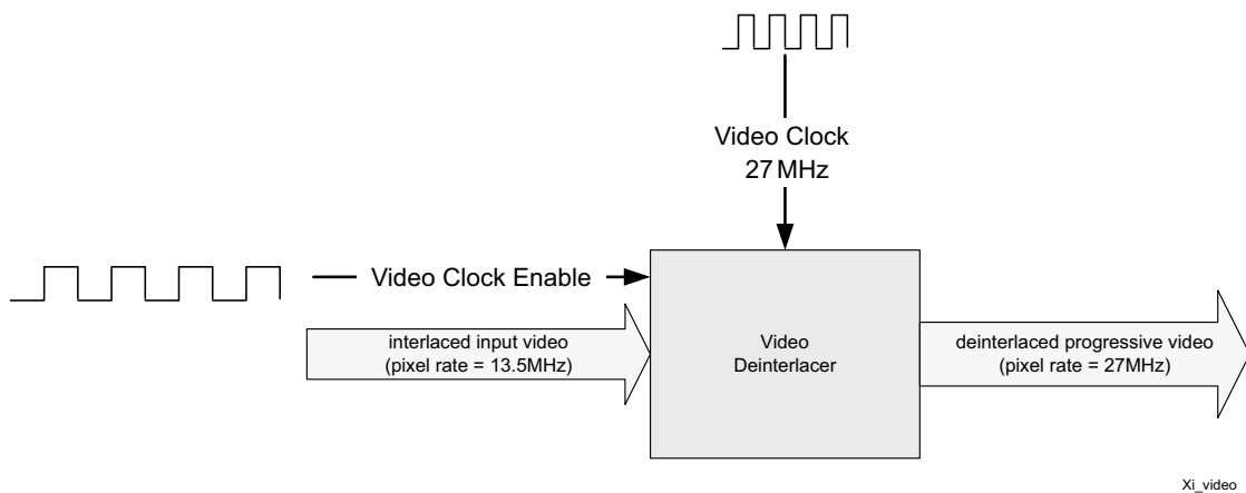
Figure 4-9: Input to Output Video Clock Ratio for SD
