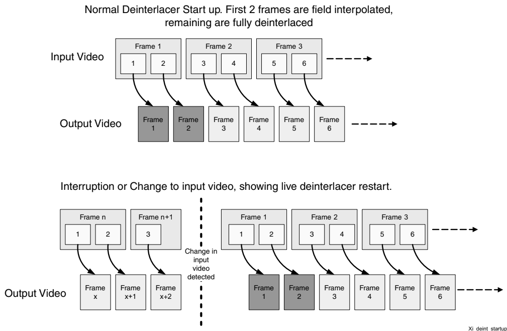
Figure 4-2: Examples of Deinterlacer Start-up Conditions
