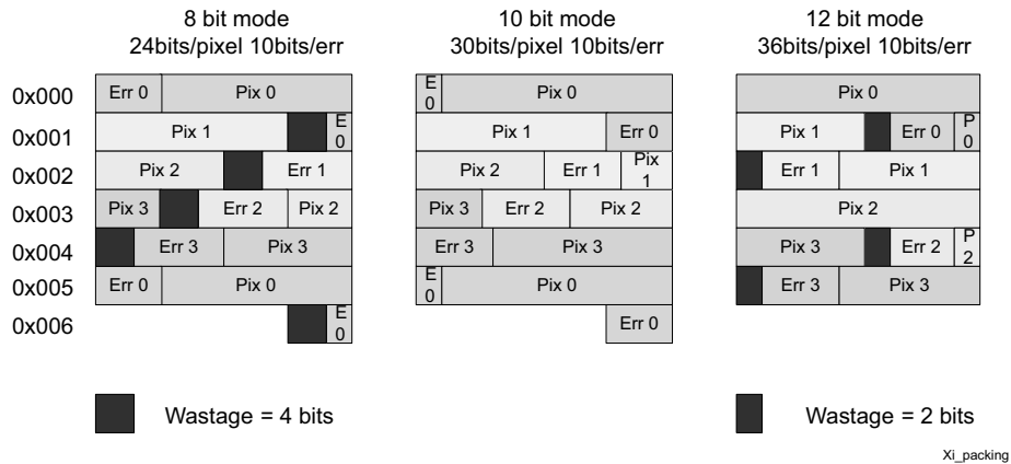
Figure 4-4: AXI4-MM Data Packing Format
