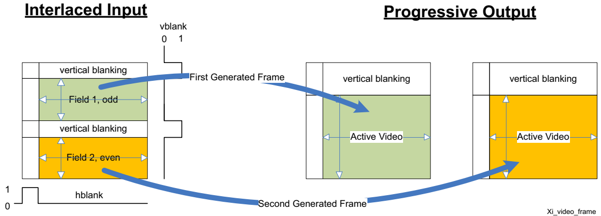
Figure 4-10: Input and Output Video Timing Formats
