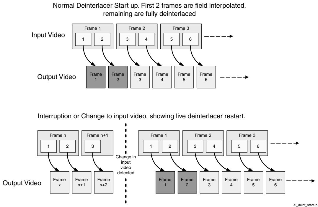
Figure 4-12: Examples of Deinterlacer Start-up Conditions
