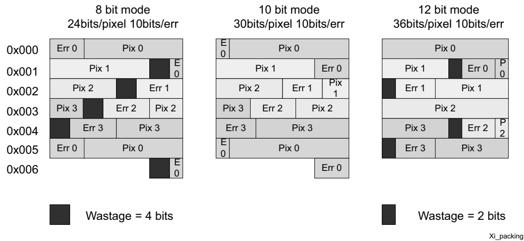
Figure 4-6: AXI4-MM Data Packing Format
