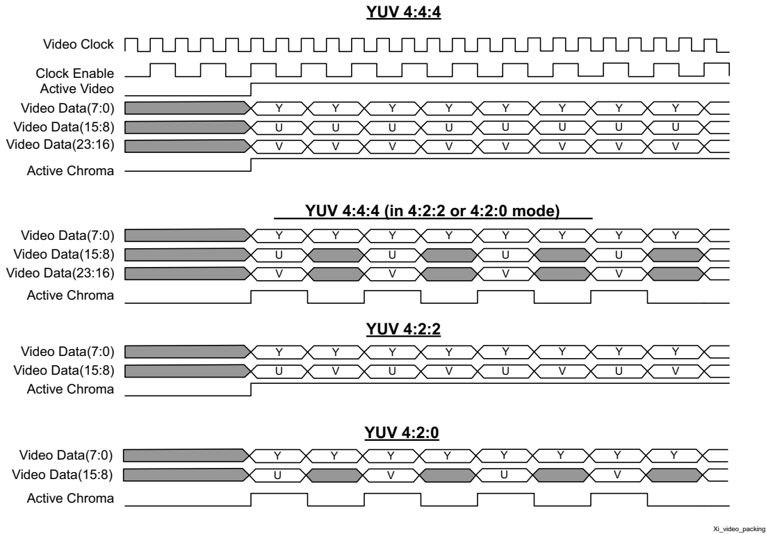
Figure 4-11: XSVI Input and Output Packing Formats
