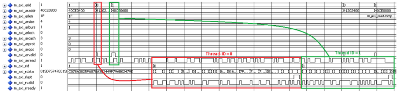
Figure 4-8: Read Stream Burst
