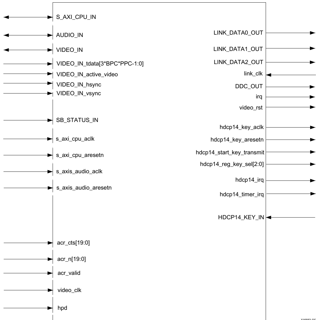
Figure 2-12: HDMI TX Subsystem Pinout – Native Video Interface (HDCP 1.4 Only)
