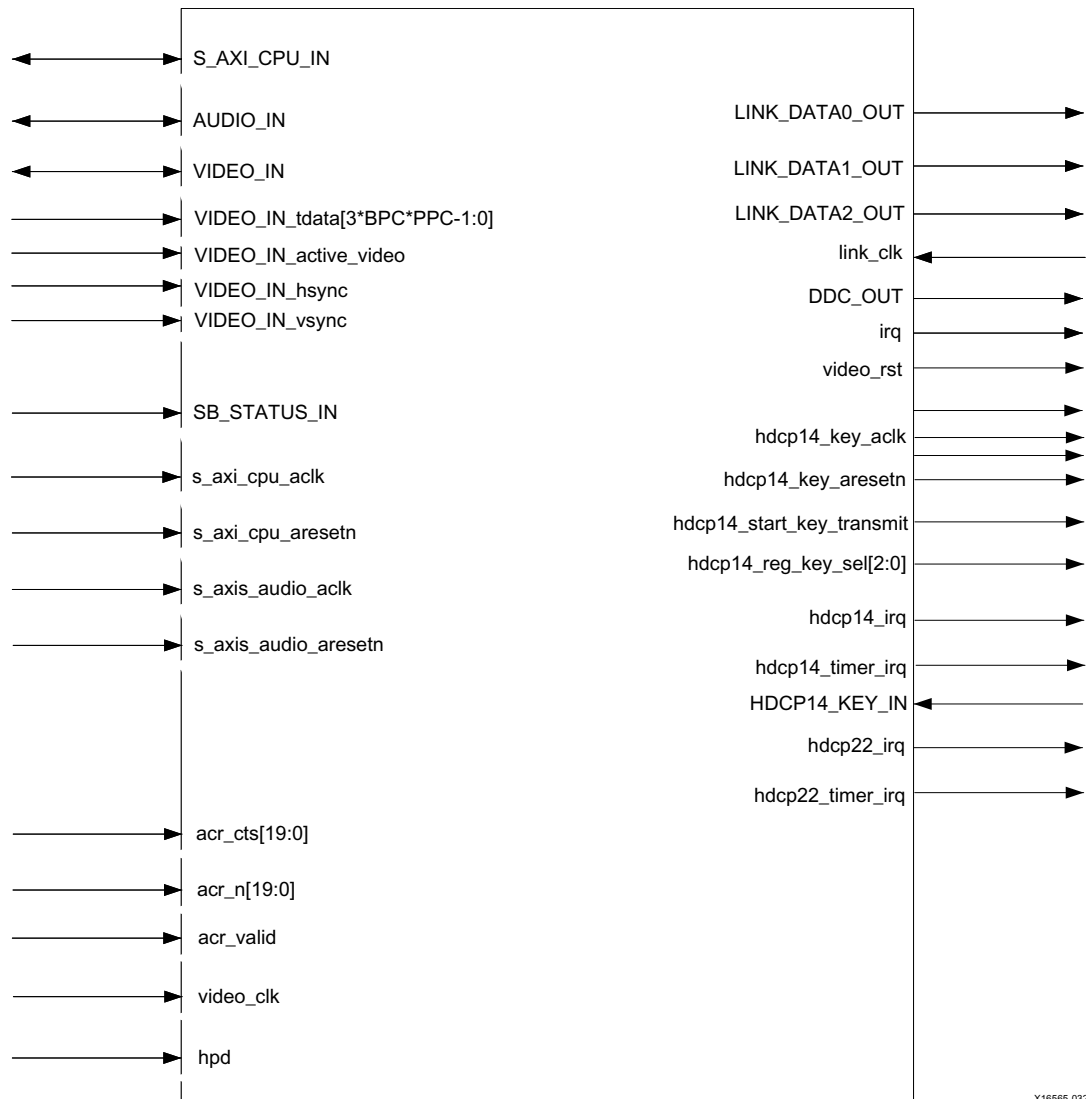
Figure 2-14: HDMI TX Subsystem Pinout – Native Video Interface (HDCP 1.4 and HDCP 2.2)
