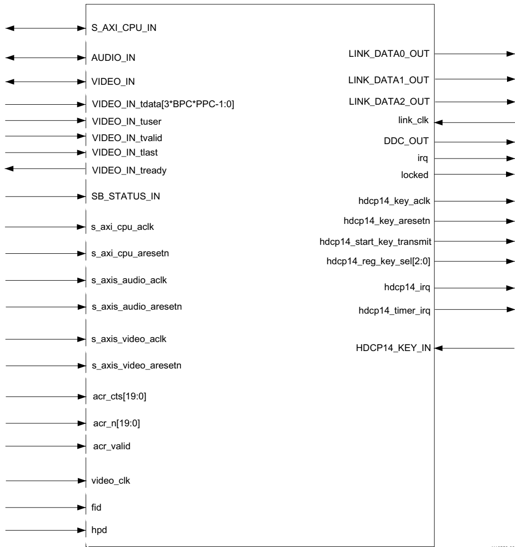
Figure 2-8: HDMI TX Subsystem Pinout – AXI4-Stream Video Interface (HDCP 1.4 Only)
