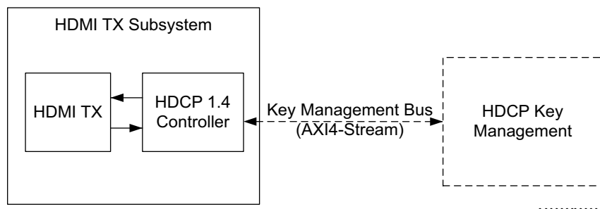
Figure 2-15: HDCP 1.4 Key Management Bus (AXI4-Stream)
