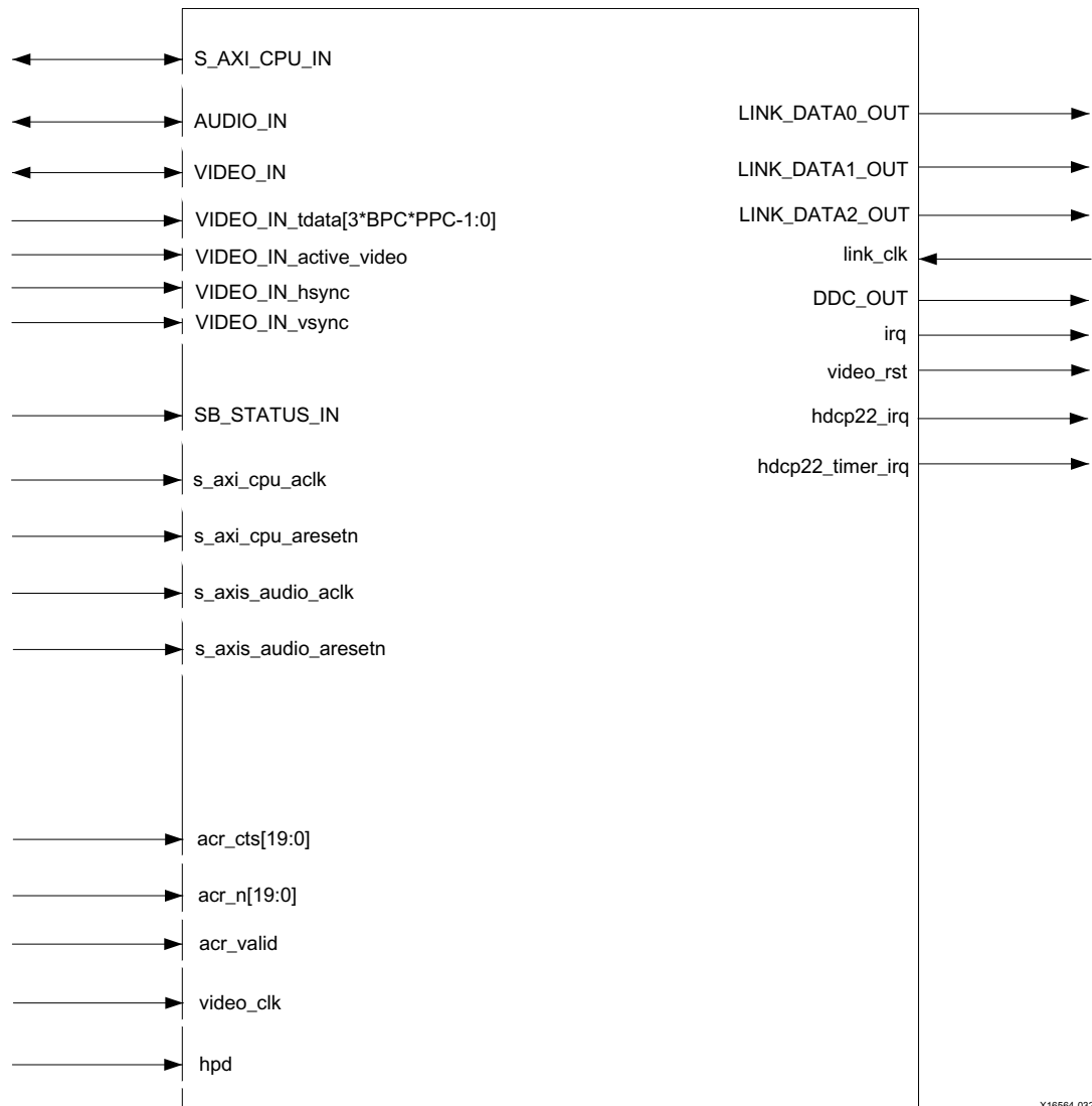
Figure 2-13: HDMI TX Subsystem Pinout – Native Video Interface (HDCP 2.2 Only)
