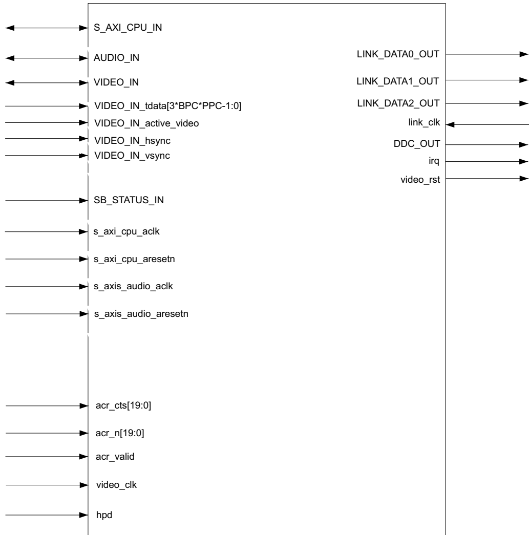
Figure 2-11: HDMI TX Subsystem Pinout – Native Video Interface (No HDCP)
