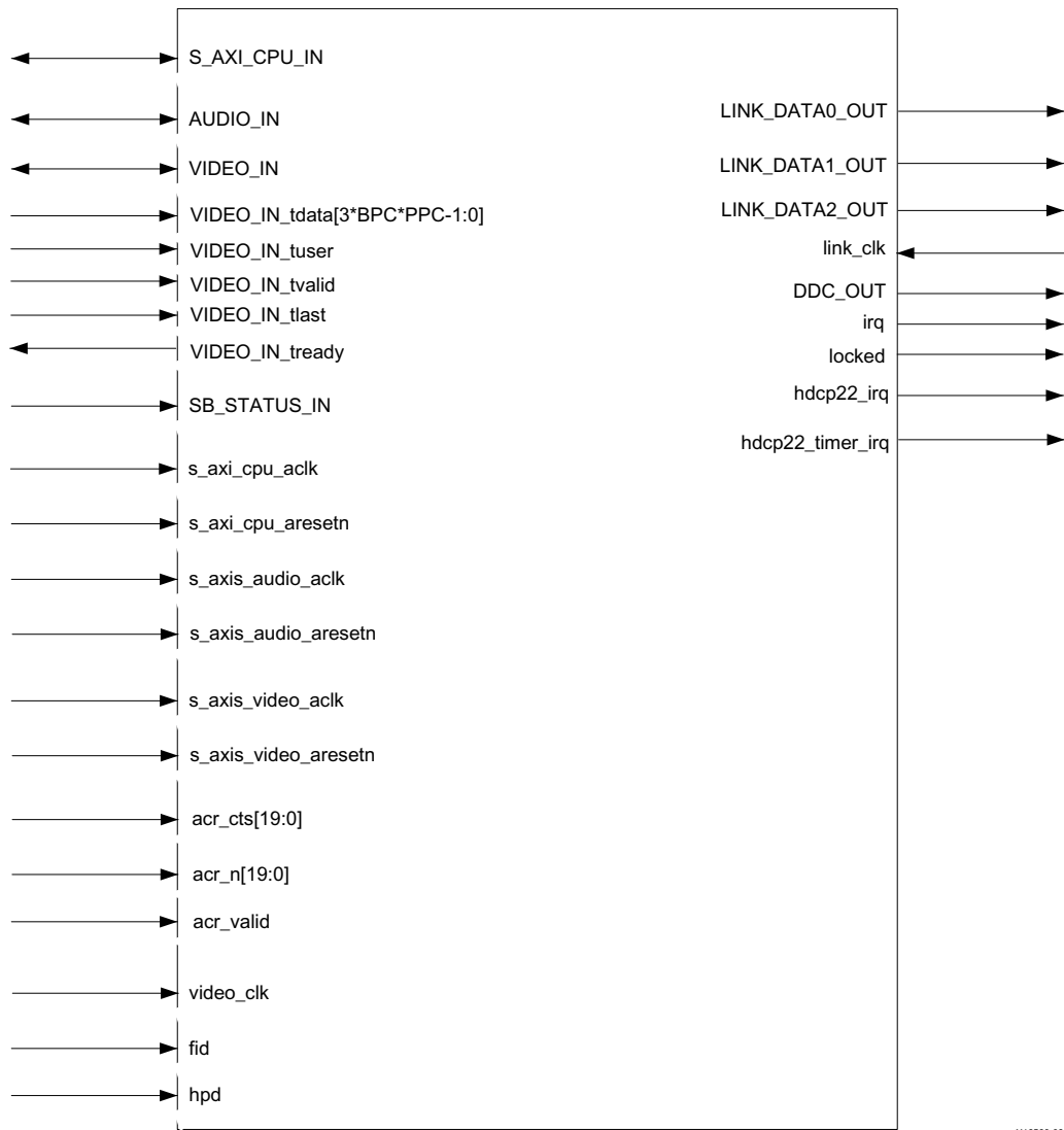
Figure 2-9: HDMI TX Subsystem Pinout – AXI4-Stream Video Interface (HDCP 2.2 Only)
