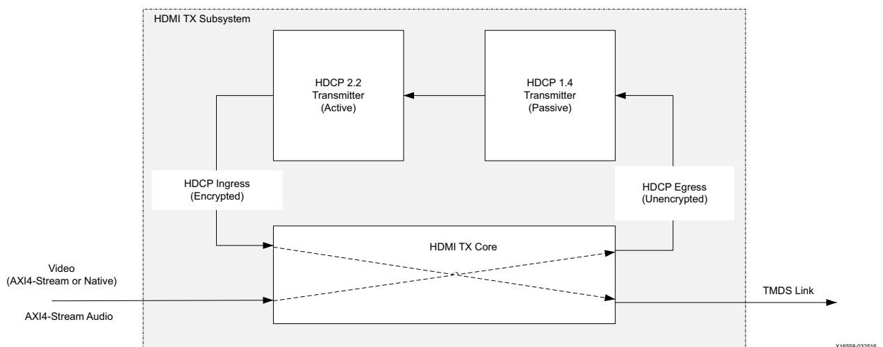
Figure 2-6: HDCP 1.4 and HDCP 2.2 over HDMI Transmitter
