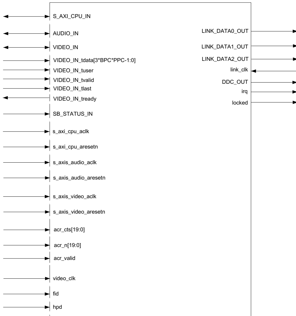
Figure 2-7: HDMI TX Subsystem Pinout – AXI4-Stream Video Interface (No HDCP)
