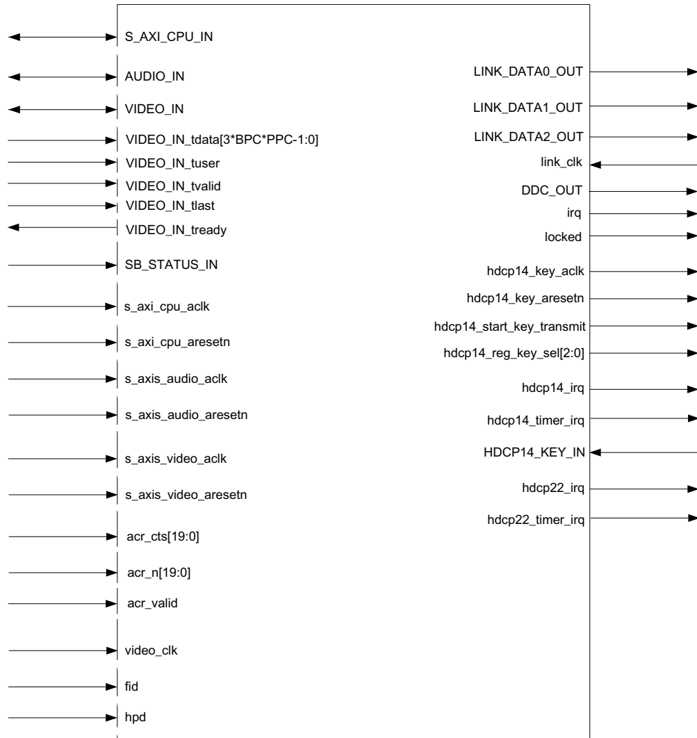
Figure 2-10: HDMI TX Subsystem Pinout – AXI4-Stream Video Interface (HDCP 1.4 and HDCP 2.2)
