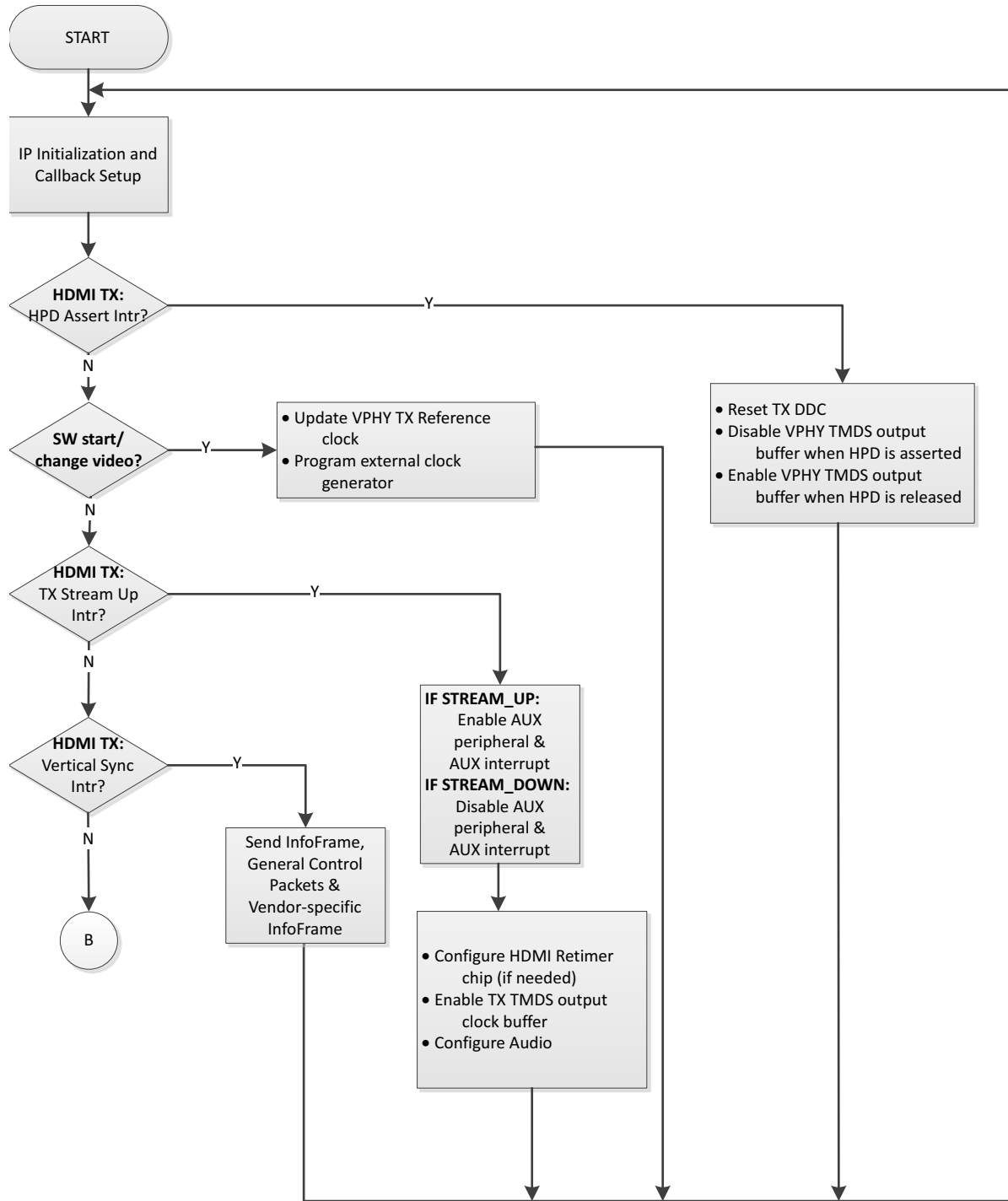
Figure C-3: TX Flow
