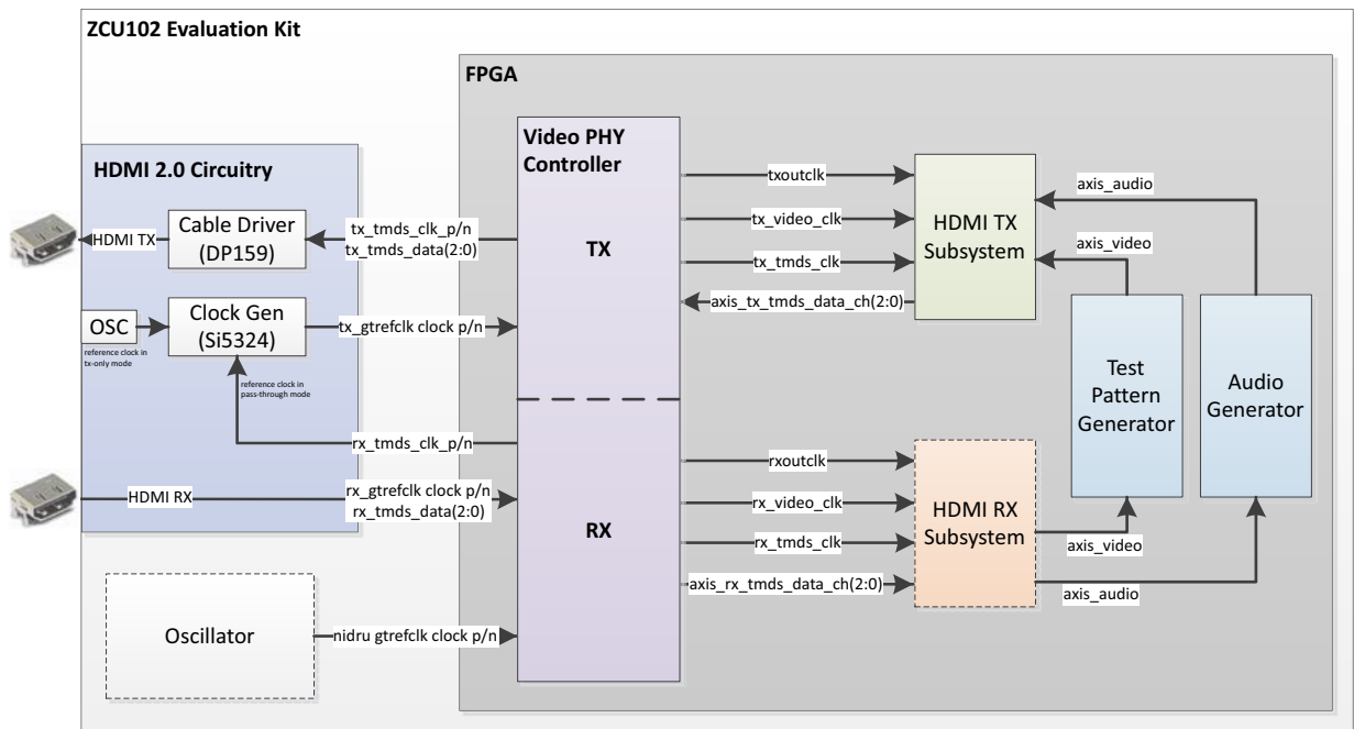
Figure 5-4: ZCU102/106 HDMI Reference Design Clock and Datapath Diagram
