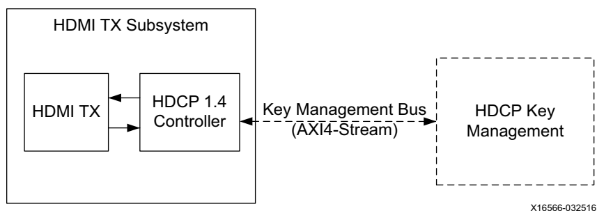
Figure 2-19: HDCP 1.4 Key Management Bus (AXI4-Stream)
