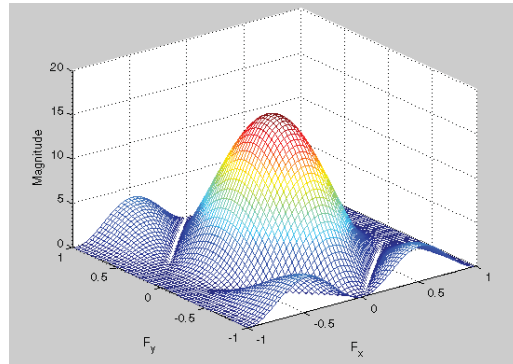
Figure 3-4: Coefficients and Frequency Response for Filter Strength 4
