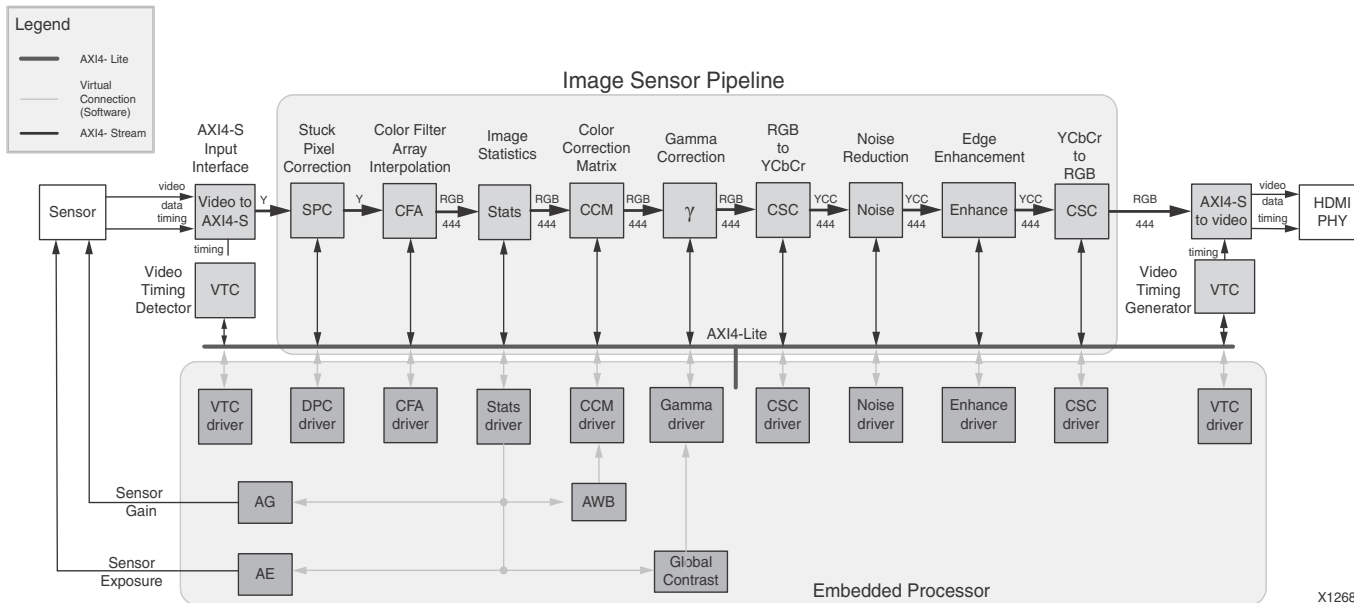
Figure 3-5: Image Sensor Pipeline System with Image Noise Reduction Core
