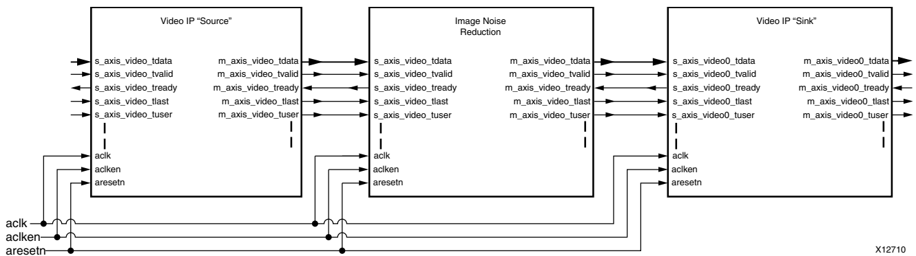
Figure 3-6: Example of ACLK Routing in an ISP Processing Pipeline
