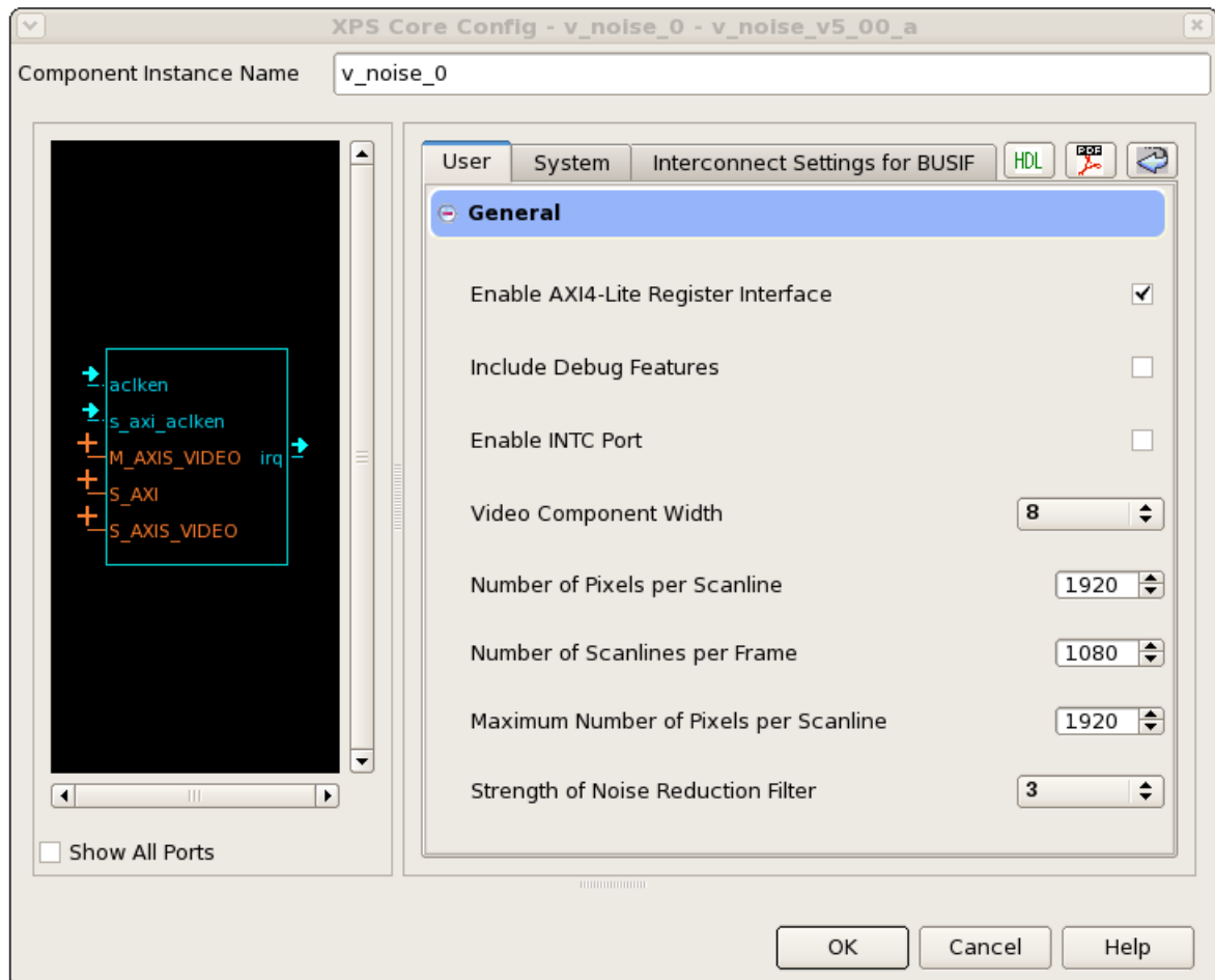
Figure 8-2: EDK GUI Screen
