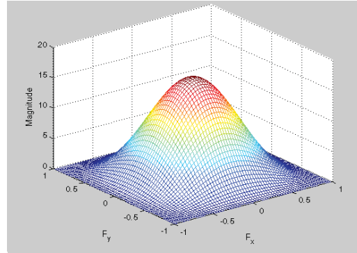
Figure 3-2: Coefficients and Frequency Response for Filter Strength 2
