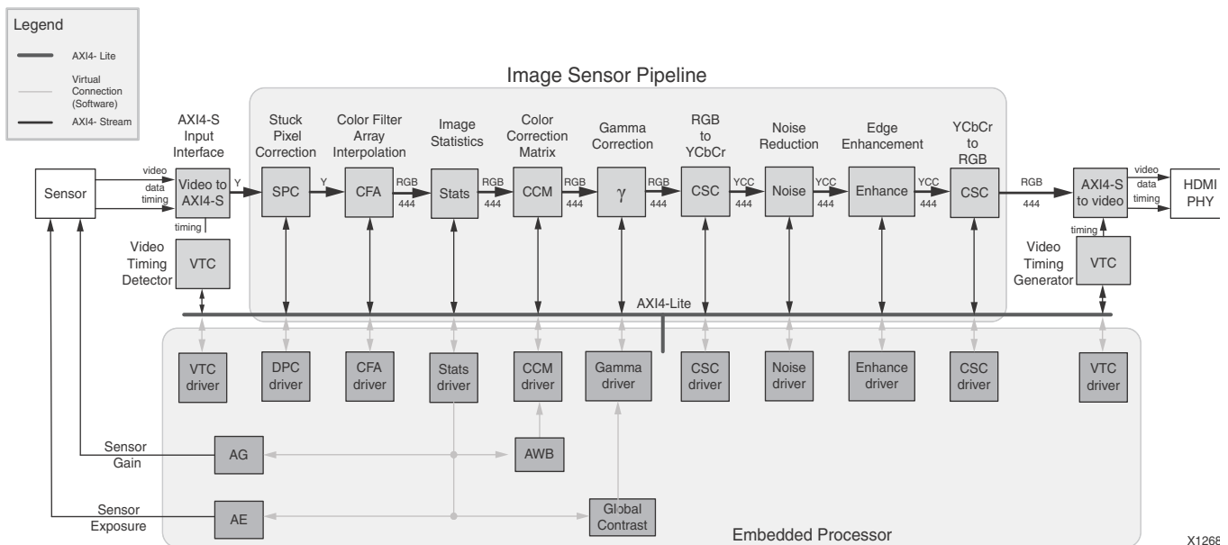
Figure 3-9: Image Sensor Pipeline System with Image Noise Reduction Core
