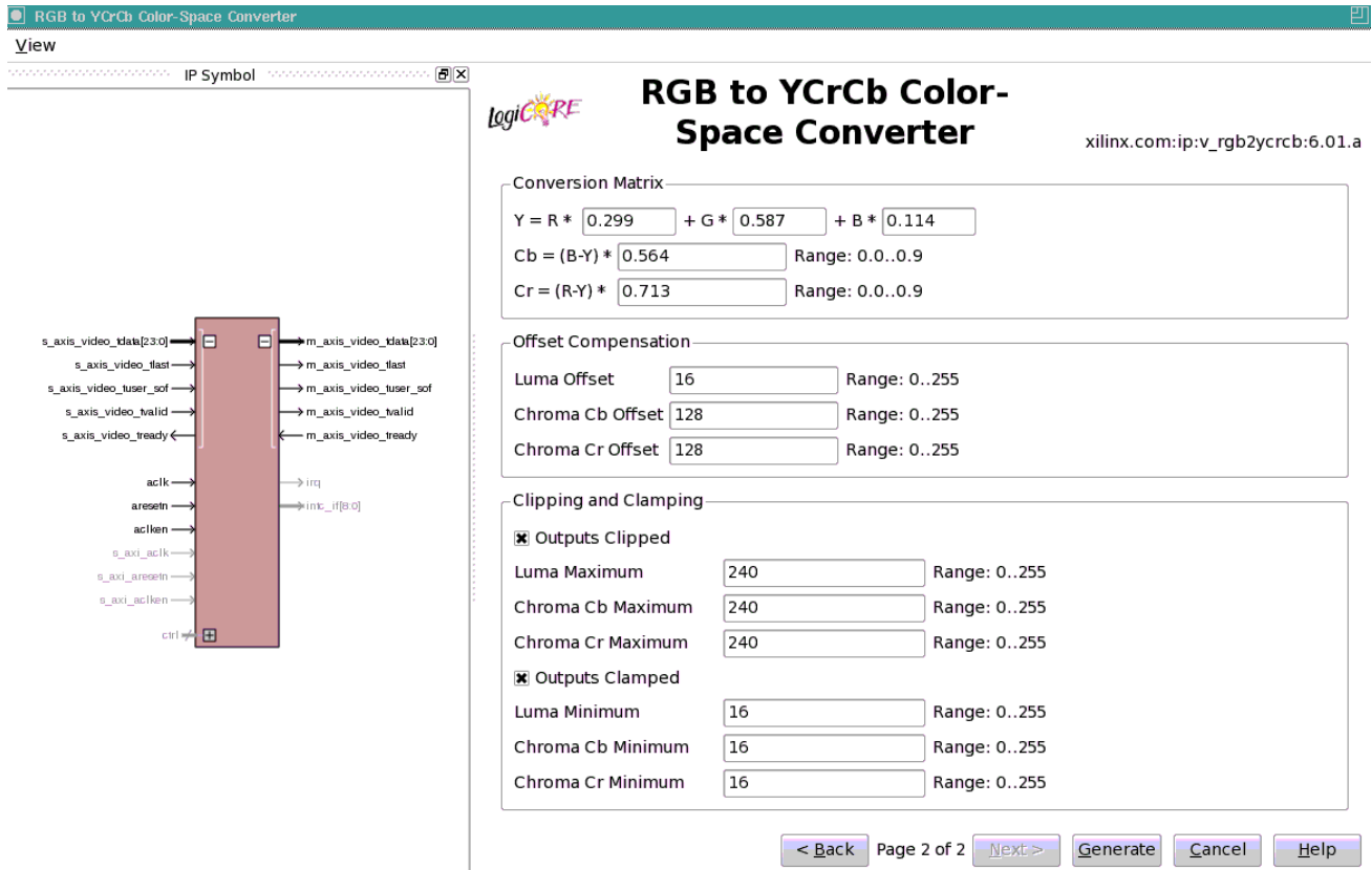
Figure 8-2: Conversion Matrix, Offset Compensation, Clipping and Clamping Screen
