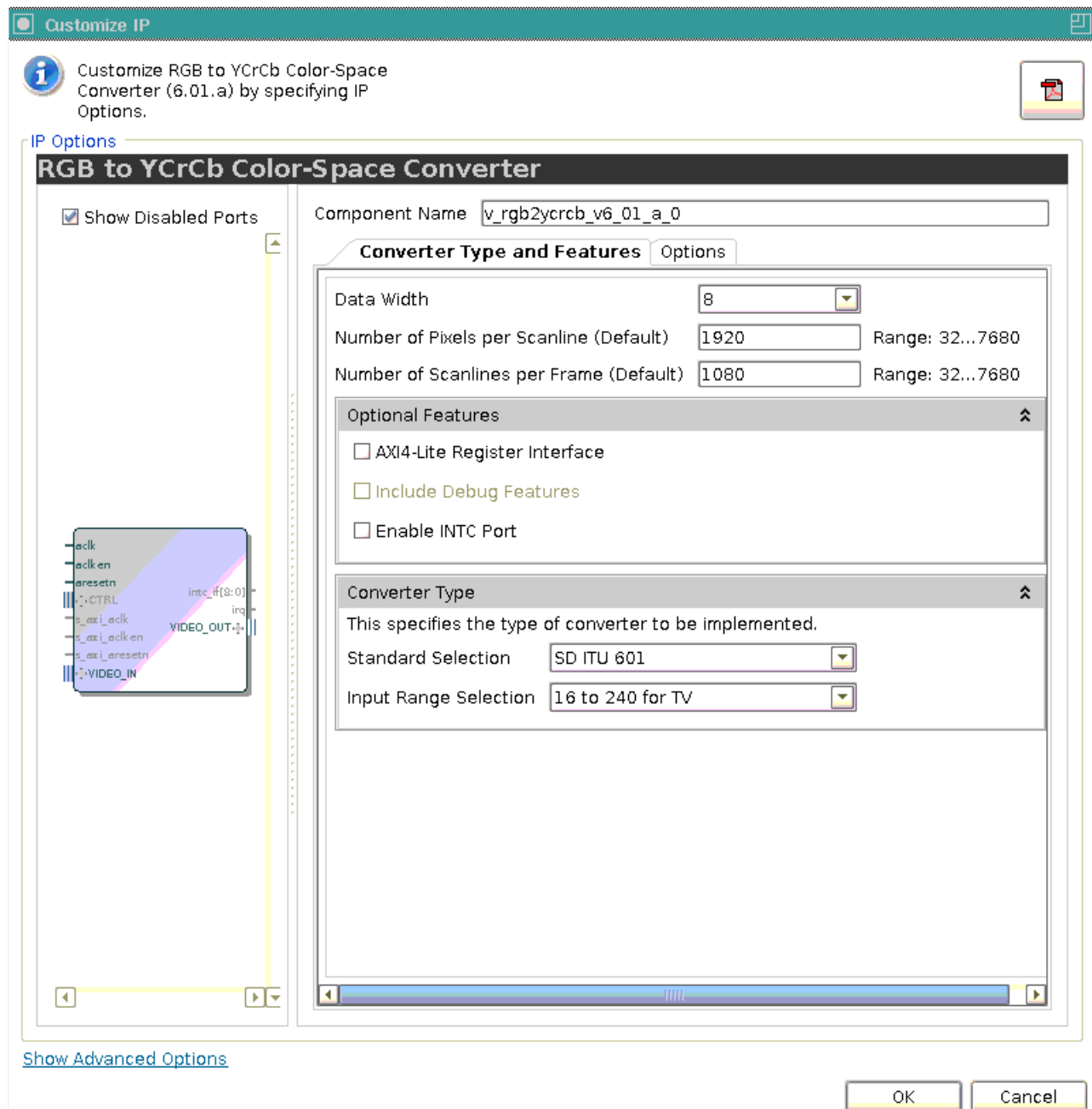
Figure 5-1: Color-Space Converter Main Screen
