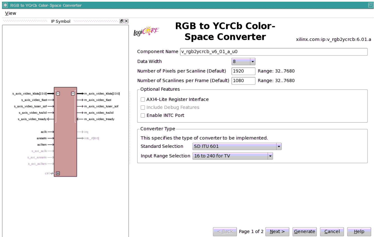
Figure 8-1: Color-Space Converter Main Screen
