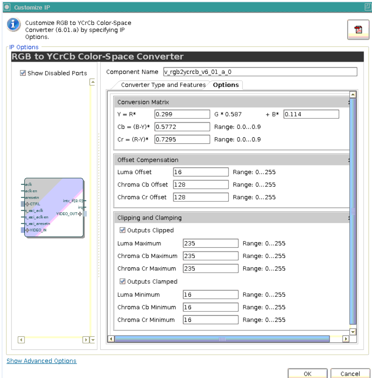
Figure 5-2: Conversion Matrix, Offset Compensation, Clipping and Clamping Screen
